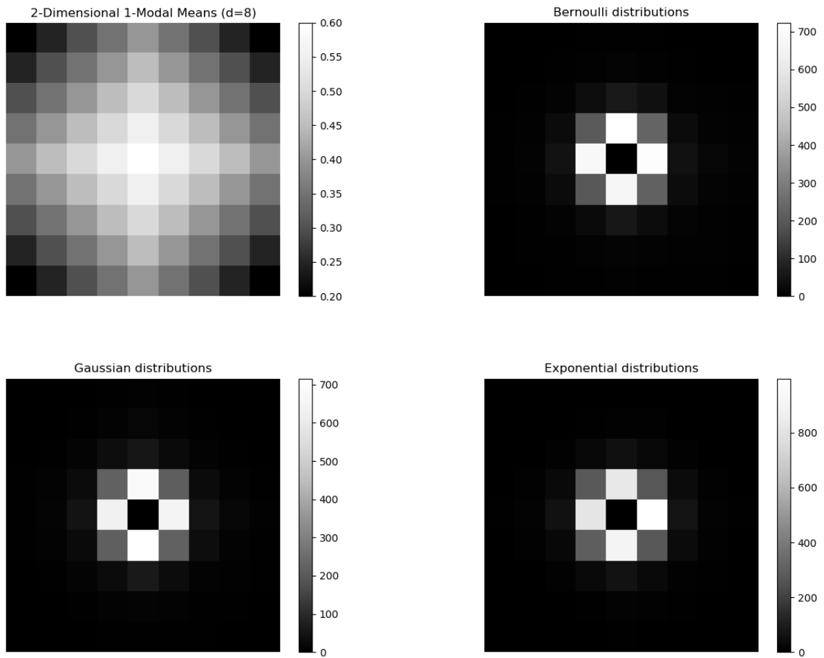
Figure 3.4: Number of pulls of sub-optimal arms under IMED-MB used in the unimodal case of Figure 3.2.
