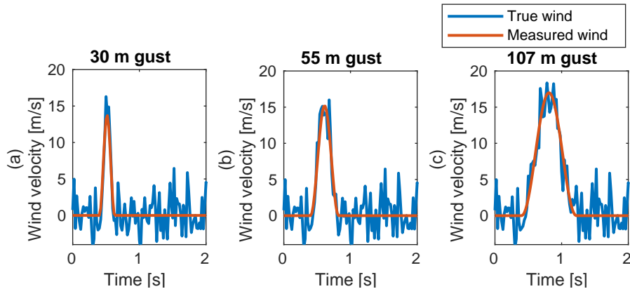
Figure 4.9: Wind velocity with and without lidar measurement noise
