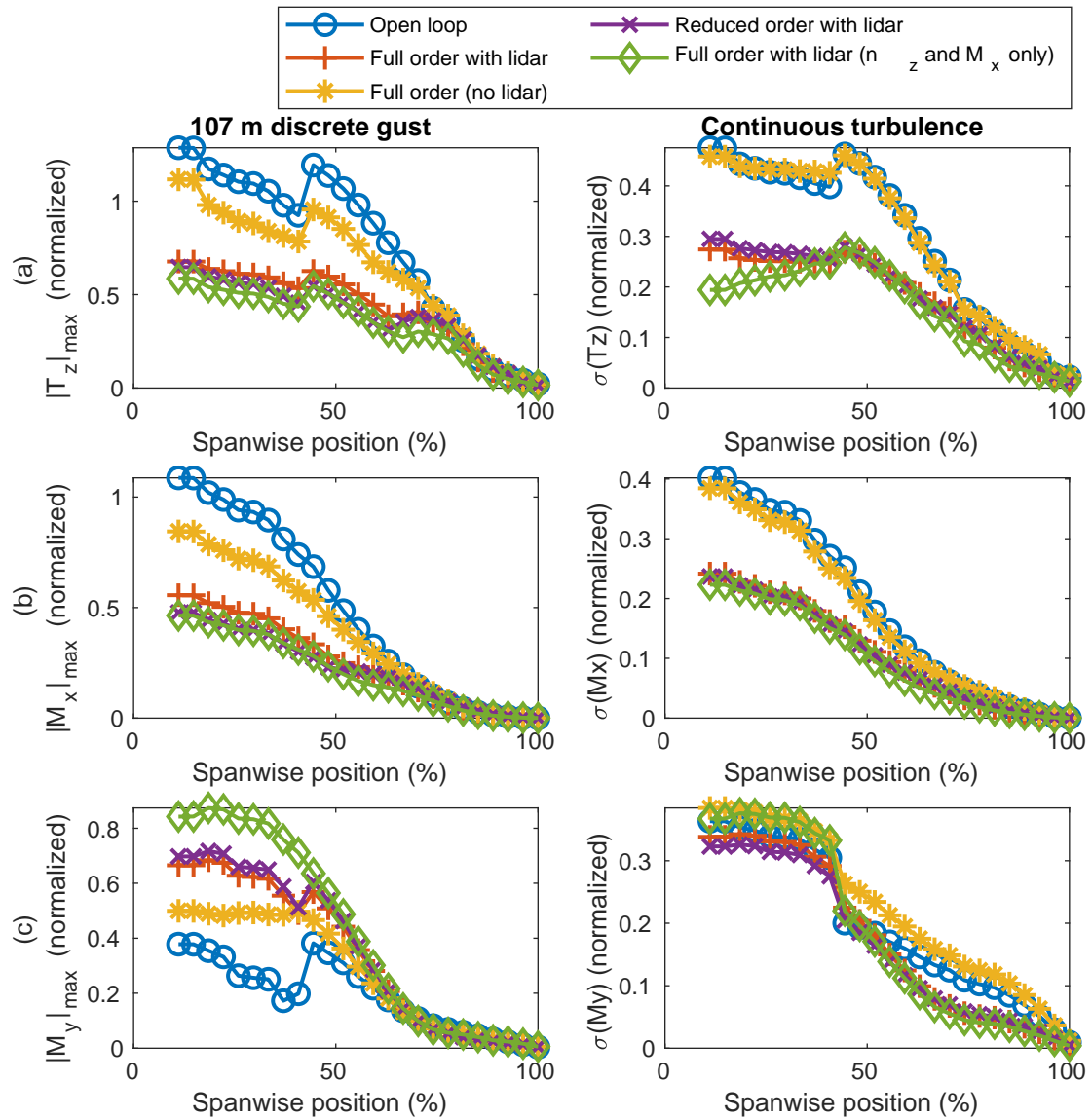
Figure 4.16: Maximum loads at several positions of the wing, with different controllers
