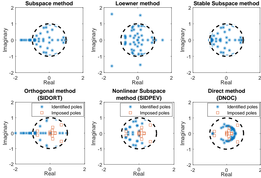
Figure 3.8: Poles of the identified models obtained by different techniques and imposed poles when applicable
