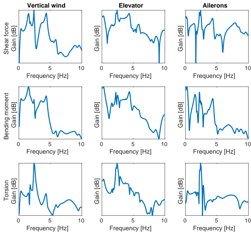
Figure 2.16: Transfer functions of the XRF1-HARW with loads outputs computed at the wing root
