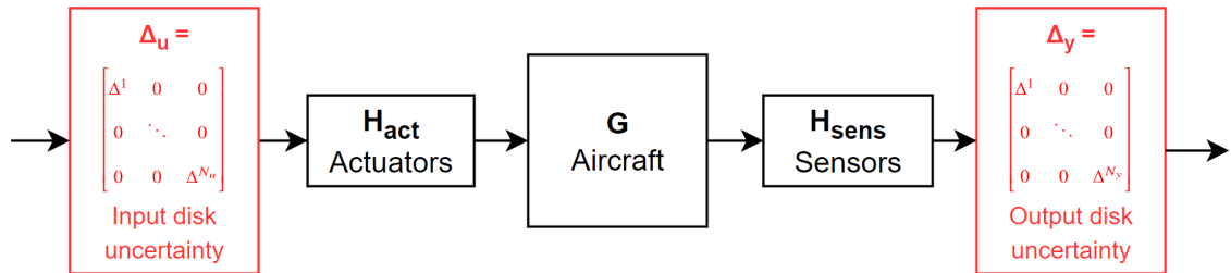
Figure 4.8: Uncertain aeroelastic model with disk uncertainties
