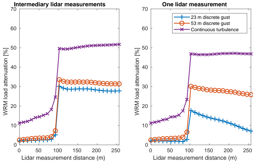
Figure 4.17: Load attenuation of the wing root bending moment with GLA controllers using lidars of varying sensing distance using intermediate measurements (left) or only one measurement (right)
