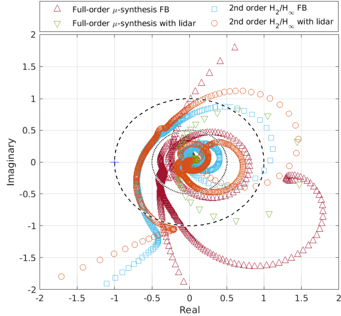
Figure E.2: MIMO nyquist diagrams of different robust GLA controllers
