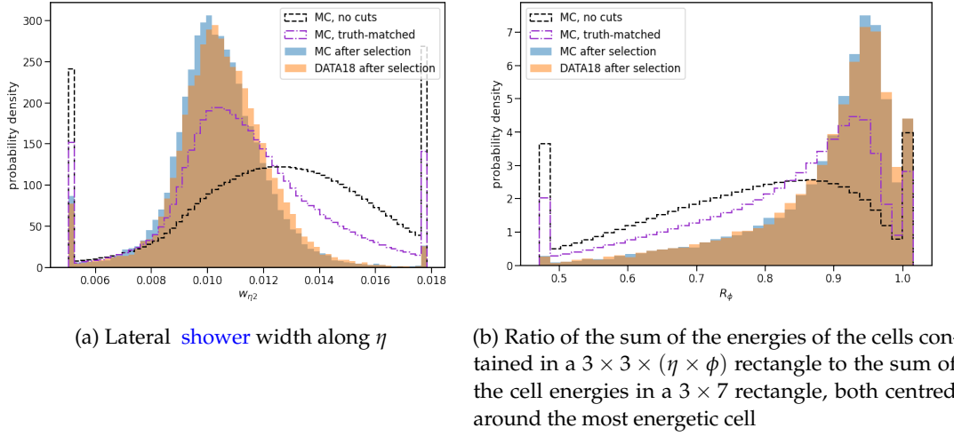
Figure 4.5.: Normalized distributions of w_{\eta^2} (a) and R_\phi (b), electron identification variables related to the second layer of the Electromagnetic (EM) calorimeter. Electron samples have been obtained by applying the selection model to EGAM1 derivations of Monte Carlo (blue) and DATA18 (orange). The reference distributions are presented for all probes before the selection (black) and probes truth-matched to b -quarks (Purple) for MC events only.
