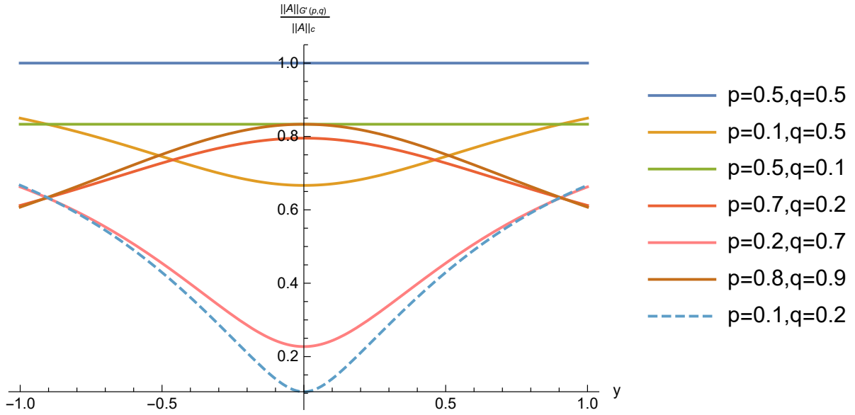
Figure 9.9: The ratio \|A\|_{G'(p,q)} / \|A\|_c for y \in [-1, 1] and different value of p and q .
