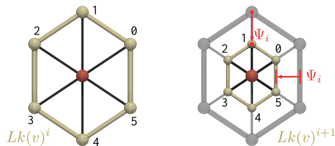
Figure 3.6 – Link topological invariance of edge-nested triangulations. From one hierarchy level ( i ) to the next ( i + 1 ), edge-nested triangulations preserve the local structure of the link Lk(v)^i of an old vertex v (red sphere). In particular, there exists a one-to-one mapping \Psi_i between the vertices and the edges (red arrows) of Lk(v)^i and Lk(v)^{i+1} .
