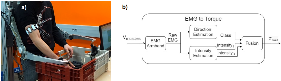
Figure 1.23: Upper-limb BHV2 exoskeleton used for the doctoral project. This exoskeleton is under-actuated and reversible. Each limb is composed of two segments and (upper arm and forearm) and four joints: two passive joints and two interrelated joints actuated with the same motor. The user is interacting with the exoskeleton at hand level with a hand strap, thus only providing upward pull force assistance (a). Approach for detecting user’s intention based on direction estimation (through neural network) and intensity estimation ( \text{Intensity}_B and \text{Intensity}_T correspond to the intensity of the Biceps activation and Triceps activation, respectively) (b) (from Treussart, Geffard, et al., 2019)
