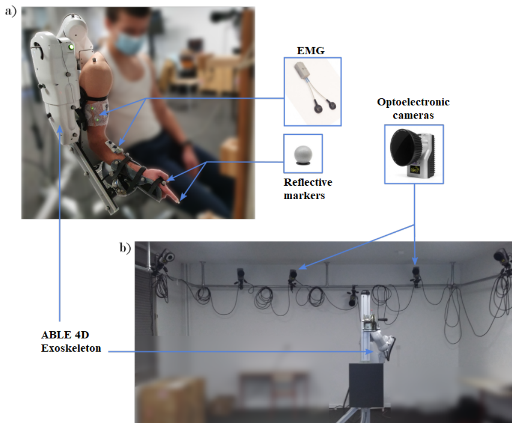
Figure 1.21: Platform for HEI analysis into the CIAMS laboratory composed of an optoelectronic system (Qualisys, Göteborg, Sweden), and EMG sensors (from S. Bastide, 2021).
