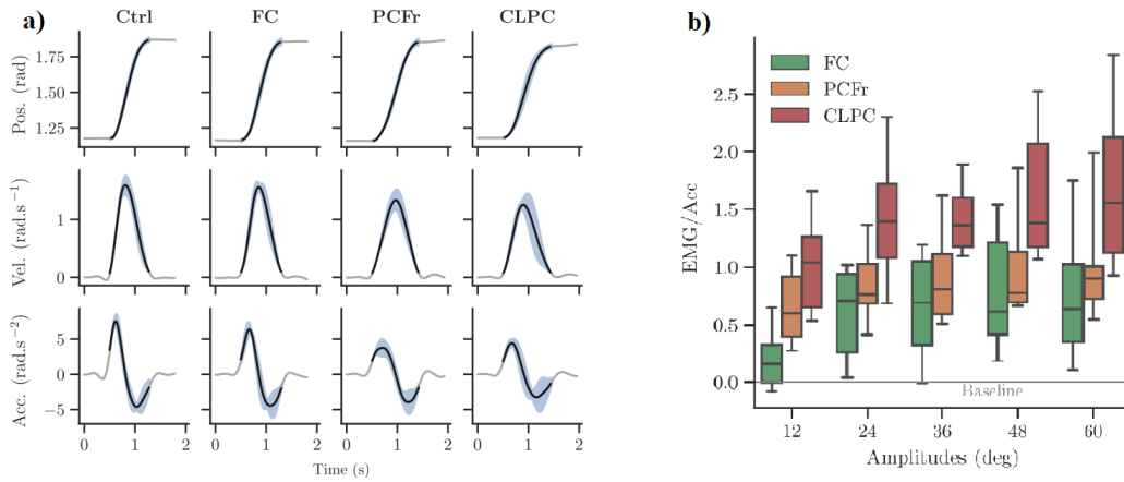
Figure 1.22: Representative trajectories of position, velocity and acceleration across time for one participant (a), and mean agonist muscle transparency index for upward movements (from S. Bastide, 2021; Verdel, Bastide, Vignais, et al., 2021). Ctrl: Control condition without wearing the exoskeleton. FC: Full compensation based on identification. PCFr: Partial Compensation based on identification without Friction compensation. CLPC: Closed-loop position control.
