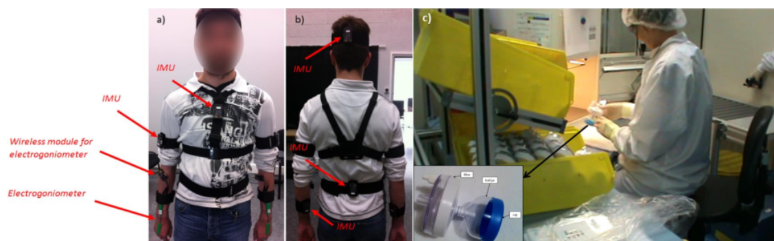
Figure 1.10: Placement of IMUs, electrogoniometers and their wireless modules in the front (a) and back views (b). Workstation dedicated to filter cleaning and description of the filter (c) (from Vignais, Bernard, et al., 2017).
