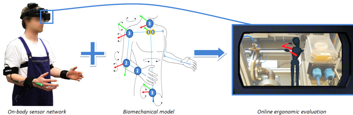
Figure 1.12: On-body sensor network composed of IMUs coupled with goniometers (left) and underlying biomechanical model of the upper body (middle) with rotation axes for local body frames, and degrees of freedom of each joint, allowing a real-time ergonomic feedback into the HMD (right) (from Vignais, Miezal, et al., 2013).
