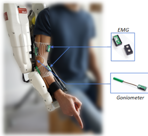
Figure 1.18: ABLExoskeleton (1 st version) for HEI analysis with goniometer and EMG sensors (Biometrics Ltd, Newport, UK) (from S. Bastide, 2021).
