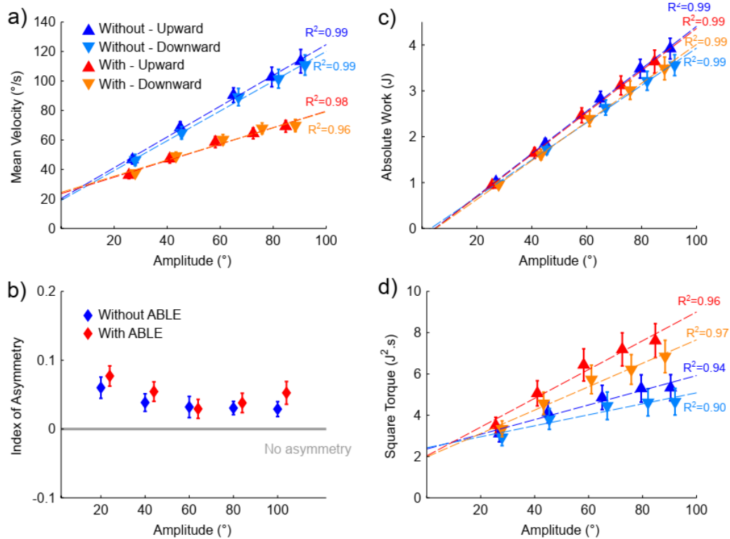
Figure 1.20: Angular velocity (a), index of asymmetry (b), absolute work (c) and square torque (d) depicted as a function of movement amplitudes averaged for all participants ( \pm standard deviation). Dotted lines represent linear regressions with associated coefficients of determination (from Bastide et al., 2018).
