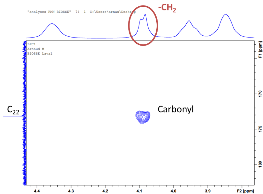
FIGURE 67: HMBC SPECTRUM
