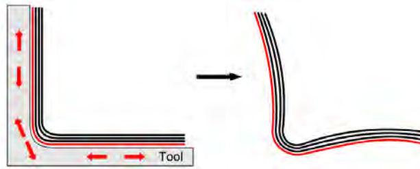
Figure 1.15: Effect of tool–part interaction on distortion of a part with curved sections [9].
