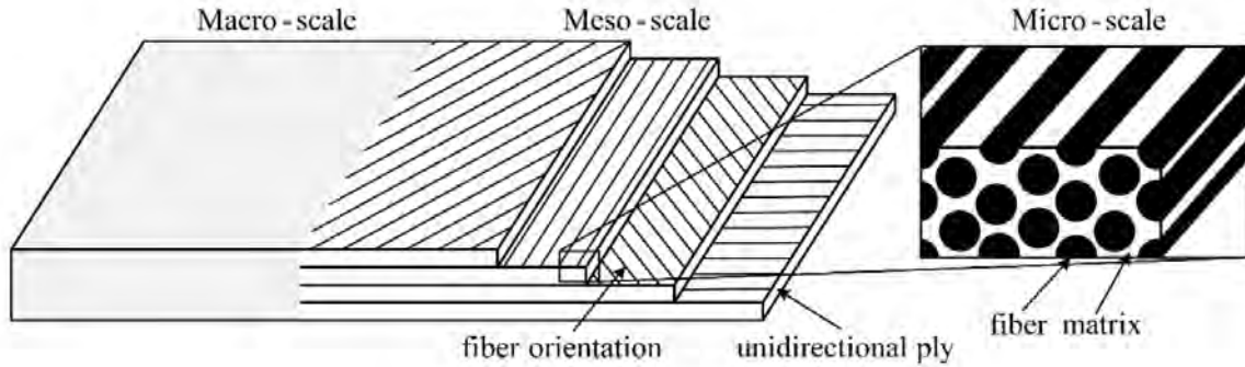
Figure 4.1: Different scales defined in a composite laminate structure [40].
