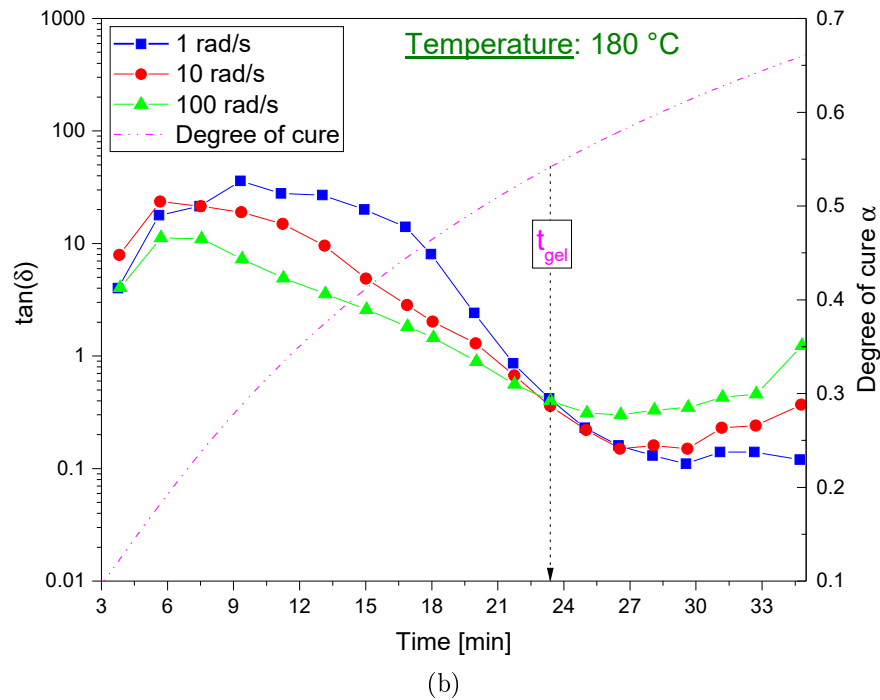
Figure 2.12: Loss factor \tan(\delta) as a function of time at three different frequencies during the isothermal curing of the M21 resin at (a) 160 °C and (b) 180 °C.
