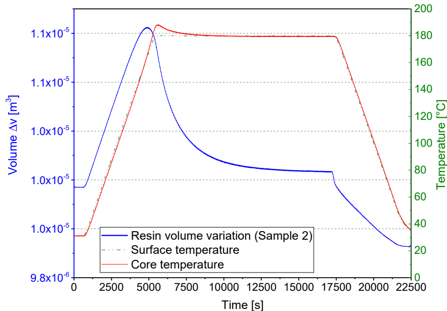
Figure 2.10: Typical dilatometric curve of volumetric behavior obtained with PvT- \alpha apparatus of the M21 resin during a curing cycle (Obtained results from sample (2) testing).
