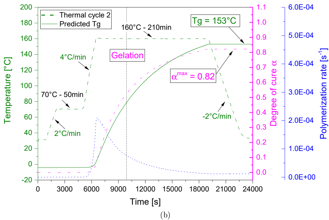
Figure 3.8: New proposed curing cycles: (a) named as cycle 1 and (b) named as cycle 2.
