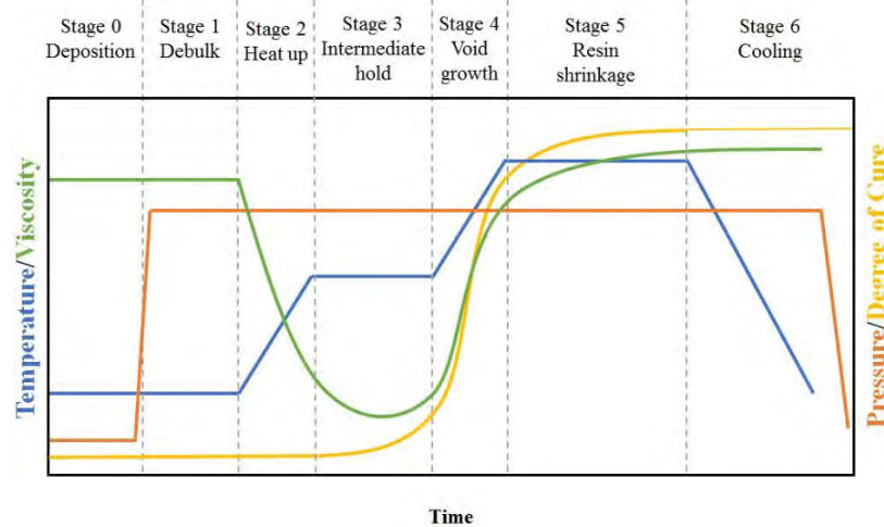
Figure 1.16: Schematic of different stages in a typical autoclave process cycle [11].
