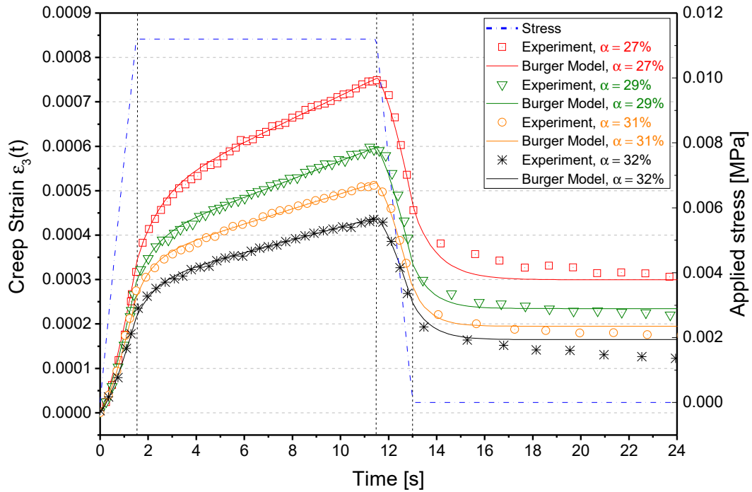
Figure 5.19: Comparison between creep-recovery experimental and fitted data predicted by Burgers model for an applied stress of 11 \cdot 10^{-3} MPa at different \alpha .
