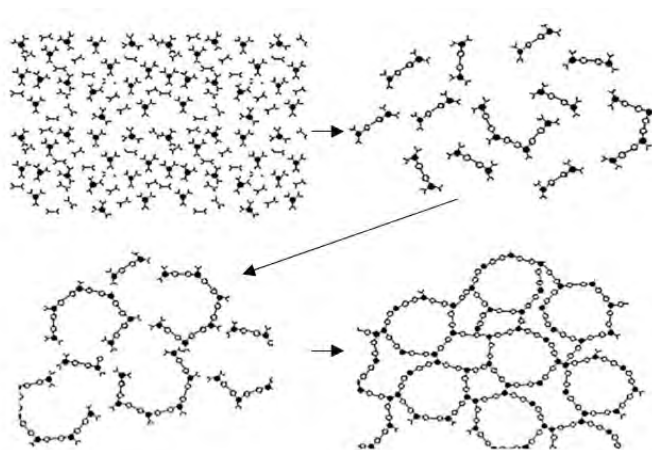
Figure 1.1: Thermoset resin polymerization mechanism from a monomer stage to a fully cured (3D) cross-linked network [2].
