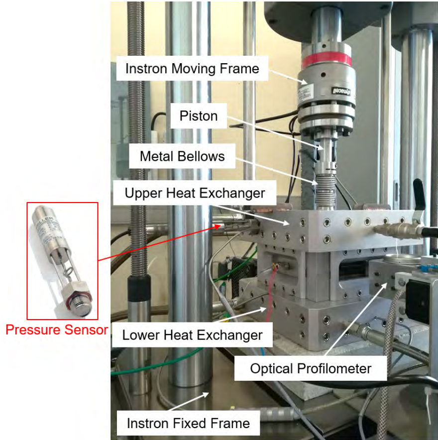
Figure 2.17: PvT-Haddoc device.
