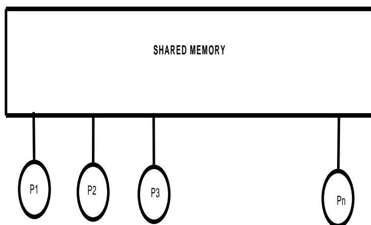
Figure 2.3: PRAM Model
