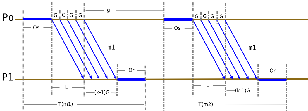
Figure 2.7: LogGP Basic Transfer
