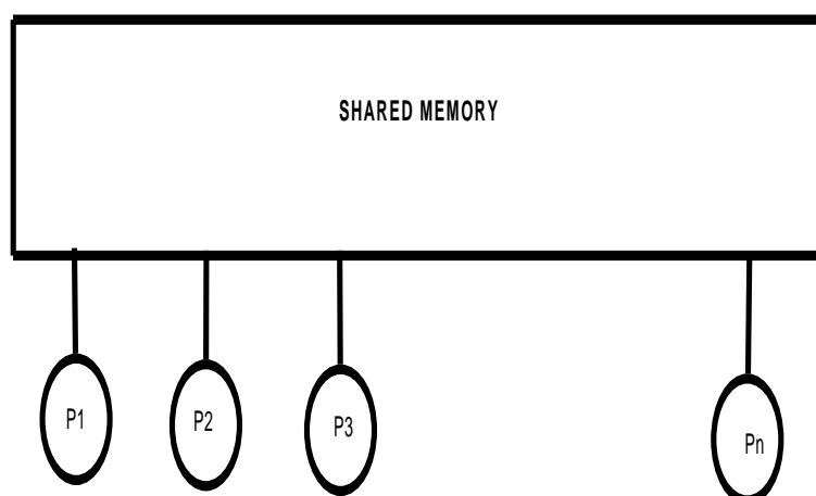
Figure 2.3: PRAM Model
