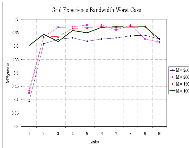
Figure 5.30: GDX-Grillon Transfer: Bandwidth Worst Case Measurement
