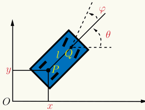
Figure 1.3: Car Model: the state vector is made of the coordinates (x, y) of the rear axle's center and of the angle \theta between the car's axis and the x -axis. The controls are the speed u and the angle \varphi between the wheels' axis and the car's axis. The length l is the distance between the two axles.
