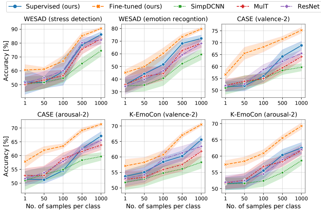
Figure 3.7: Performance comparison with state-of-the-art supervised learning-based methods on limited labeled data sampled from the three emotion recognition datasets. The horizontal axis of each subplot is the number of randomly selected samples from each class, varying from 1 to 1000, while the vertical axis is the corresponding average accuracy.
