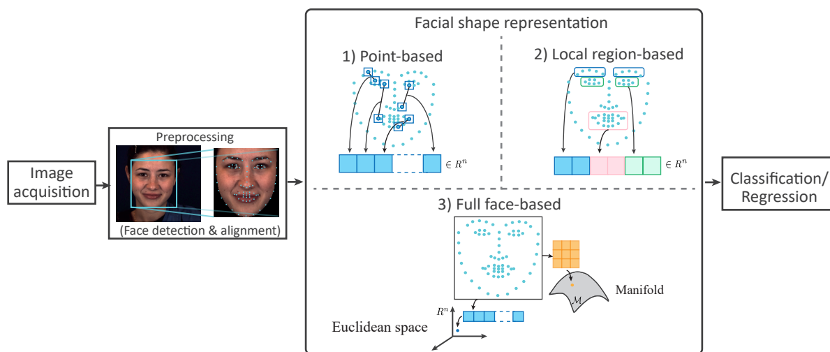
Figure 2.8: Landmark-based facial expression recognition pipeline.
