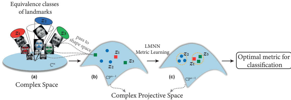
Figure 6.1: Overview of the proposed approach. (a) 2D landmarks detected in images of facial expressions are first converted to vectors in complex space; (b) The variants obtained by affine transformation constitute the equivalence class of landmarks, which can be considered as the same point in the complex projective space; (c) The application of metric learning enables the reduction of intra-class differences while enlarging inter-class distances. Finally, the learned metric is used for similarity-based classification.
