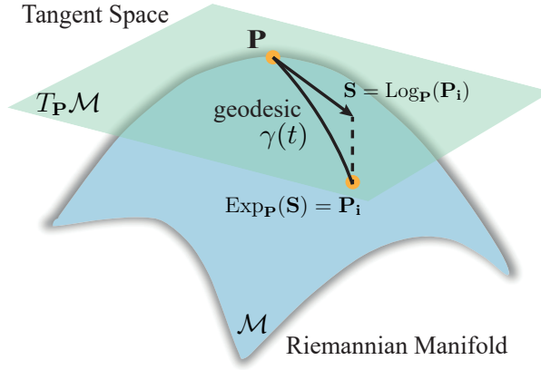
Figure 4.2: Exponential map and logarithm map between the Riemannian Manifold \mathcal{M} and the tangent space T_{\mathbf{P}}\mathcal{M} at \mathbf{P} .
