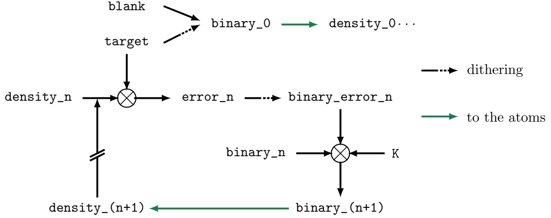
Figure 2.6: Diagram of the grey levels iterative loop. The first row represents the initialisation while the second row describes a loop. Dithering time steps are represented with half-dashed arrows and green arrows mean imprinting the image on the atoms via the DMD.
