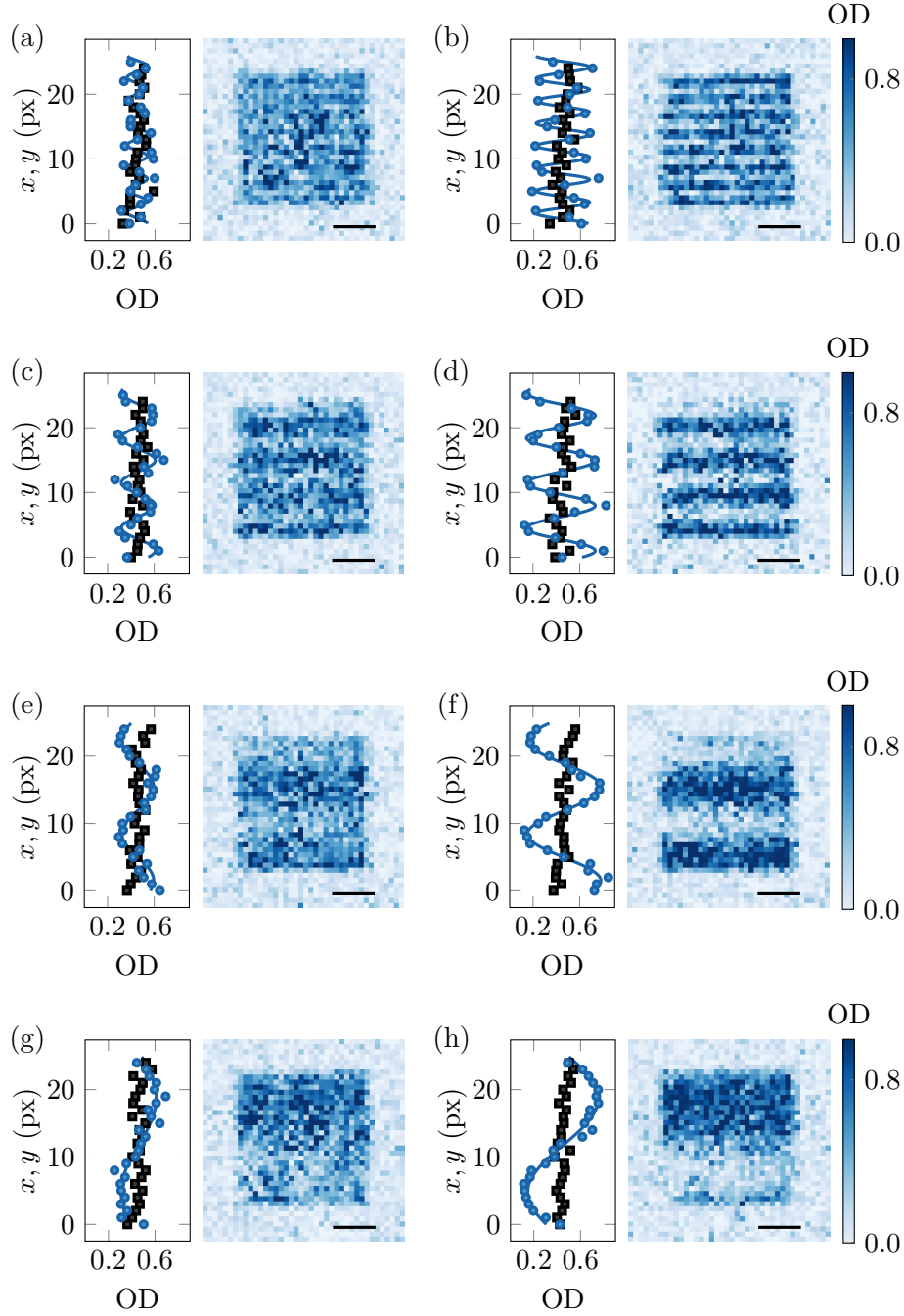
Figure 6.13: Images of the atomic cloud in a periodic potential of period \lambda = 4\mu\text{m} (a)-(b), \lambda = 8\mu\text{m} (c)-(d), \lambda = 16\mu\text{m} (e)-(f) and \lambda = 32\mu\text{m} (g)-(h) (scale bar: 10\mu\text{m} ). The average profiles in the direction x (black squares) and y (blue points) are shown on the left. The blue solid lines are fit to the data in the y -axis, using a sine function. The light intensity is doubled between the left and the right columns. Here, the in-plane confinement is a square box of side L = 32\mu\text{m} .
