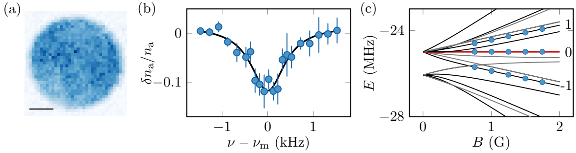
Figure 3.7: (a) Homogeneous atomic sample (bar length: 10\ \mu\text{m} ). (b) Typical microwave photoassociation signal. The atoms are initially prepared in |1,0\rangle and shined by a mw field of frequency \nu . The depletion, maximal at \nu = \nu_m , indicates the creation of dimers. The solid line is a fit to the data, using Eq. (3.28). (c) Energy diagram of the multiplicity \mathcal{B} showing the three lines measured from |f=1, m_f=0\rangle (blue points) and the fitted model (solid lines). The corresponding total angular momentum projection is indicated on the right. The red line indicates the magnetic-insensitive state |\Psi_0^{(n=-1)}\rangle and the grey lines are forbidden from |f=1, m_f=0\rangle by the electronic selection rules.
