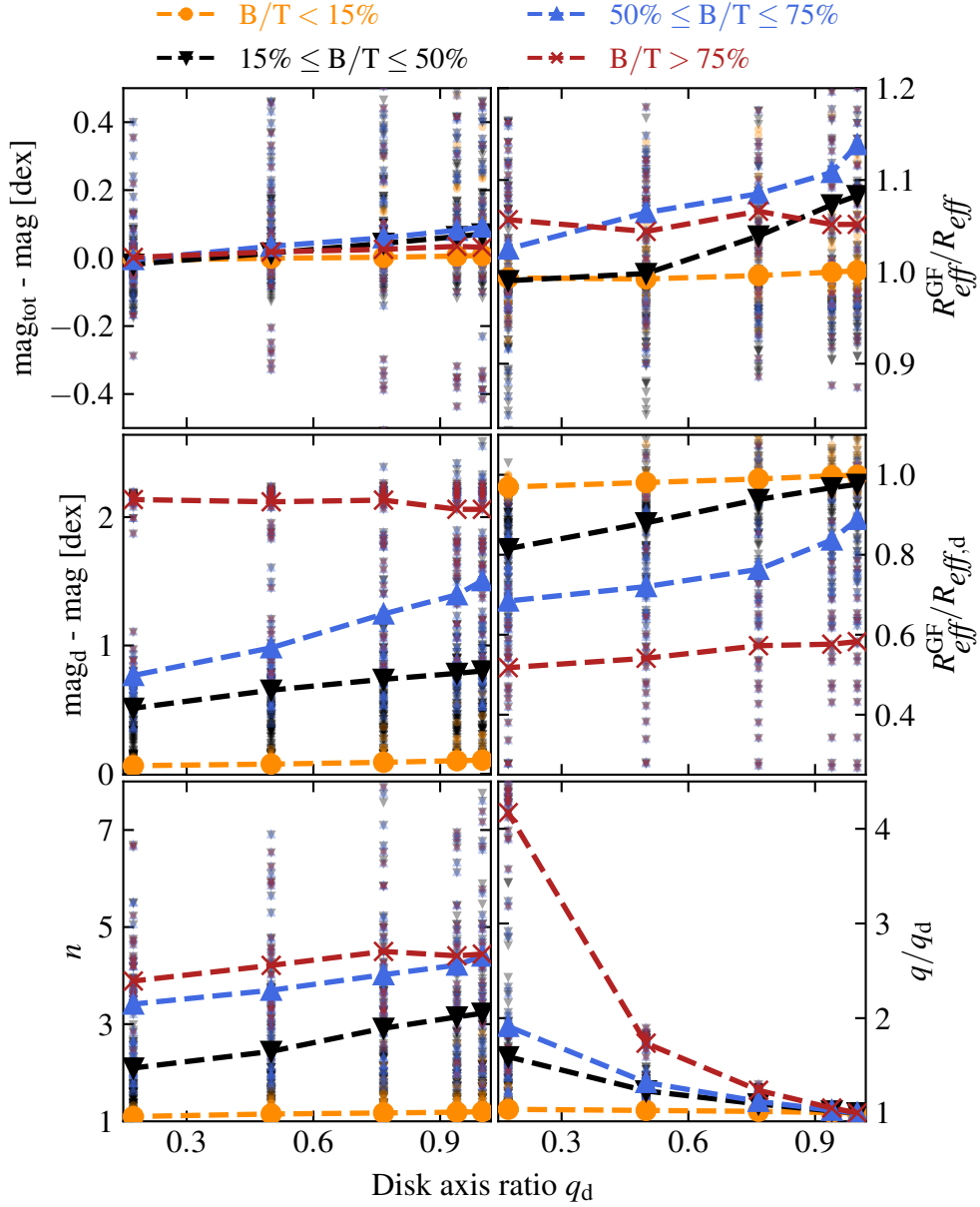
Figure 4.5: Variation of the best-fit parameters for various composite galaxy models with non negligible bulge contribution as a function of the true disk axis ratio and bulge-to-total flux ratio (B/T). Each model was fitted with GALFIT using a single Sérsic profile with free Sérsic index. The B/T values for each model are shown as small markers whereas the median values for each B/T are shown as large markers with dashed lines. From left to right and top to bottom: (i) difference between the true total magnitude (disk and bulge, noted \text{mag}_{\text{tot}} ) and that of the best-fit model ( \text{mag} ), (ii) ratio between the model effective radius ( R_{\text{eff}}^{\text{GF}} ) and the true global effective radius (noted R_{\text{eff}} , see Sect. 4.3.2 for its definition), (iii) difference between the true disk magnitude ( \text{mag}_{\text{d}} ) and that of the best-fit model, (iv) ratio between the model effective radius and the true disk effective radius R_{\text{eff,d}} , (v) best-fit Sérsic index, and (vi) ratio between the model axis ratio q and the true disk axis ratio q_{\text{d}} . Even if the global parameters (total magnitude and global effective radius) are quite well recovered, a single Sérsic fit overestimates the flux contained in the disk and its axis ratio while it underestimates its size, especially for large bulge contributions.
