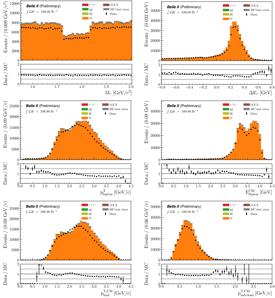
Figure E.1: Data-MC comparison in the 5 - 20\sigma sidebands of reconstructed \tau \rightarrow e\phi events for M_T , \Delta E_T and variables taken as inputs to the BDT, before the preselection.
