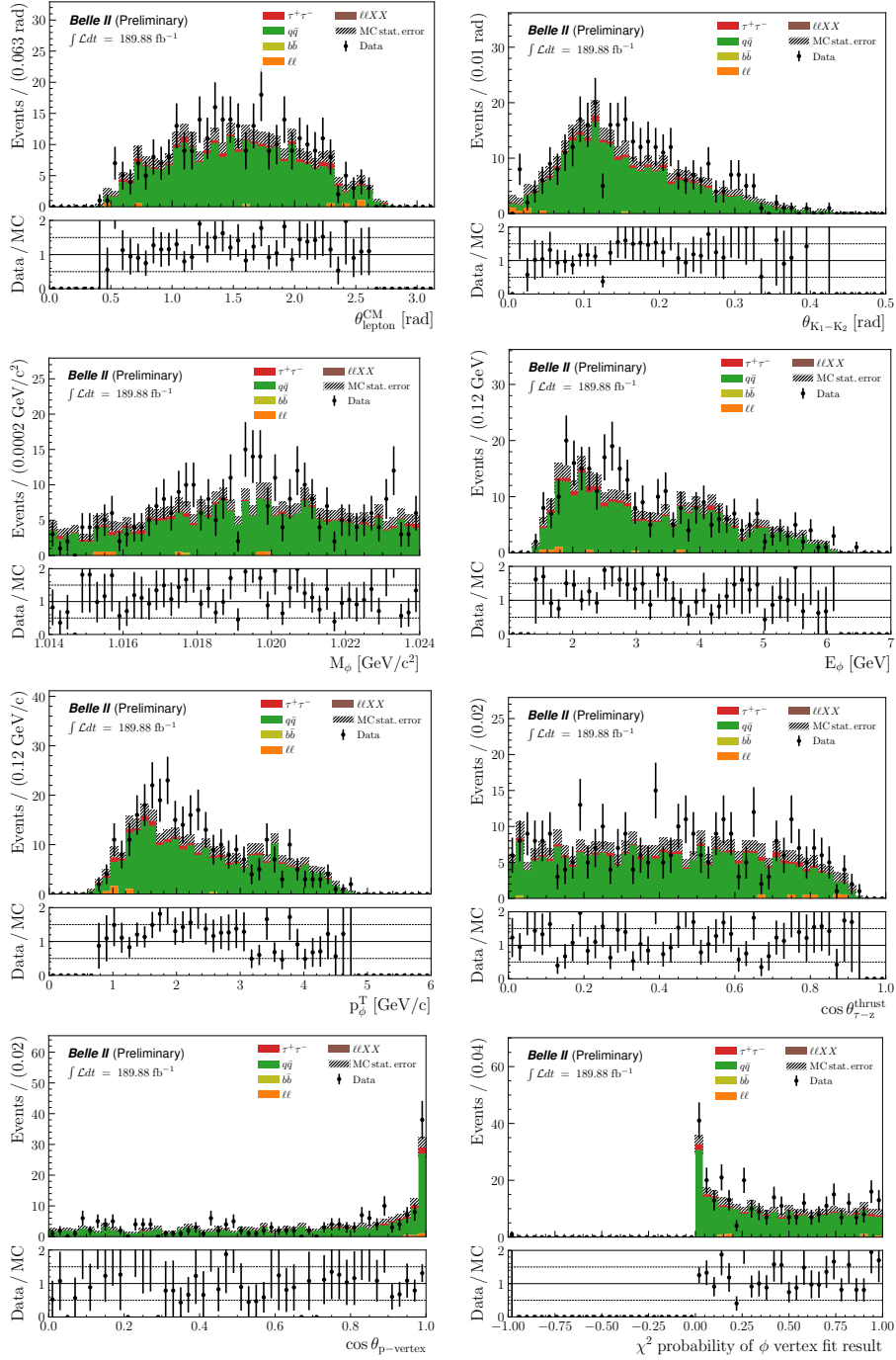
Figure E.4: Data-MC comparison in the 5 - 20\sigma sidebands of reconstructed \tau \rightarrow \mu\phi events for M_\tau , \Delta E_\tau and variables taken as inputs to the BDT, after the preselection.
