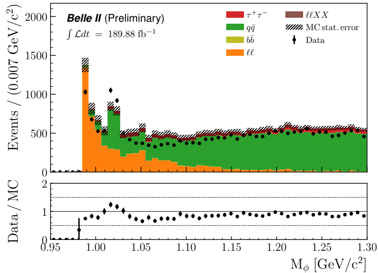
Figure 4.18: Data-MC comparison of the \phi mass ( M_\phi ) distributions in the 5 – 20 \sigma sidebands, for the \tau \rightarrow e\phi channel, after the preselection and with an enlarged mass window.
