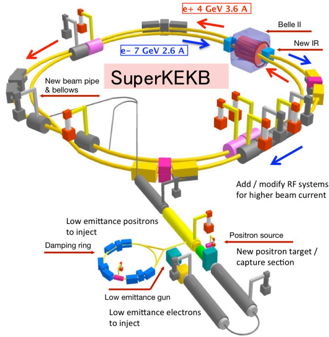
Figure 2.1: Schematic view of the SuperKEKB collider.
