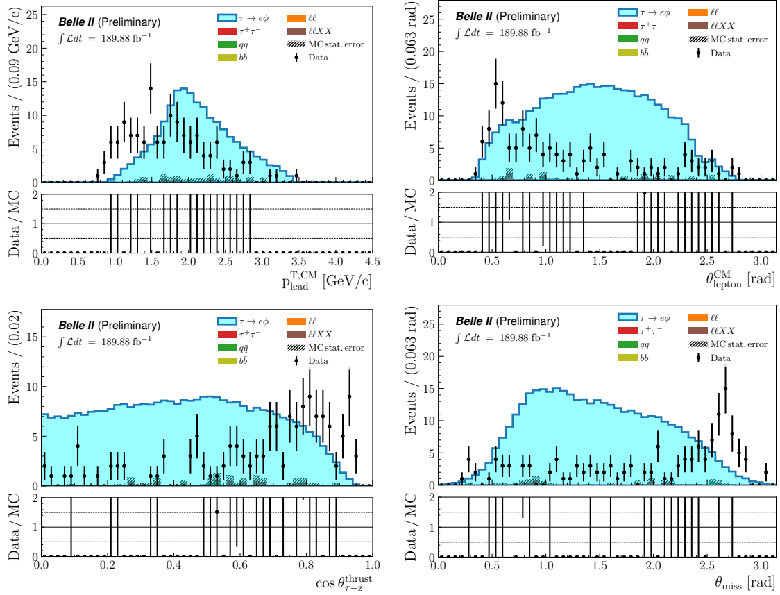
Figure 4.19: Data-MC comparison in the 5 – 20 \sigma sidebands after the preselection, the BDT and the 2D selections of variables used in the training of the data BDT. The signal MC distribution is rescaled to the data bin with highest yield.
