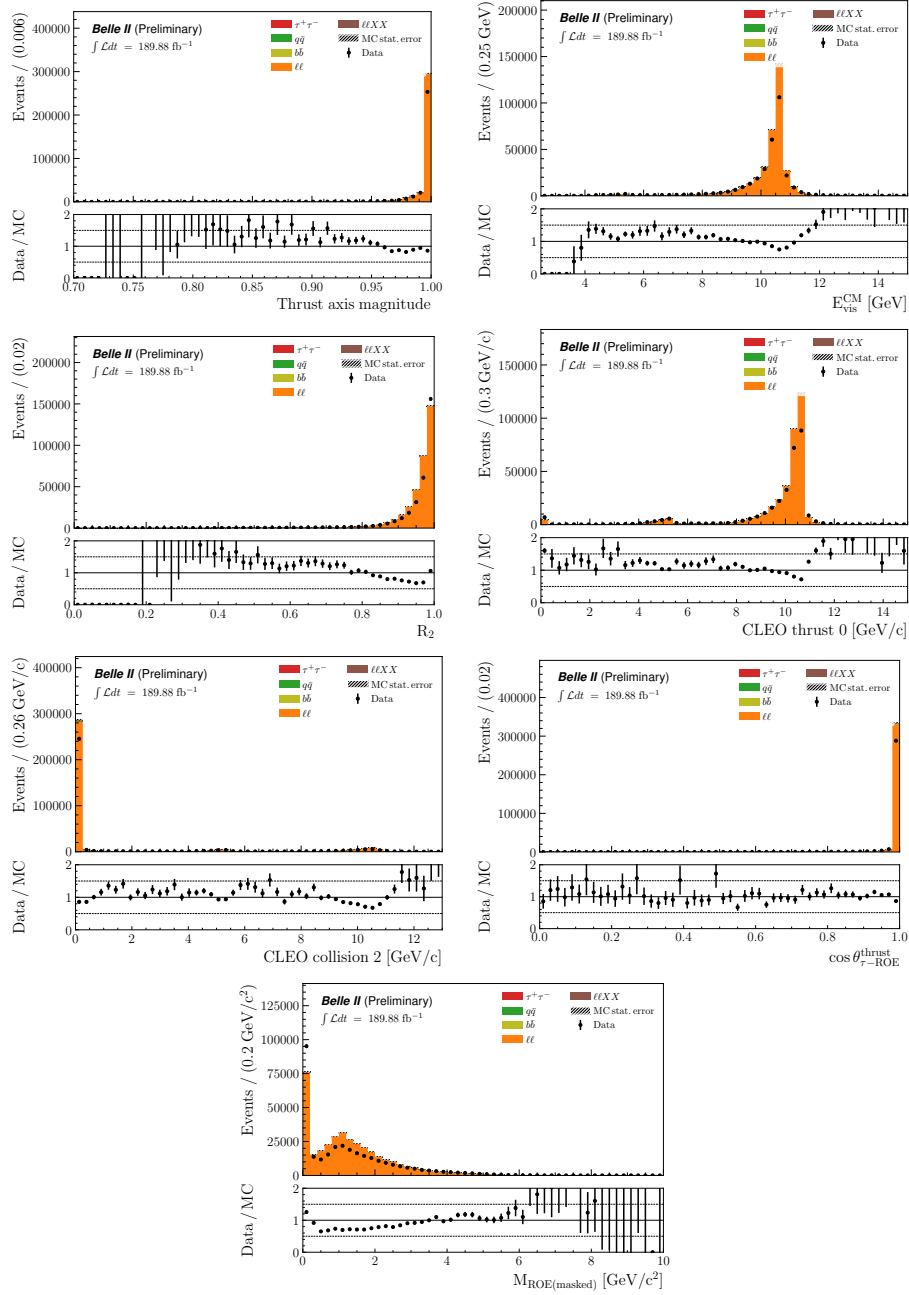
Figure E.1: Data-MC comparison in the 5 – 20 \sigma sidebands of reconstructed \tau \rightarrow e\phi events for M_\tau , \Delta E_\tau and variables taken as inputs to the BDT, before the preselection.
