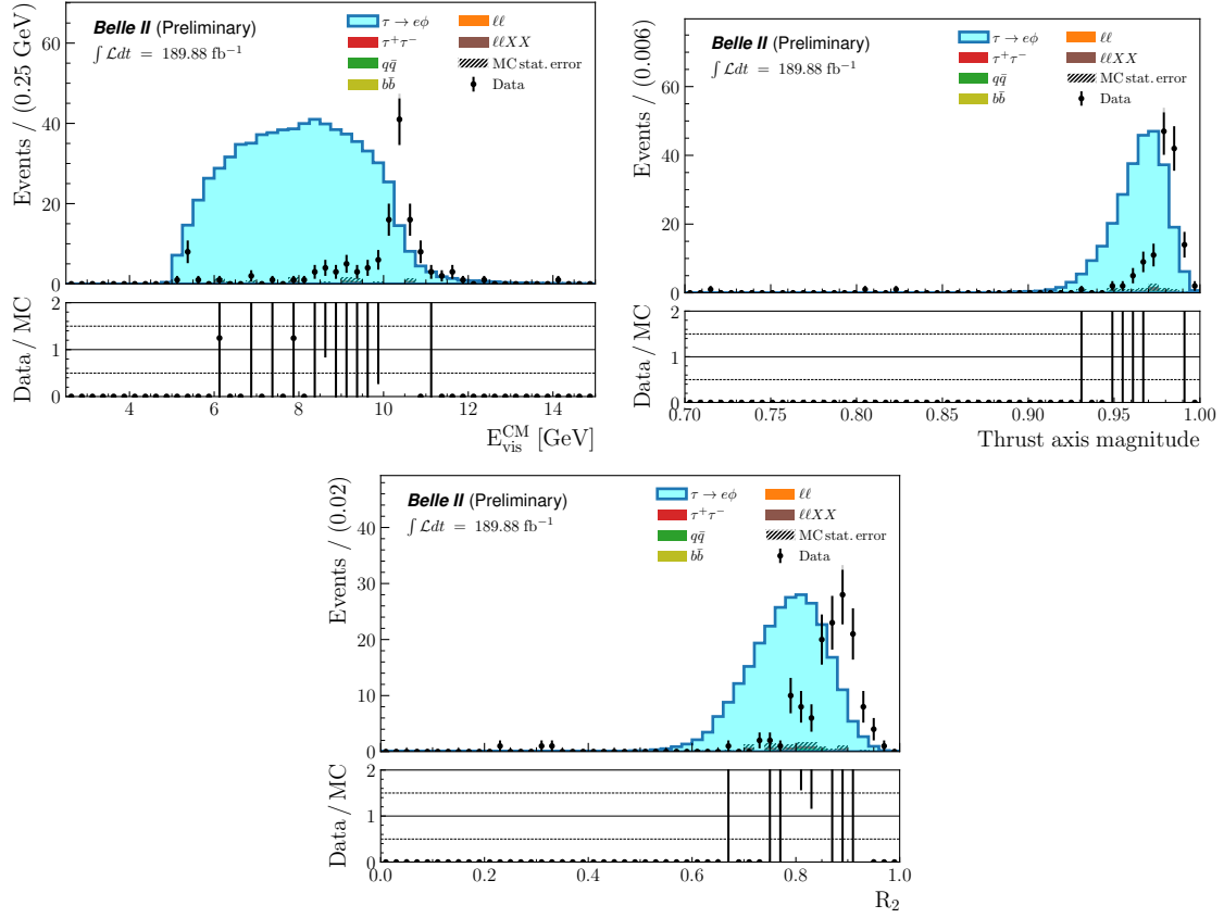
Figure 4.19: Data-MC comparison in the 5 - 20\sigma sidebands after the preselection, the BDT and the 2D selections of variables used in the training of the data BDT. The signal MC distribution is rescaled to the data bin with highest yield.
