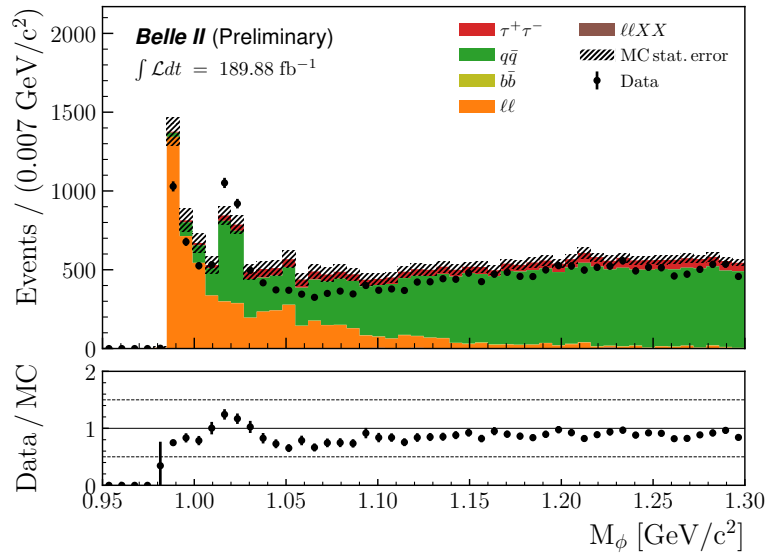
Figure 4.18: Data-MC comparison of the \phi mass ( M_\phi ) distributions in the 5 – 20 \sigma sidebands, for the \tau \rightarrow e\phi channel, after the preselection and with an enlarged mass window.
