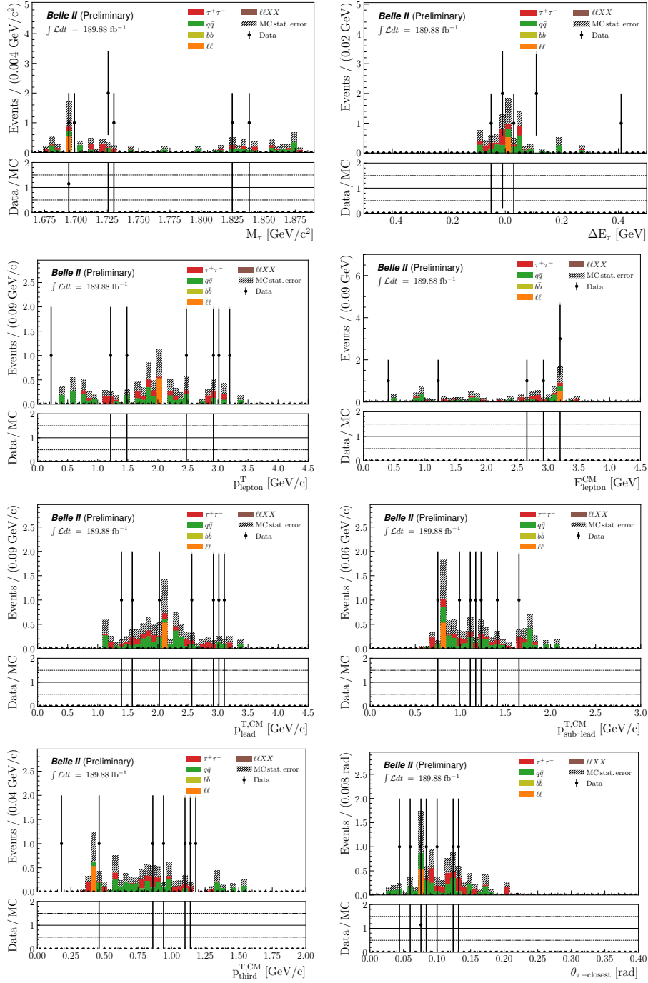
Figure E.7: Data-MC comparison in the 5–20 \sigma sidebands of reconstructed \tau \rightarrow \mu\phi events for M_\tau , \Delta E_\tau and variables taken as inputs to the BDT, after the full selection.
