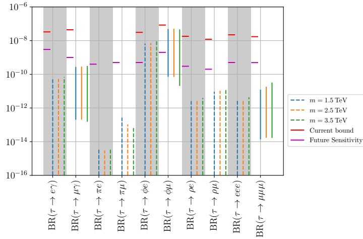
Figure 1.8: Current and expected upper limits (red and purple horizontal lines) on the branching fractions of lepton flavour violating \tau decay modes studied at the Belle II experiment, and predicted ranges at 90% C.L. in the U_1 leptoquark hypothesis for input masses m_U = 1.5, 2.5, 3.5 \text{ TeV}/c^2 (blue, yellow and green solid or dashed lines) [3].
