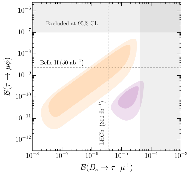
Figure 1.6: Two-dimensional branching fraction regions for \tau \rightarrow \mu\phi and B_s \rightarrow \tau^- \mu^+ processes, with 1\sigma (dark colour) and 2\sigma (light colour) uncertainties, in the hypothesis of a U_1 vector leptoquark. Two scenarios are shown, in orange or purple, for \beta_R^{b\tau} = 0 or \beta_R^{b\tau} = -1 (see Equation 1.43) respectively. The grey bands correspond to 95% confidence level (C.L.) upper limits from past experimental results. Projected limits from Belle II and LHCb, depending on the integrated luminosity, are indicated with dashed lines [1].
