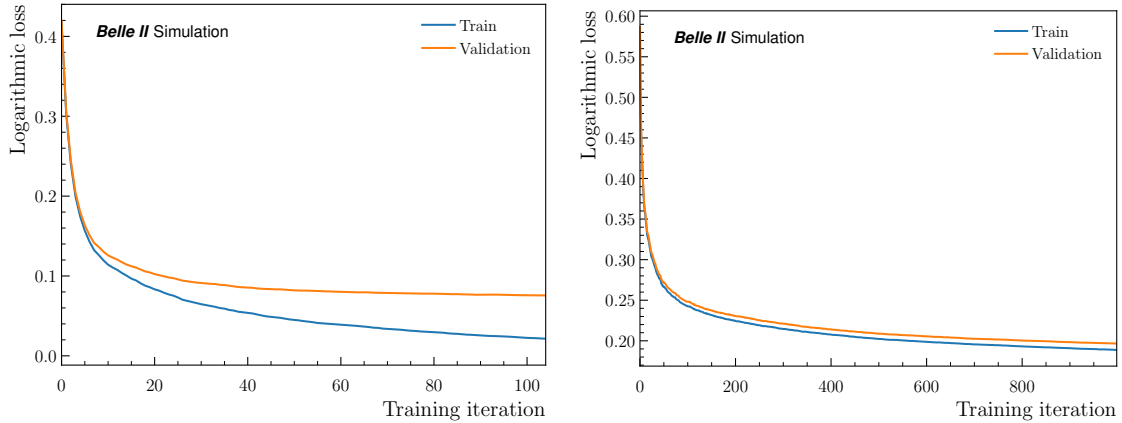
Figure 4.14: Logarithmic loss as a function of the training iteration, in the \tau \rightarrow e\phi (left) and \tau \rightarrow \mu\phi (right) channels. The ranges go up to the last iteration allowed by the early stopping.
