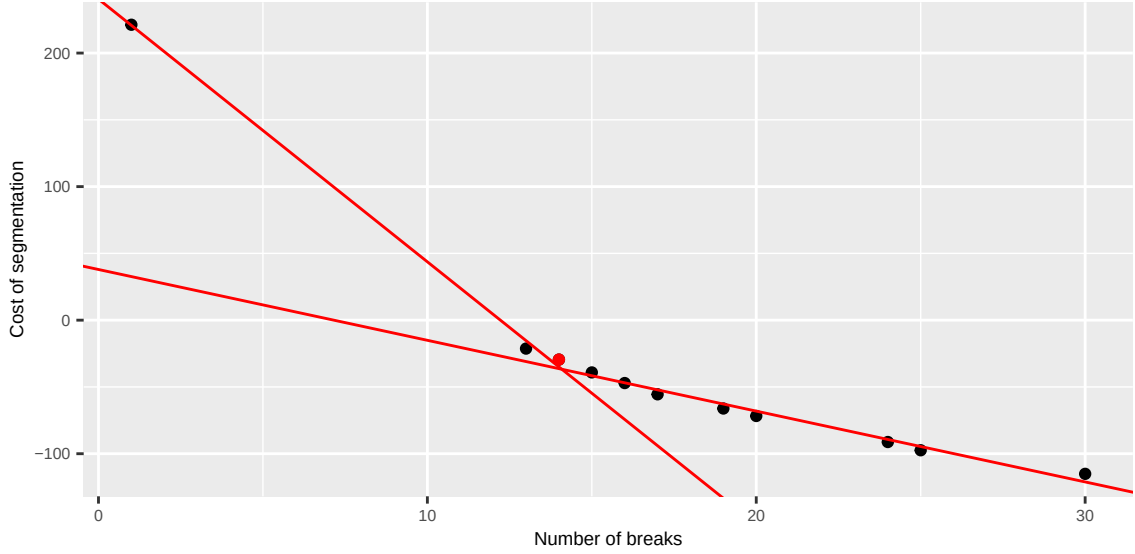
Figure 5.7: Elbow method selecting the optimal segmentation of the full signal \bar{\mathcal{D}} .
