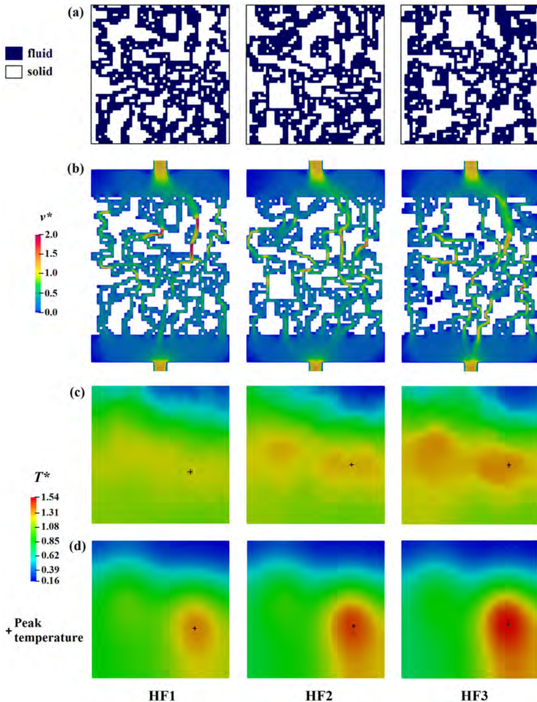
Figure 4.6 Influence of heat flux shape on the performance of GATO and RSC heat sinks. (a) optimized flow channel configuration; (b) velocity field ( z^* = -0.5 ) of the GATO heat sink; (c) temperature field at the heating surface of the GATO heat sink; (d) temperature field at the heating surface of the RSC heat sink.
