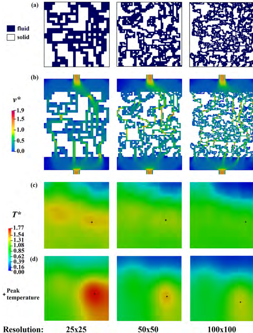
Figure 4.9 Influence of matrix resolution ( M_{r \times c} ) on the performance of GATO and RSC heat sinks. (a) optimized flow channel configuration; (b) velocity field ( z^*=-0.5 ) of the GATO heat sink; (c) temperature field at the heating surface of the GATO heat sink; (d) temperature field at the heating surface of the RSC heat sink.
