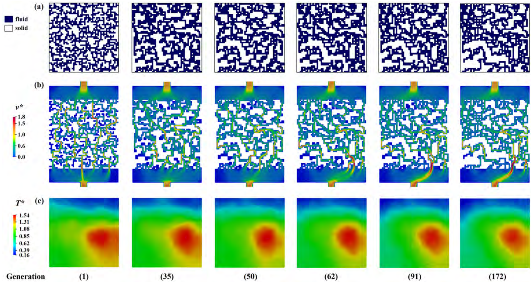
Figure 6.3 Top-ranked flow path configuration for RMSD_{T^*} minimization at generation 1, 35, 50, 62, 91, and 172. (a) Fluid/solid elements distribution in the design domain; (b) Corresponding velocity field at mid-channel depth; (c) Temperature field at the heating surface.
