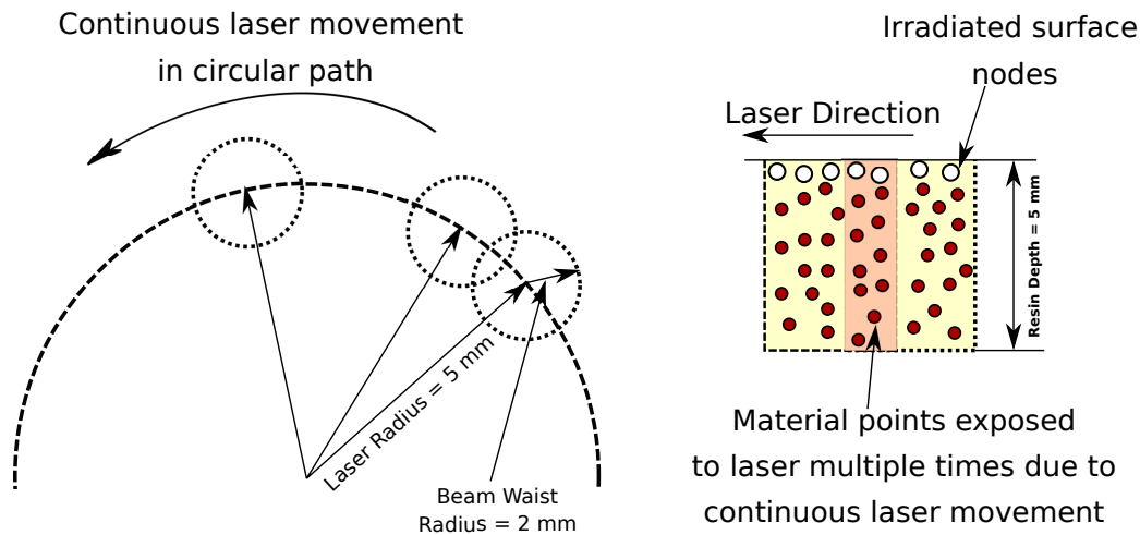
Figure 6.2. Laser path
