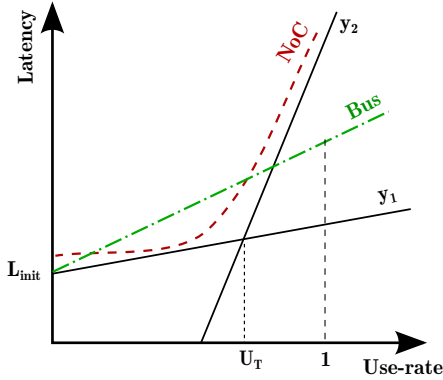
Figure 5.10 – Communication model
