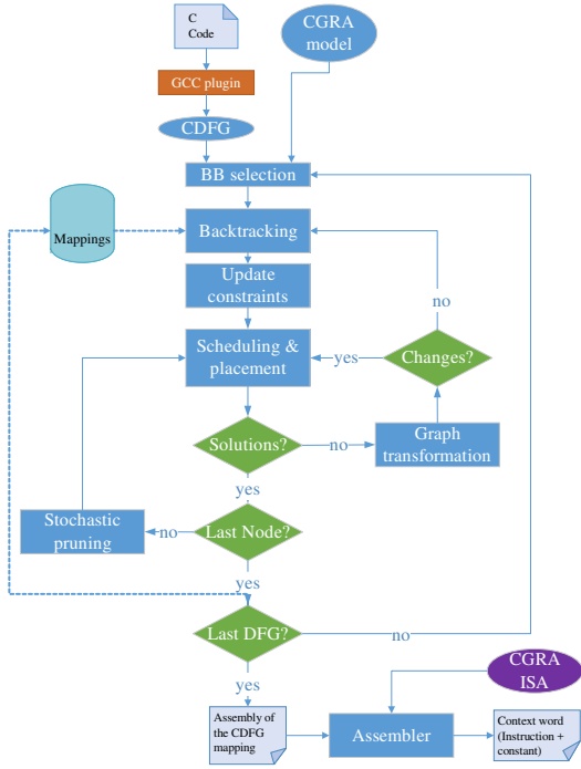
Figure 7: Compilation flow
