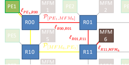
Figure 5.17 – Example on path declaration in the NoC
