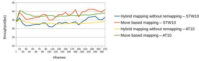
Figure 5.13 – Comparison of throughput for different mapping strategies for decoding Foreman sequence with MPEG4-SP
