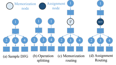
Figure 8: Graph transformation
