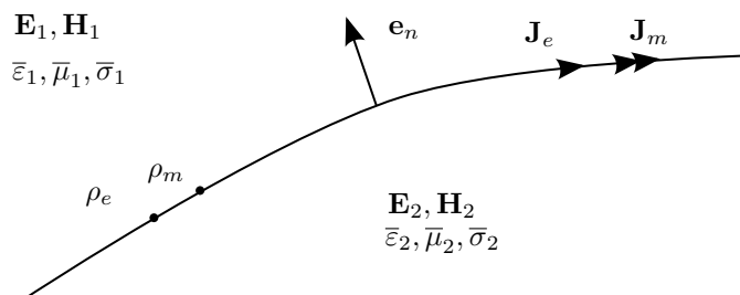
Figure 2.1: Field and flux density discontinuity across boundaries with electric/magnetic current and charge distributions. \mathbf{e}_n stands for the unit normal vector.
