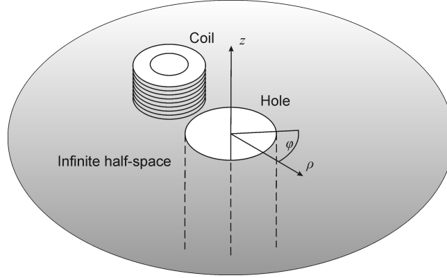
Figure 4.8: Borehole inspection using a cylindrical probe coil. The coil is located above the half-space interface and is moving parallel to it.
