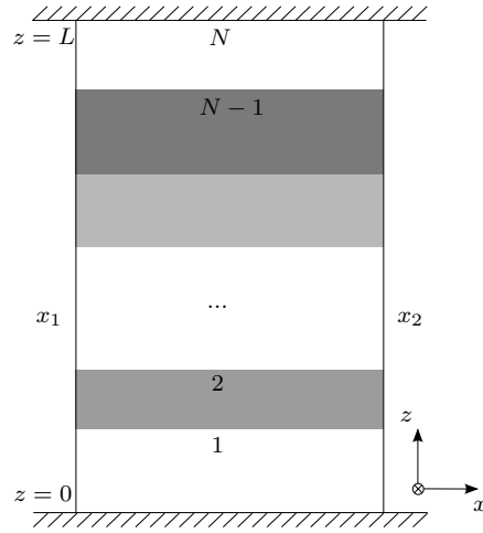
Figure 4.2: Planar multilayer medium of finite thickness.
