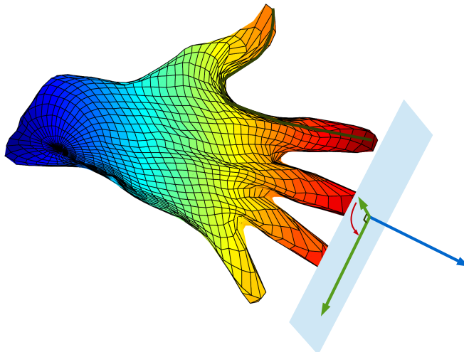
Figure 3.12: Scalar product on the tangent plan to the tip of the middle finger of a hand, and shortest path from the tip of the index finger to the tip of the thumb.
