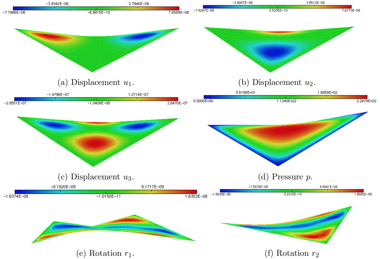
Figure 4.2: Solution on a hyperbolic paraboloid shell
