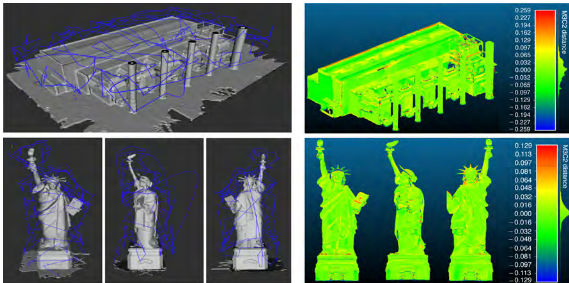
Figure 2.6: Numerical experiments: [top] Powerplant and [bottom] SoL: [left] Reconstructed mesh and 3D exploration path P_{0,f} (blue) of the quadrotor UAV (SR); [right] Signed distance error. The colour coding shows the error in meters with respect to the ground truth, computed with CloudCompare’s M3C2 algorithm.
