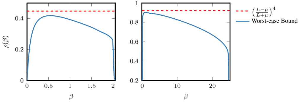
Figure 4.5: We plot \rho(\beta) , by solving a SDP reformulation of (4.22) with \mu/L = 0.1 (left) and \mu/L = 0.01 (right).
