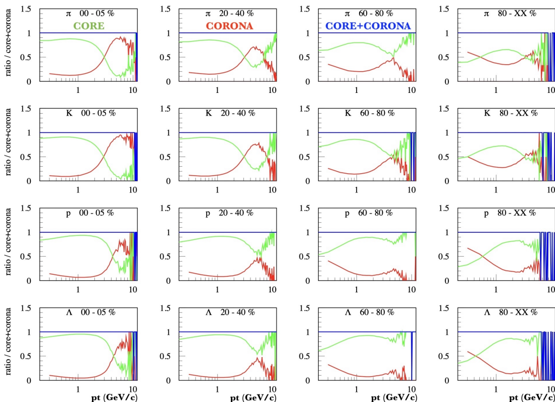
Figure 2.10: The ratios of core, corona, and core+corona to core+corona as a function of transverse momentum spectra for identified particles in Au-Au collisions at \sqrt{s_{NN}} = 200 GeV in mid-rapidity region |\eta| < 1 . For each particle, the transverse momentum spectra for most central (0-5%), mid-central (20-40%), mid-peripheral (60-80%), and most peripheral ( > 80\% ) collisions are plotted. The green, red, and blue curves represent the core, corona, and core+corona productions, respectively.
