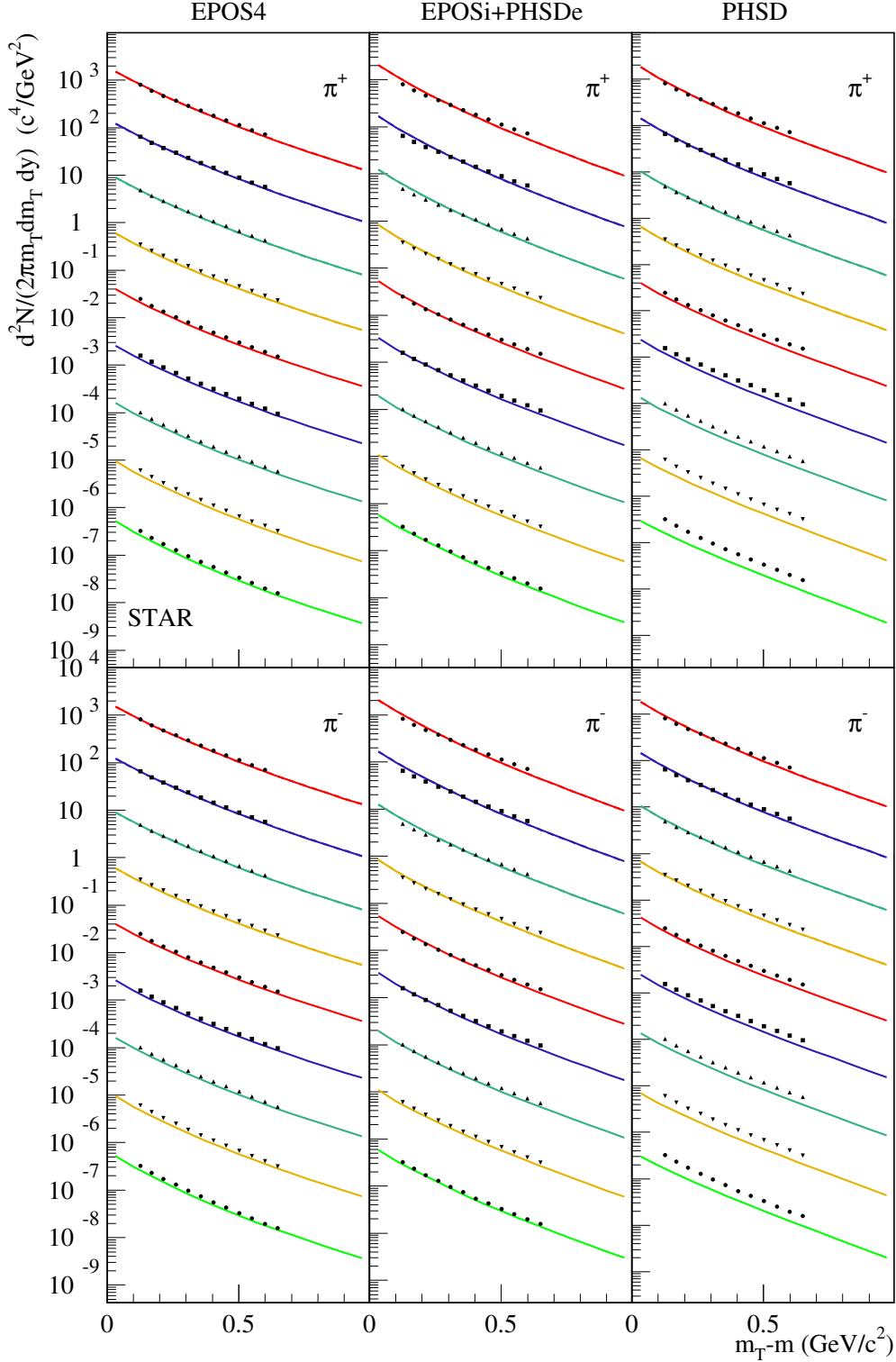
Figure 5.4: Invariant yield as a function of transverse mass for \pi^\pm for \text{Au-Au} collision at \sqrt{s_{NN}}=200 GeV at mid-rapidity ( |y| < 0.5 ) in three different simulations: EPOS 4 (left panel), EPOSi+PHSDe (middle panel), and pure PHSD (right panel). The different transverse mass spectra are plotted with different centrality ranges 0-5%, 5-10%, 10-20%, 20-30%, 30-40%, 40-50%, 50-60%, 60-70%, 70-80% from top to bottom in each plot. All the results compared to the STAR experimental data [160] with the black points. All curves and experimental data are scaled by 2 * 10^{-n} starting from the top most curve with 2 * 10^0 .
