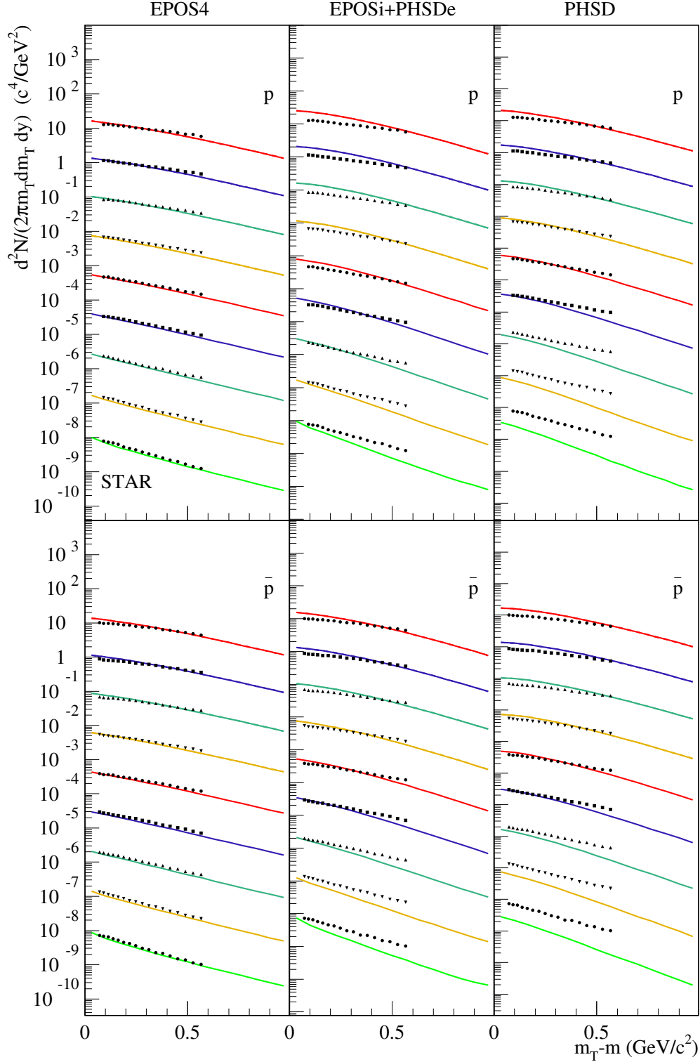
Figure 5.6: Invariant yield as a function of transverse mass for proton ( p ), and antiproton ( \bar{p} ) for \text{Au-Au} collision at \sqrt{s_{NN}} = 200 GeV at mid-rapidity ( |y| < 0.5 ) in three different simulations: EPOS 4 (left panel), EPOSi+PHSDe (middle panel), and pure PHSD (right panel). The different transverse mass spectra are plotted with different centrality ranges 0-5%, 5-10%, 10-20%, 20-30%, 30-40%, 40-50%, 50-60%, 60-70%, 70-80% from top to bottom in each plot. All the results compared to the STAR experimental data [160] with the black points. All curves and experimental data are scaled by 2 * 10^{-n} starting from the top most curve with 2 * 10^0 .
