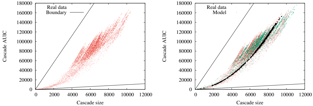
Figure 2.8 – Comparative scatterplots of the cascade sizes and AUIC in the real data and the 2-phase model. The black solid lines represent the theoretical boundaries outside which no cascade can exist, black dots correspond to model cascades with a similar linear growth rate ( 300 \pm 5 infected holdings per day).
