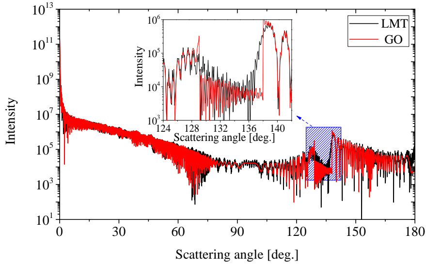
Figure 2.15 – Comparison the scattering diagrams of a sphere between LMT and GO in perpendicular polarization. The forward diffraction is also included here. The incident plane wave with wavelength \lambda = 0.6328 \mu\text{m} is in perpendicular polarization. The radius of particle and its refractive index are a = 100 \mu\text{m} and m = 1.333 .
