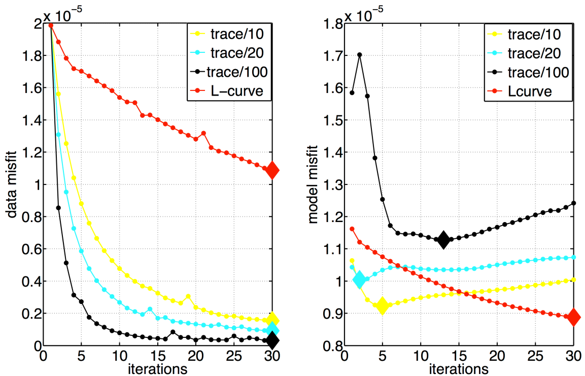
Figure 6.14: Data and model misfits evolution with iterations for four regularization parameter applied to the v -method and a feedback value of 0.1.
