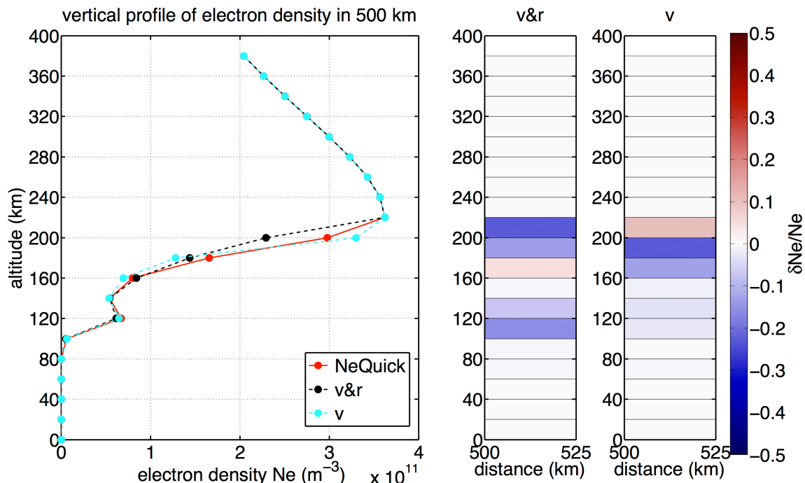
Figure 7.16: Vertical profiles of electron density at 500 km distance from the radar using data from December 13, 2008 measured in 67^\circ azimuth. The electron density perturbation of one point in the left plot corresponds to the block starting from the altitude of the point in the right plot.
