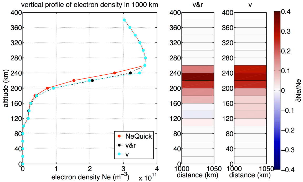
Figure 7.11: Vertical profile of electron density in 1000 km distance from the radar calculated from real data inversion of OTH radar Nostradamus. The data was collected march 14, 2006 in azimuth 247^\circ . The electron density perturbations \delta Ne/Ne obtained by inversion are shown in the two subplots in the right. The electron density perturbation of one point in the left plot corresponds to the block starting from the altitude of the point in the right plot.
