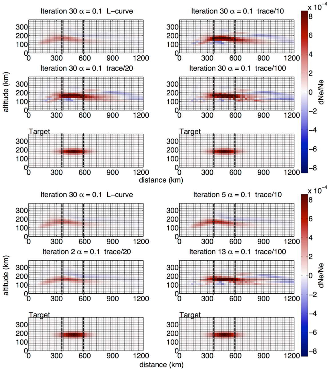
Figure 6.15: Effect of regularization on the iterative v -method. Inversion results with the v -method at model misfit (bottom panel) and data misfit (top panel) minima in Figure 6.14. For all four methods, a feedback value of 0.1 was applied.
