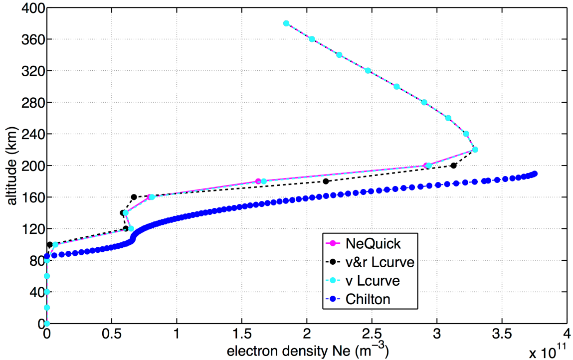
Figure 7.19: Comparison of the vertical profile of electron density obtained at the ionosonde station Chilton (blue) December 19, 2008 with the one obtained by ionospheric tomography using the v - and the v&r -method.
