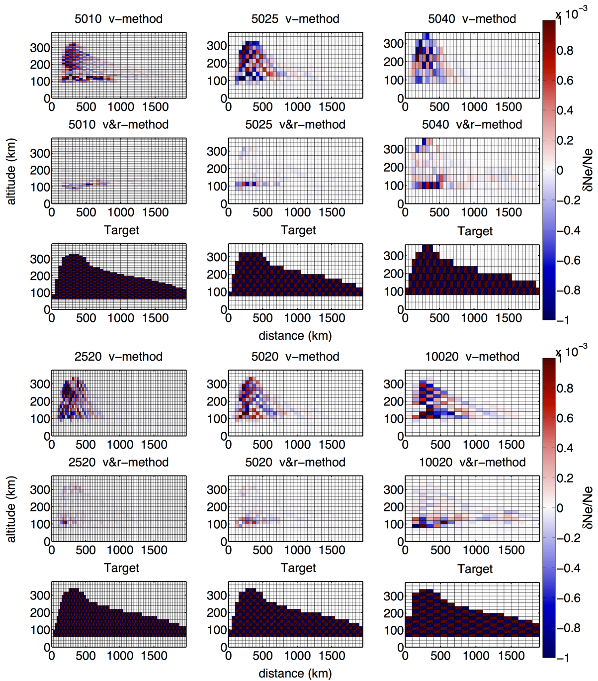
Figure 5.5: Inversion results for a checkerboard perturbation of 0.1% using the v and the v&r -method. The cell dimensions are fixed to 50 km in distance and enlarged in altitude from 10 km, to 25 km and 40 km in the top panel. In the bottom panel, cell dimensions are fixed to 20 km in altitude and enlarged from 25 km to 50 km and 100 km in distance. The sign of the perturbations is alternating from cell cell (radically).
