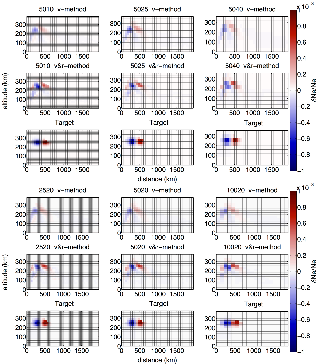
Figure 5.6: Inversion results for two localized perturbation of 0.1% using the v - and the v&r -method. The cell dimensions are fixed to 50 km in distance and increased in altitude from 10 km, to 25 km and 40 km in the top panel. In the bottom panel, cell dimensions are fixed to 20 km in altitude and enlarged from 25 km to 50 km and 100 km in distance.
