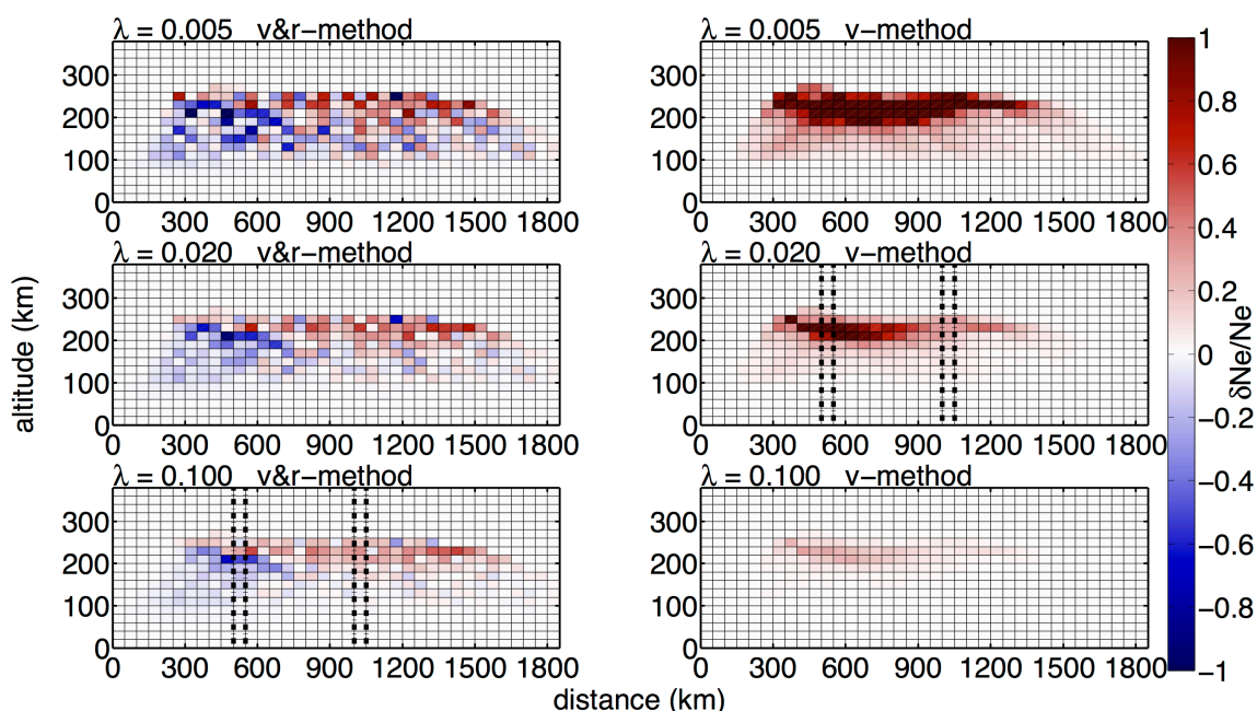
Figure 7.9: Real data inversion for data of March 14, 2006 at 1855 UT in azimuth 247^\circ . In the v\&r -method (left) and the v -method (right), different values of regularization \lambda were used. The grid size is 50 \times 20 km in distance and altitude. The results for the best regularization parameter are shown in the bottom left and the middle right plot, respectively.
