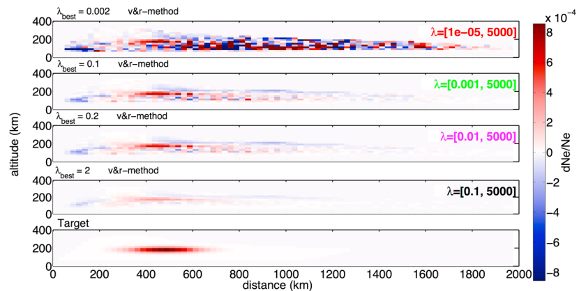
Figure 7. Inversion results using the v and r method with the best value of regularization chosen from the L curves in Figure 6a for the localized perturbation in order to explore the sensitivity to the \lambda range. The bottom row shows the target model.
