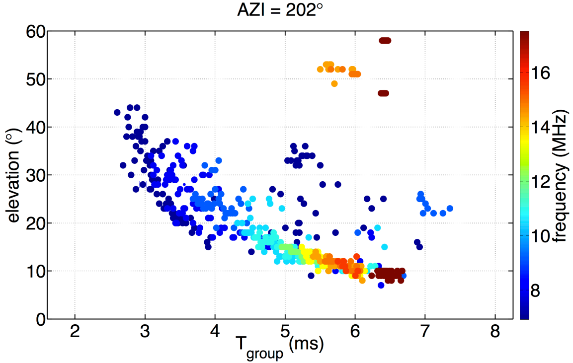
Figure 7.1: Real data (group propagation time as function of elevation angle) obtained from the OTH radar Nostradamus on March 14, 2006 at 1855 UT in azimuth 202°. The frequency is color coded.
