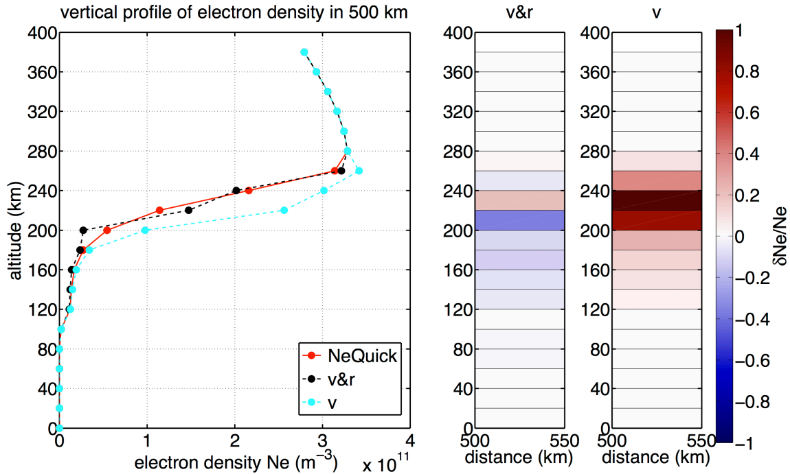
Figure 7.10: Vertical profile of electron density in 500 km distance from the radar calculated from real data inversion of OTH radar Nostradamus. The data was collected March 14, 2006 in azimuth 247^\circ . The electron density perturbations \delta Ne/Ne obtained by inversion are shown in the two subplots in the right. The electron density perturbation of one point in the left plot corresponds to the block starting from the altitude of the point in the right plot.
