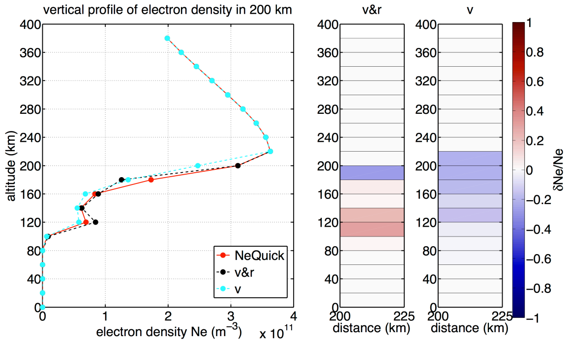
Figure 7.15: Vertical profiles of electron density at 200 km distance from the radar using data from December 13, 2008 measured in 67^\circ azimuth. The electron density perturbations are obtained from the inversion in Figure 7.14 for the best regularization parameter. The electron density perturbation of one point in the left plot corresponds to the block starting from the altitude of the point in the right plot.
