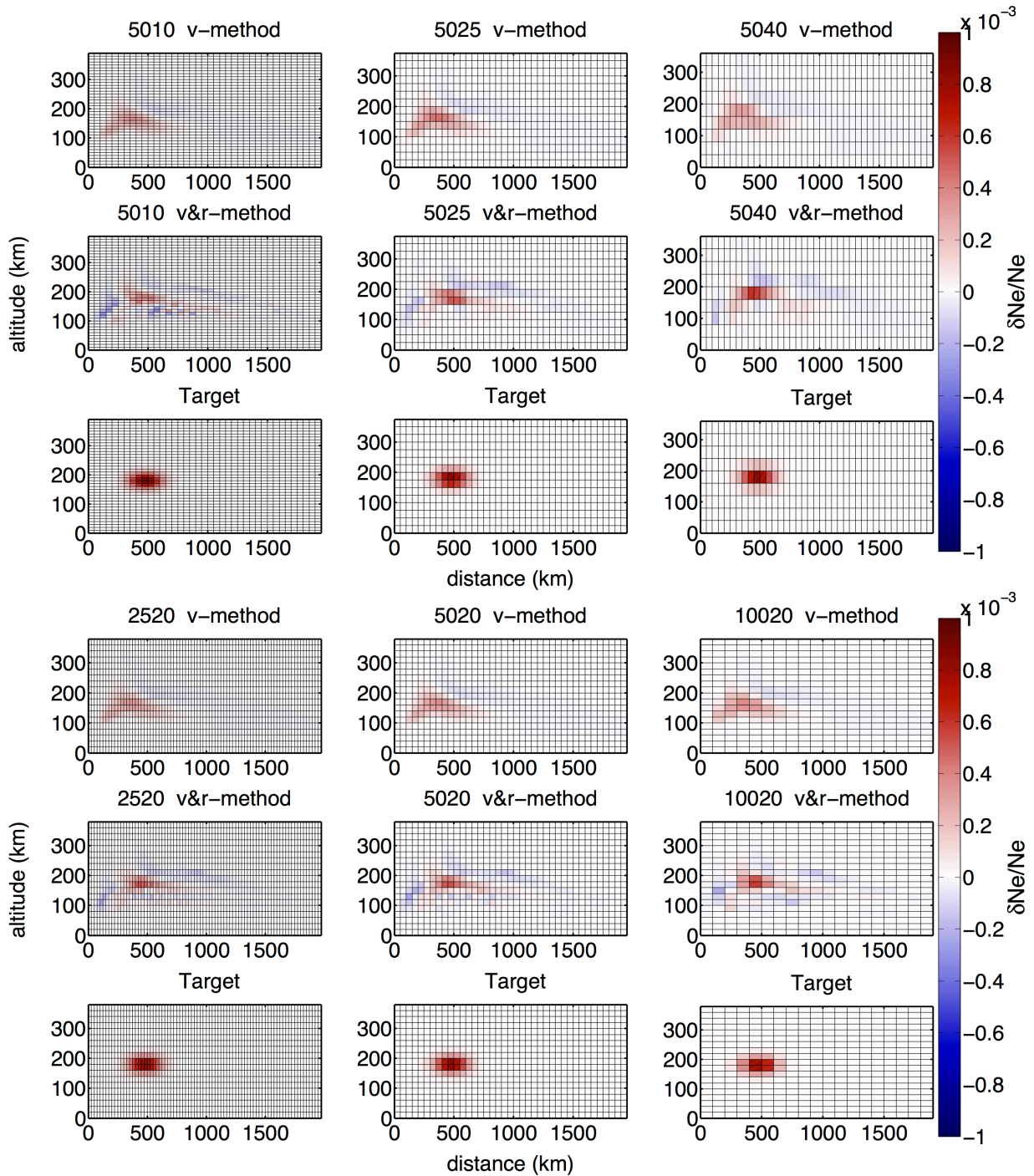
Figure 5.2: Inversion results for a localized perturbation of 0.1% using the v and the v&r -method. The cell dimensions are fixed to 50 km in distance and increased in altitude from 10 km to 25 km and 40 km in the top panel. In the bottom panel cell dimensions are fixed to 20 km in altitude and enlarged from 25 km to 50 km and 100 km in distance.
