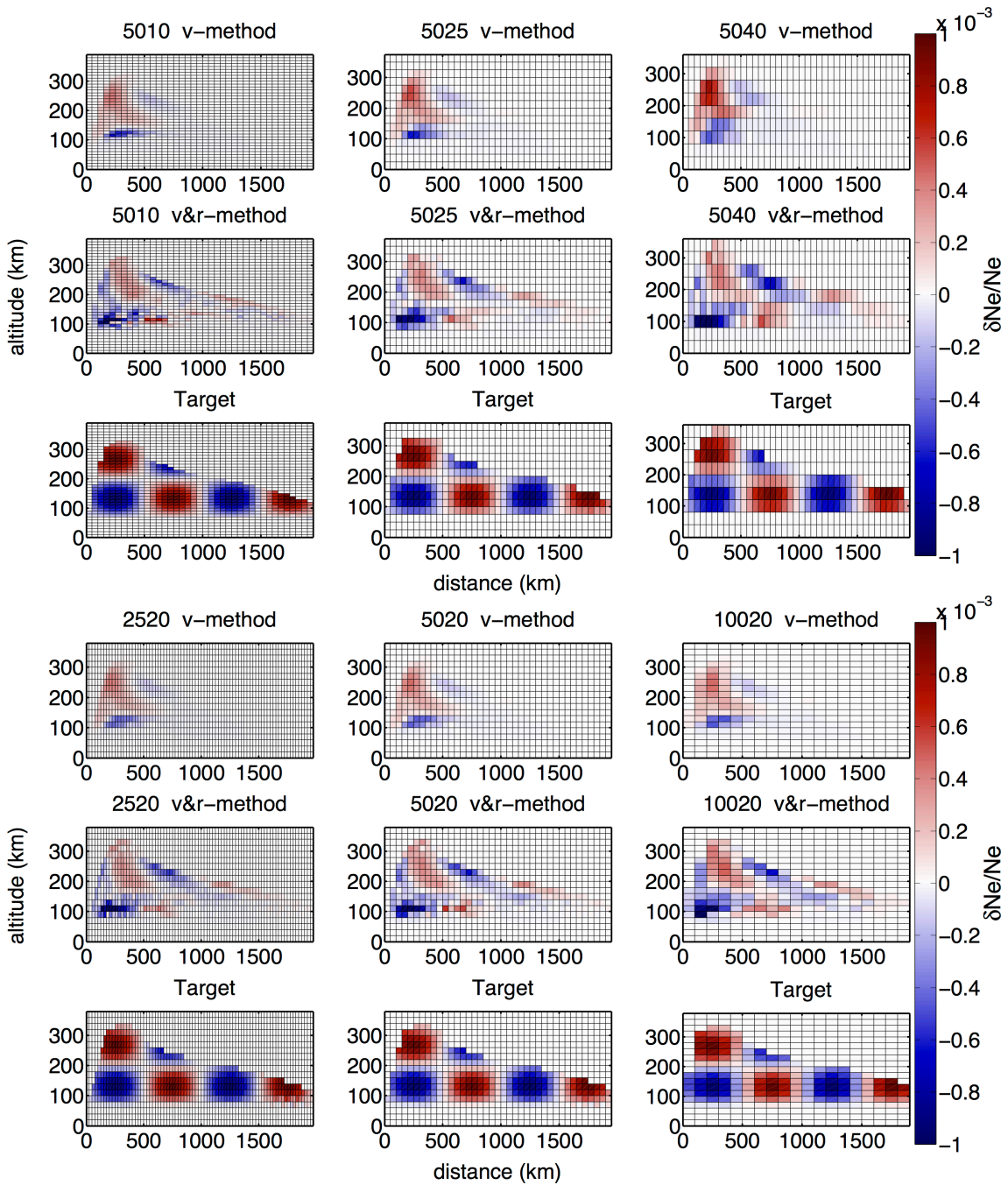
Figure 5.3: Inversion results for a checkerboard perturbation of 0.1% using the v - and the v&r -method. The cell dimensions are fixed to 50 km in distance and enlarged in altitude from 10 km, to 25 km and 40 km in the top panel. In the bottom panel, cell dimensions are fixed to 20 km in altitude and enlarged from 25 km to 50 km and 100 km in distance.
