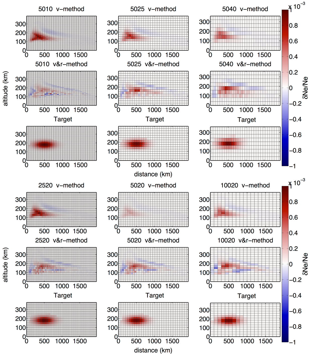
Figure 5.1: Inversion results for a localized perturbation of 0.1% using the v -method and the v&r -method. The cell dimensions are 50 km in distance and varied in altitude from 10 km to 25 km and 40 km in the top panel. In the bottom panel, cell dimensions are 20 km in altitude and varied from 25 km to 50 km and 100 km in distance.
