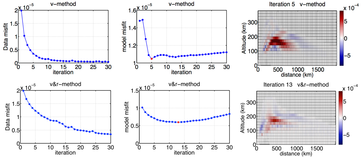
Figure 6.3: Data misfit \sum_{j=1}^{rays} \left(\frac{\delta \mathbf{T}}{\mathbf{T}}\right)_j and model misfit as a function of iterations for the v -method (top) and the v\&r -method (bottom). The inversion results for the minimum (red point) of the model misfit (iteration 5 for v -method and iteration 13 for v\&r -method) are shown on the right panels.
