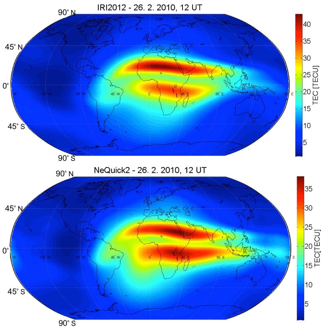
Figure 2.5: Global ionospheric TEC maps for 26th February 2010 at 12 UT modeled by the empirical models NeQuick and IRI. Although they are different in the way they model the ionosphere, they both distinguish the equatorial anomaly. Source: Najman and Kos (2014)
