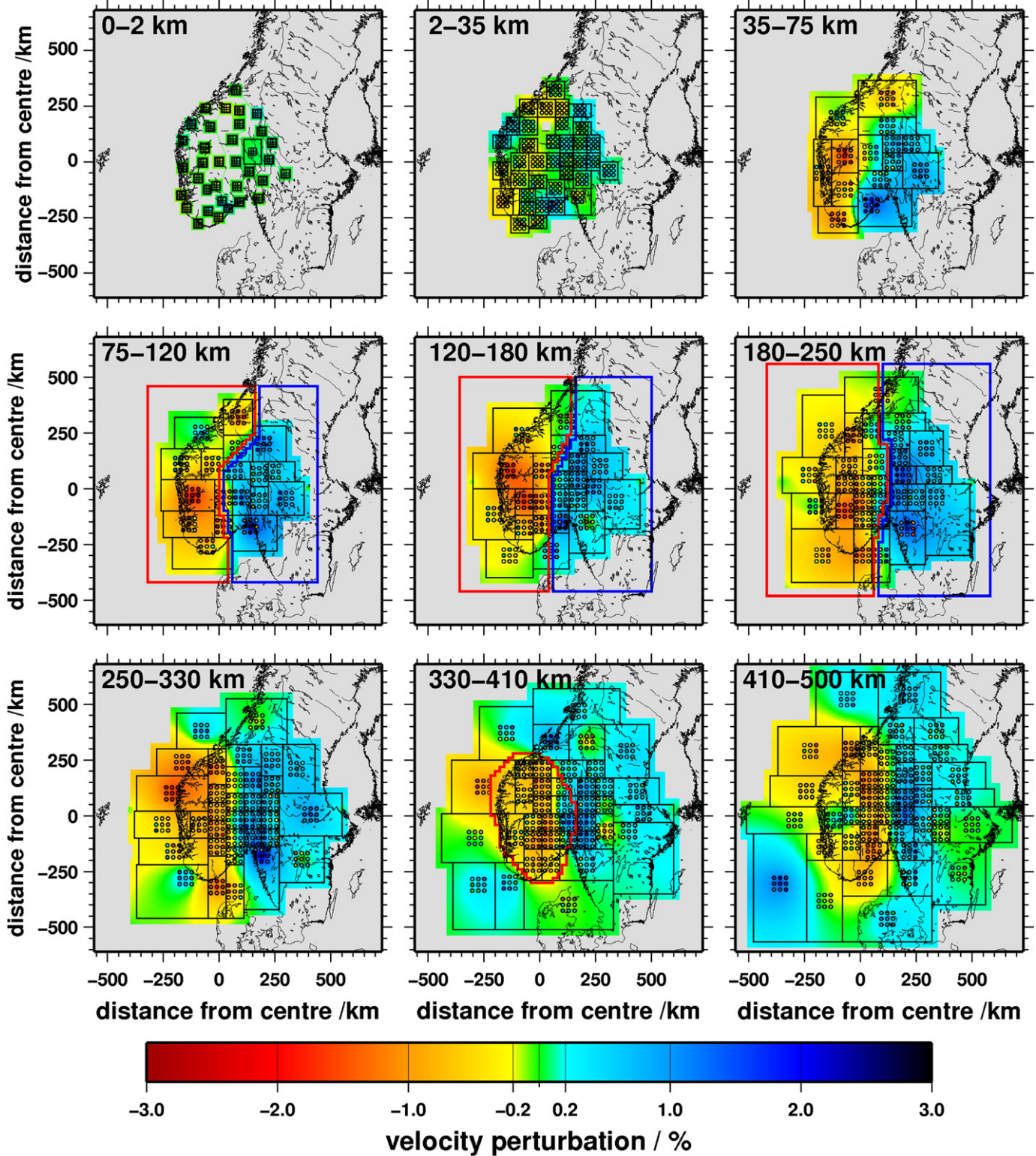
Fig. 12. Reconstruction test AT2 (anomaly pattern test 2). The pre-set synthetic anomalies are placed in the velocity model at 75–250 km depth (blue outline: +1.5% v_s , red outline: -1.5% v_s ) in addition to a stronger synthetic anomaly (red outline: -2.5% v_s ) at 330–410 km depth. These anomalies represent v_s contrasts as found in the real model (Fig. 7). The interpolated S-wave velocity distribution visualises the corresponding inversion result after applying the offset and averaging technique (vertical cross sections see Supp. Fig. S3). Additionally, the circles show the inversion results of the individual nine offset inversion models before averaging. This reconstruction test illustrates a good reproduction (position and amplitude) of the synthetic anomalies, although some vertical smearing is visible.
