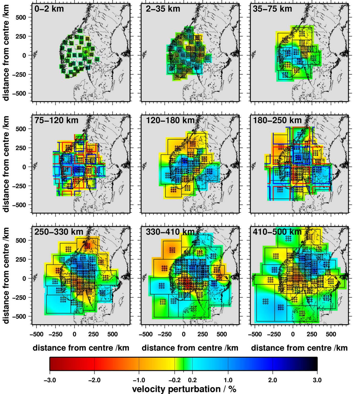
Fig. 10. Reconstruction test CBT (checkerboard pattern test). The pre-set synthetic anomalies (blue outline: +1.5% v_s , red outline: -1.5% v_s ) are placed in the velocity model at 75–120 km and 180–250 km depth. The interpolated S-wave velocity perturbations visualise the corresponding inversion result after applying the offset and averaging technique. Additionally, the circles show the block-wise inversion results of the individual nine offset inversion models before averaging. There is strong vertical smearing which leads to reduced vertical resolution within the model space.
