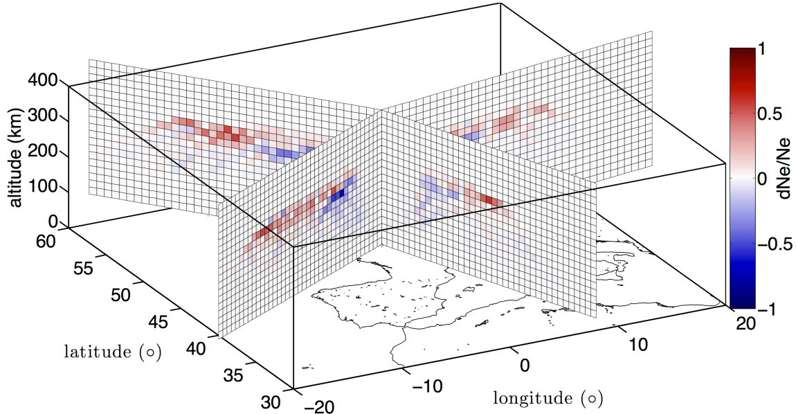
Figure 7.12: Electron density perturbation obtained by real data inversion. The data as collected at OTH radar Nostradamus March 14, 2006, at 1855 UT in four azimuth directions, nominally 67^\circ , 157^\circ , 247^\circ and 337^\circ . Source: Roy et al. (2014)
