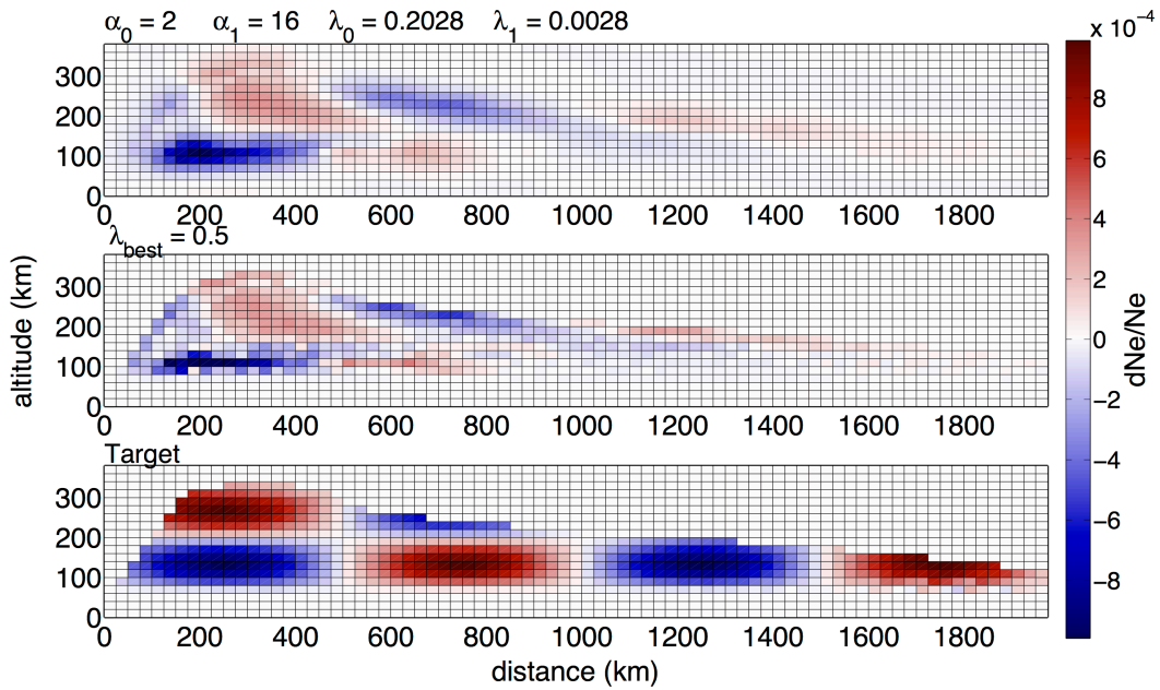
Figure 4.16: Damped least squares inversion vs. damped least squares with constraints for a checkerboard perturbation. From bottom to top: Target model, damped least squares inversion with the best regularization parameter \lambda_{best} chosen from the L -curve, and damped least squares inversion with constraints.
