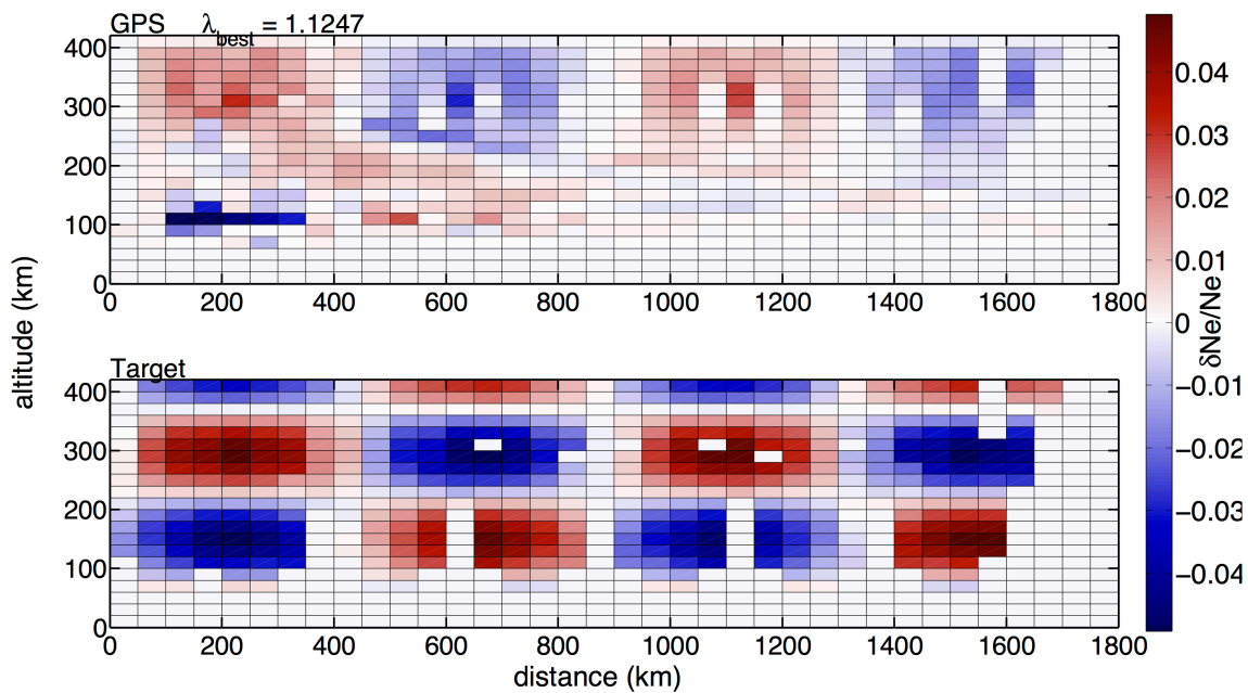
Figure 7.20: Joint inversion of OTH radar and GPS (top) using simulated data for a checkerboard perturbation of 5%. Perturbation gaps in the target model are due to missing ray-paths. The grid size is 50 \times 20 km in distance and altitude, respectively.
