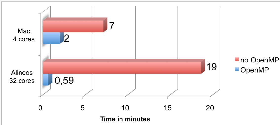
Figure 6.2: Computational costs for tracing \sim 10^3 rays on a grid with 1000 pixels for the v -method. The execution time in parallel (openMP) and on a single processor is compared using a Mac laptop with four and a 32 core desktop computer.
