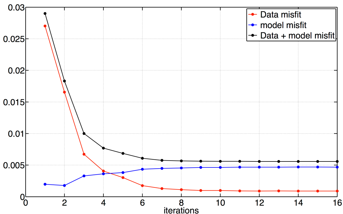
Figure 4.23: Data and model misfit (equation 4.45) as a function of iterations for the Conjugate Gradient Method applied to a checkerboard perturbation.
