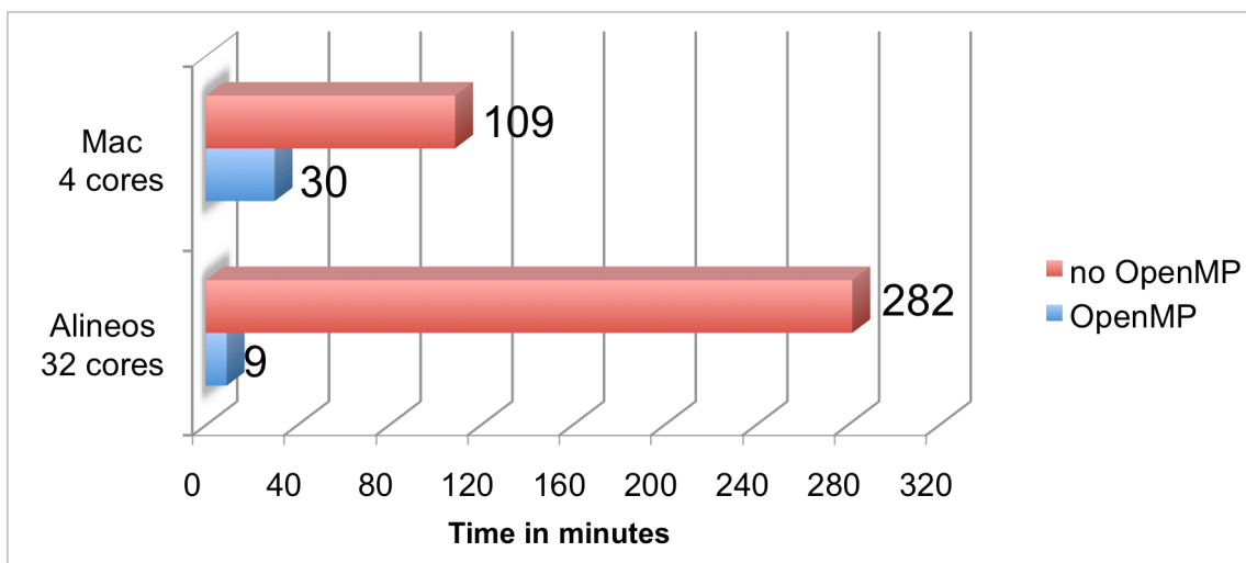
Figure 6.1: Computational costs for numerical calculation of ray-path deflection in the v&r -method for \sim 10^3 rays on a grid with 1000 pixels. The execution time in parallel (openMP) and on a single processor is compared using a Mac laptop with four cores and a 32 core desktop computer.
