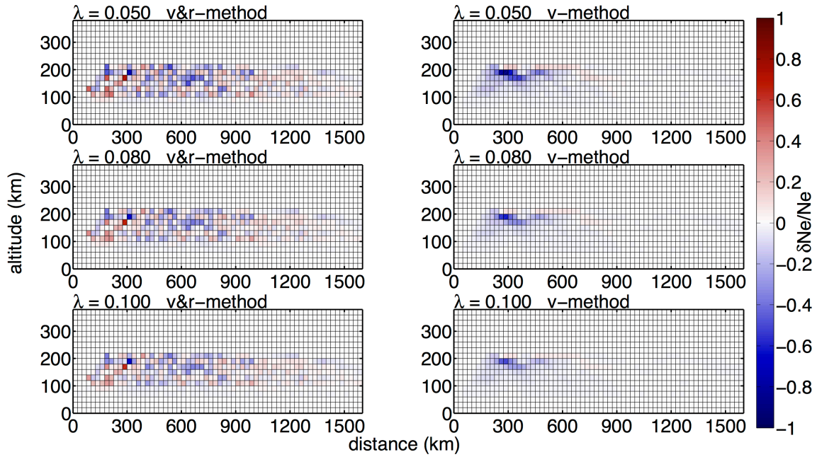
Figure 7.14: Real data inversion for data of December 13, 2008 at 1154 UT in azimuth 67^\circ . In the v&r-method (left) and the v-method (right), different values of regularization \lambda were used. The grid size is 25 \times 50 km in distance and altitude, respectively.
