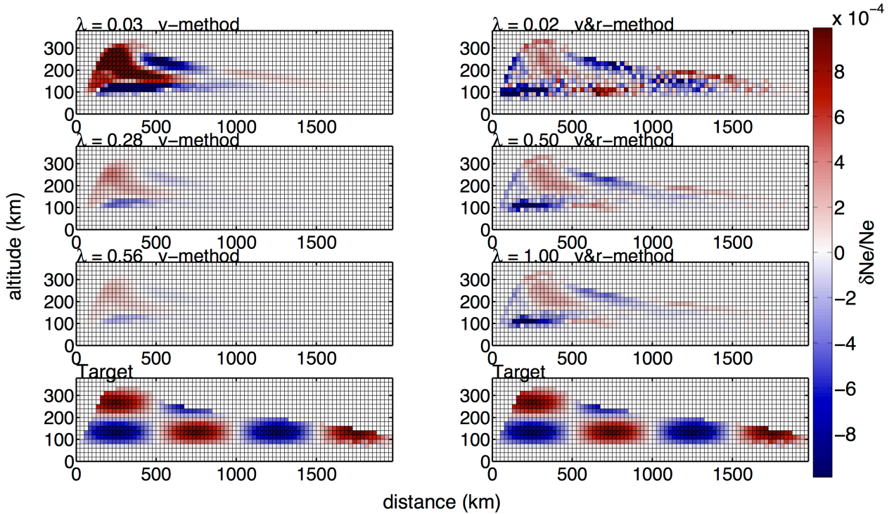
Figure 4.11: Inversion results for the v -method (left) and v&r -method (right) for a checkerboard perturbation of 0.1 % using different regularization parameter. The inversions for the best regularization parameter are shown in the second plot from the top.
