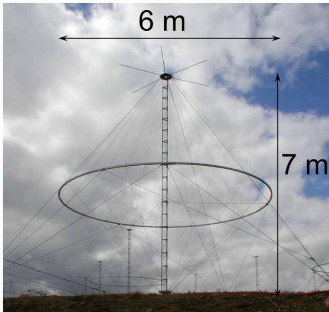
Figure 3.3: Example of an antenna of Nostradamus. Source: Molinié (2011)
