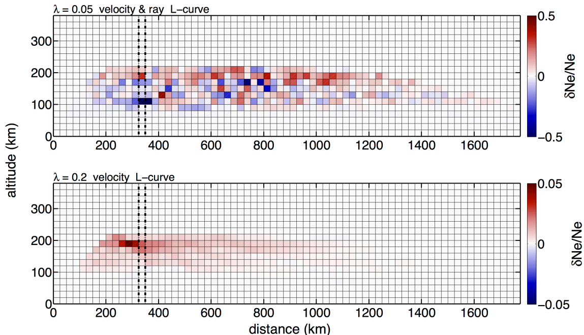
Figure 7.18: Inversion results using real data measured by OTH radar Nostradamus December 19, 2008 at noon in 337^\circ azimuth. v\&r -method (top) and v -method (bottom). The perturbations found at distances marked by dashed lines were used to correct a vertical profile of electron density from the a priori ionospheric model and are shown in Figure 7.19.
