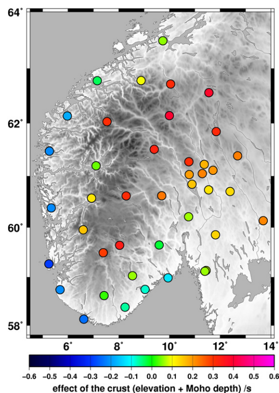
Fig. 3. Crustal travel time correction terms for an average teleseismic shear wave slowness of 7 \text{ s}^\circ . The correction time is relative to the iasp91 reference Earth model (Kennett and Engdahl, 1991) and includes station elevation (Weidle et al., 2010) and Moho topography (Stratford et al., 2009) effects on the travel time.
