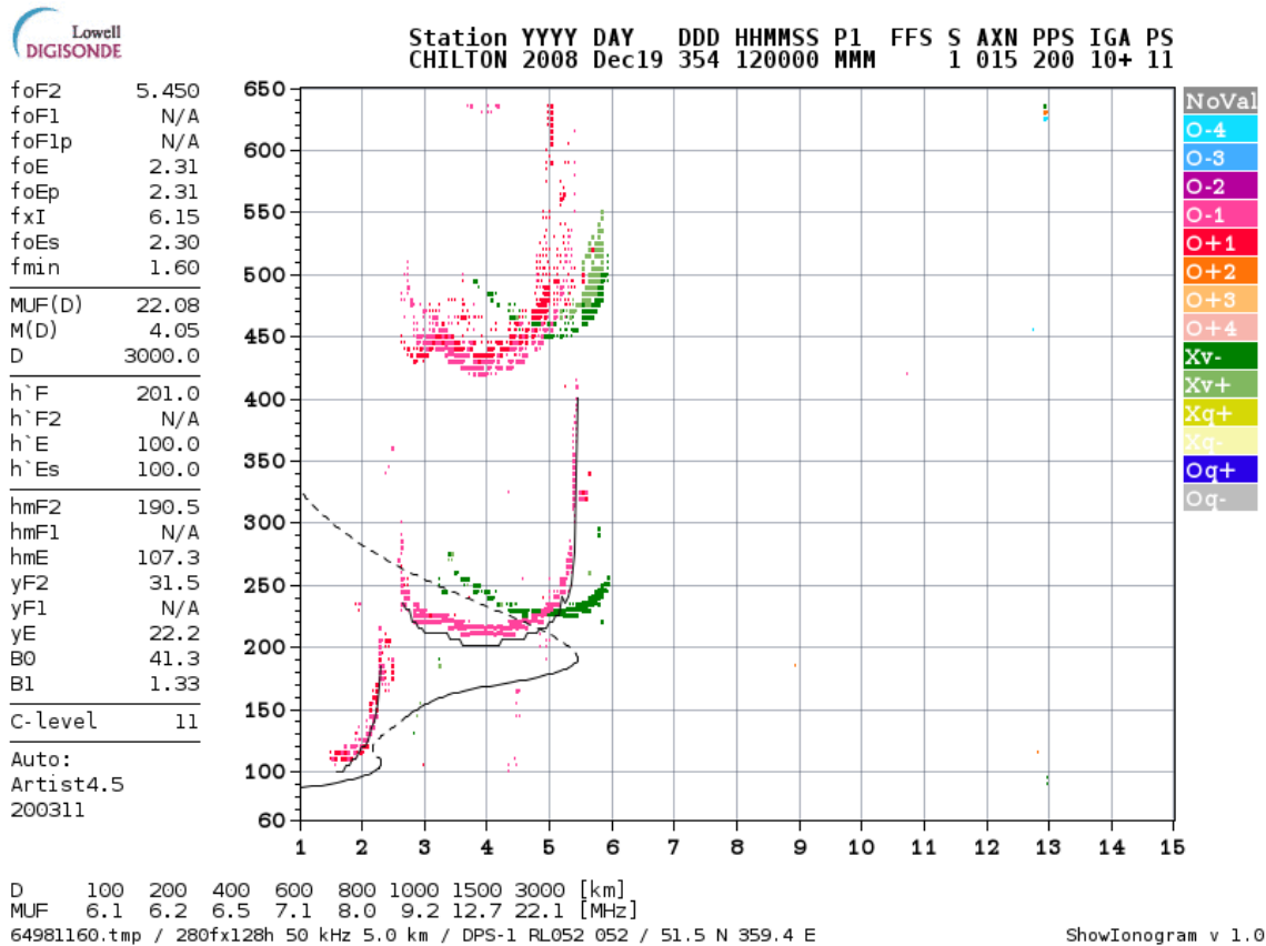
Figure 7.17: Ionogram measured at Chilton at December 19, 2008 at noon and inverted vertical profile of plasma frequency over the station (black line). Source: http://car.uml.edu/common/DIDBDayStationStatistic?ursiCode=RL052&year=2008&month=12&day=19
