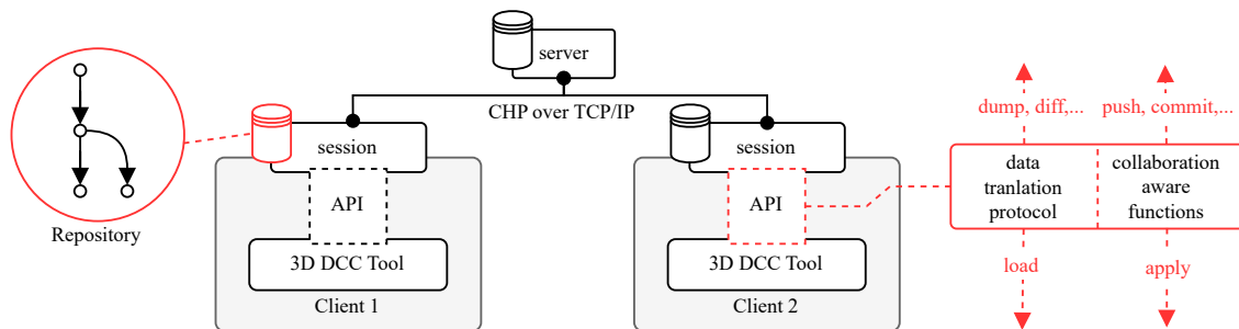
FIGURE II.1.1 – Architecture globale du framework
