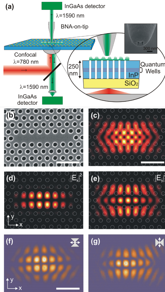
Figure 1.3. (a) Schematic of the experiment. (b) SEM image of the PC nanocavity. (c-e) FDTD simulations of the structure's fundamental mode at \lambda = 1590 \text{ nm} : (c) total electric intensity distribution, (d) intensity of the X electric field component ( |E_x|^2 ), (e) intensity of the Y electric field component ( |E_y|^2 ). (f and g) Near-field images of the PC laser nanocavity collected by the BNA-on-tip. The orientation axis of the BNA is (f) parallel and (g) perpendicular to the long cavity axis (see Figure inset). (scale bars: 1590 nm).
