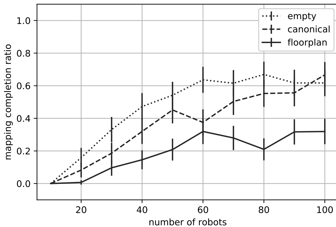
Figure 4.3: Completion ratio of Ramaititima: the portion of runs where the robots map out the entire area.
