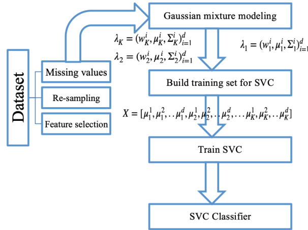
FIGURE 4.3 – Algorithm description
