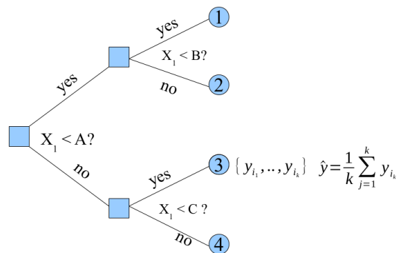
FIGURE 3.2 – Regression tree
