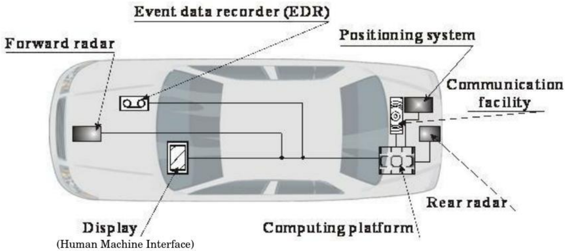
FIGURE 2.7 – A smart vehicle [4]
