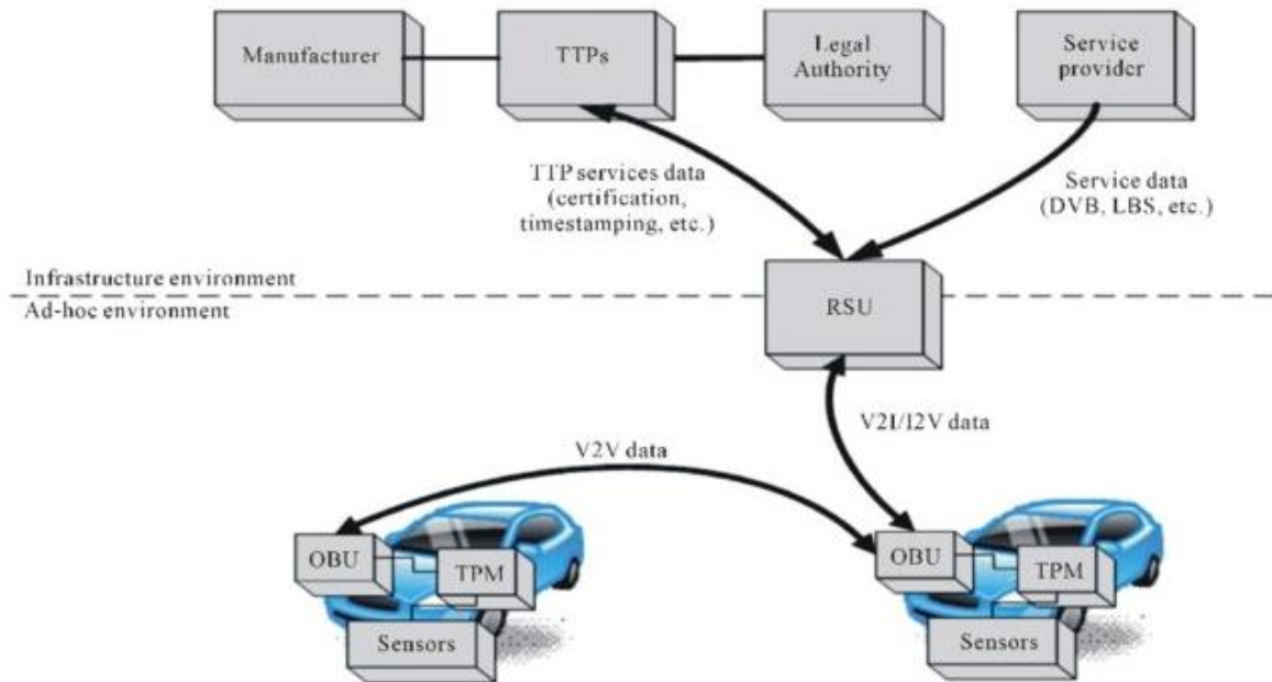
FIGURE 2.6 – VANET units and entities [3]
