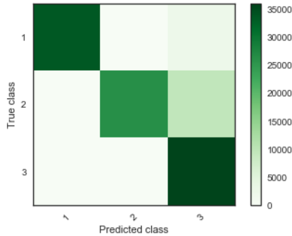
FIGURE 4.10 – Confusion matrix for accident dataset
