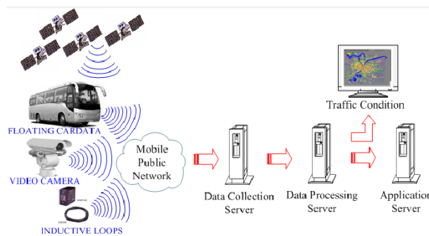
FIGURE 4.1 – Traffic-data-acquisition -using-different-detectors
