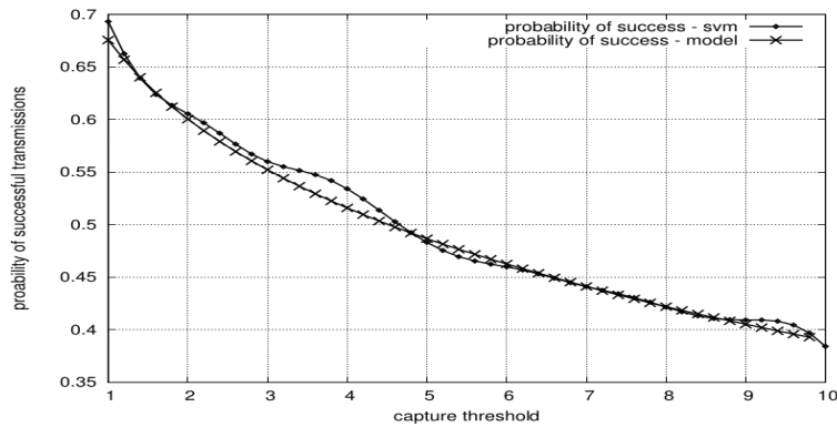
FIGURE 3.10 – Probability of successful reception versus T with error in the database ( x=75m , \mu = 10 , \beta = 4 ).
