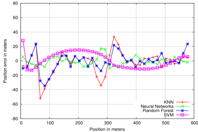
FIGURE 3.5 – Position errors versus position x \in [0, 600m] on the roads with the different machine-learning techniques \sigma = 0.05 . No training data available in [30m, 105m]
