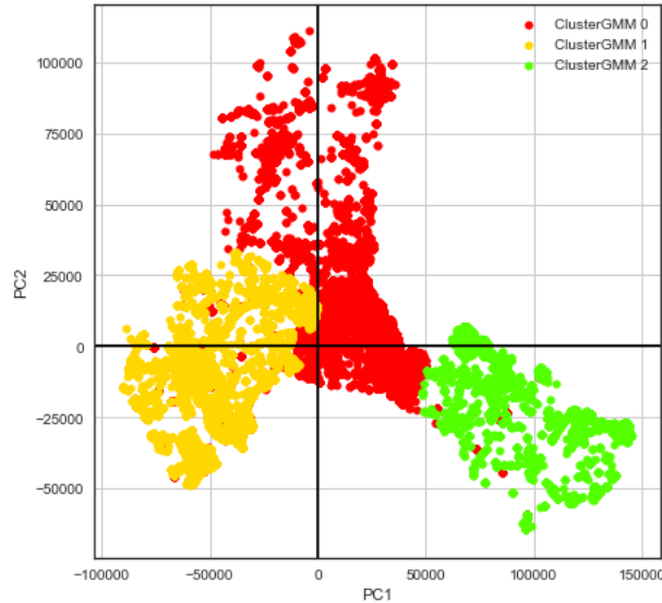
FIGURE 4.9 – Gaussian mixture modelling results
