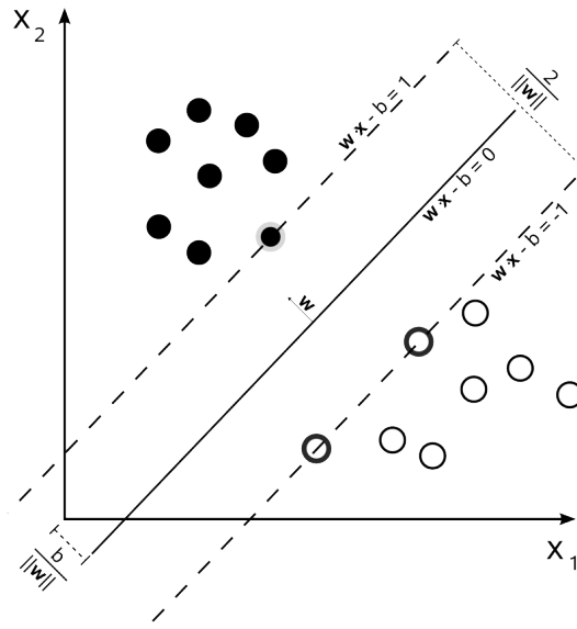
FIGURE 4.6 – Concept of optimal hyper-plane
