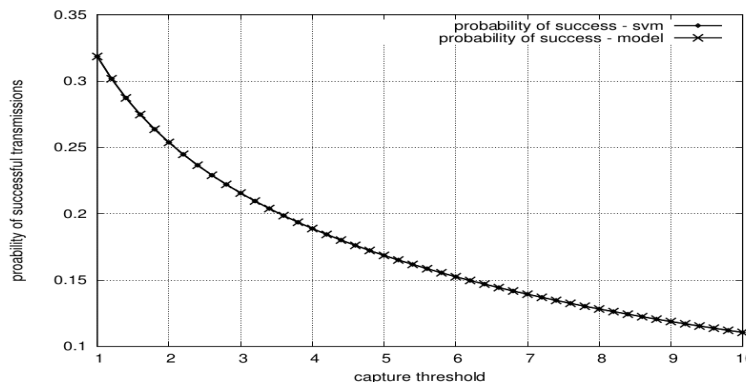
FIGURE 3.9 – Probability of successful reception versus T ( x = 125m , \mu = 10 , \beta = 4 ).
