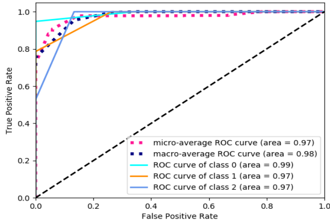
FIGURE 4.11 – ROC curve for the accident dataset
