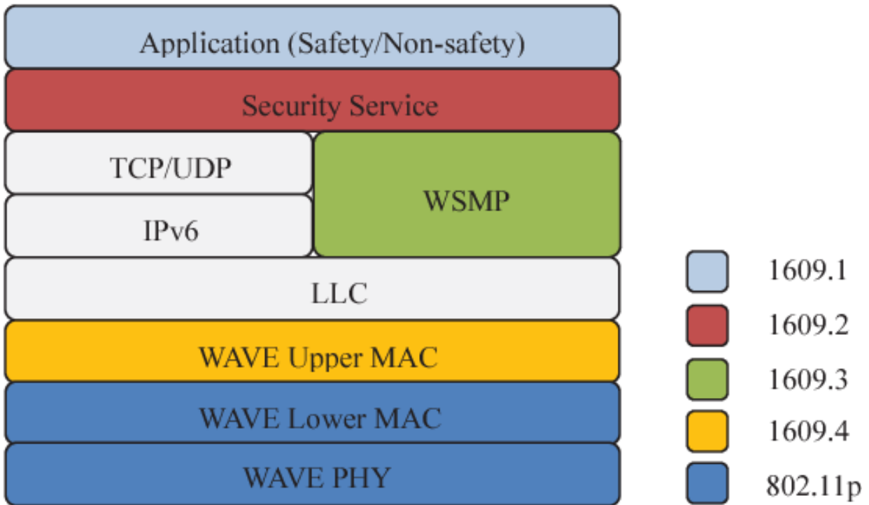
FIGURE 2.10 – IEEE 802.11p DSRC-WAVE Protocol stack[2]
