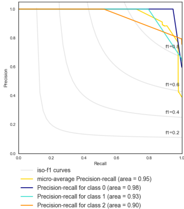
FIGURE 4.13 – AUC-PR curves for each class on various ISO-F1 curves for the accident dataset
