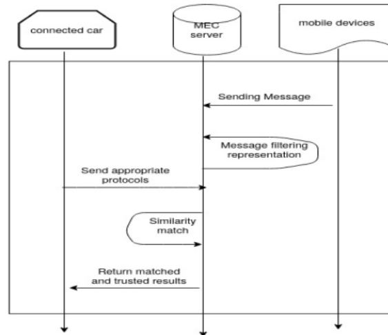
FIGURE 5.3 – Mobile Edge Entity Search Process
