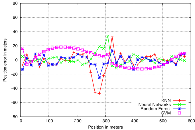
FIGURE 3.4 – Position errors versus position x \in [0, 600m] on the roads with the different machine-learning techniques \sigma = 0.05 . Training data measurements available only every 30m
