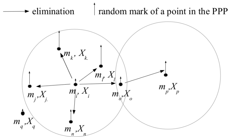
FIGURE 3.7 – Matern CSMA selection process and an example of over-elimination.
