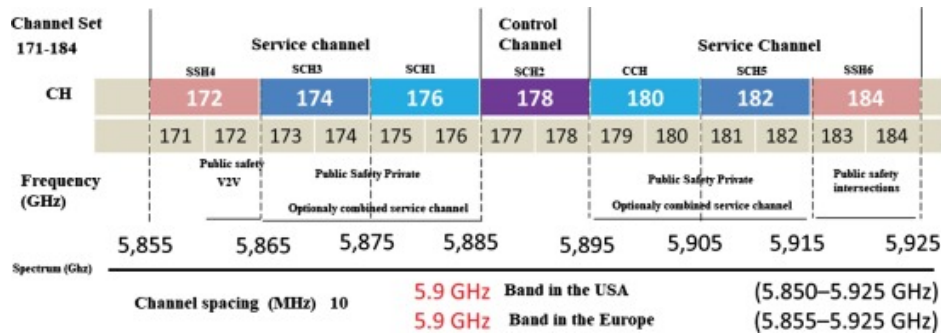
FIGURE 2.9 – DSRC frequency spectrum [2]
