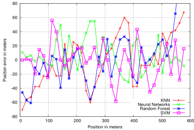
FIGURE 3.6 – Position errors versus position x \in [0, 600m] on the roads with the different machine-learning techniques with Rayleigh fading .
