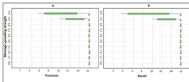
FIGURE 5.8 – Precision and recall
