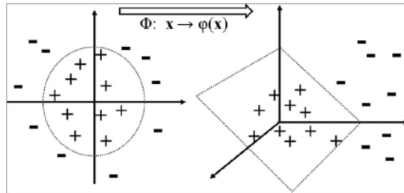
FIGURE 4.7 – Kernel trick
