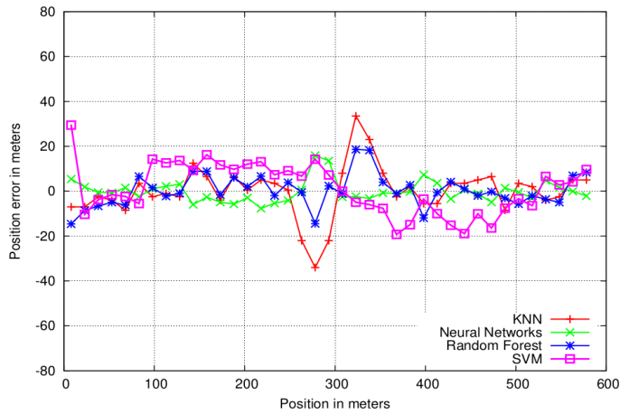
FIGURE 3.3 – Position errors versus position x \in [0, 600m] on the roads with the different machine-learning techniques \sigma = 0.05 .
