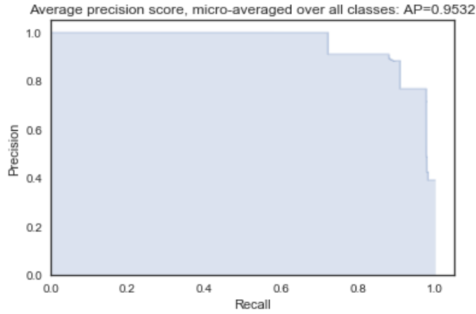
FIGURE 4.12 – AUC-PR curve micro averaged over all classes for the accident dataset
