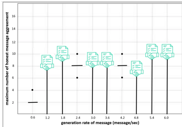
FIGURE 5.7 – Relationship between the block creation rate and the maximum agreement between trusted blocks
