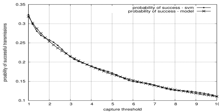
FIGURE 3.11 – Probability of successful reception versus T with error in the database ( x=125m , \mu = 10 , \beta = 4 ).
