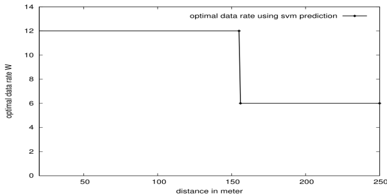
FIGURE 3.12 – Optimal data rate versus distance vehicle-RSU, \mu = 10 , \beta = 4 ).
