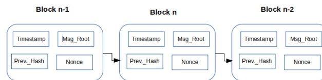
FIGURE 5.2 – The structure of blocks in a blockchain
