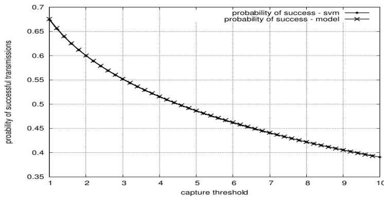
FIGURE 3.8 – Probability of successful reception versus T ( x = 75m , \mu = 10 , \beta = 4 ).
