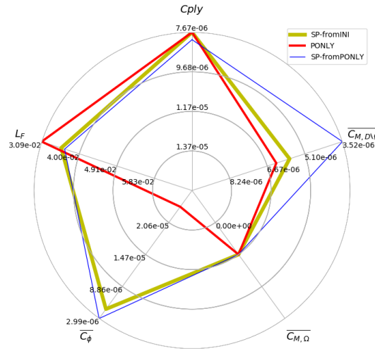
Figure 9.20: Quantitative values visualization, initialization 2, aluminium, large cantilever, V_{tar} = 1.1V_0
