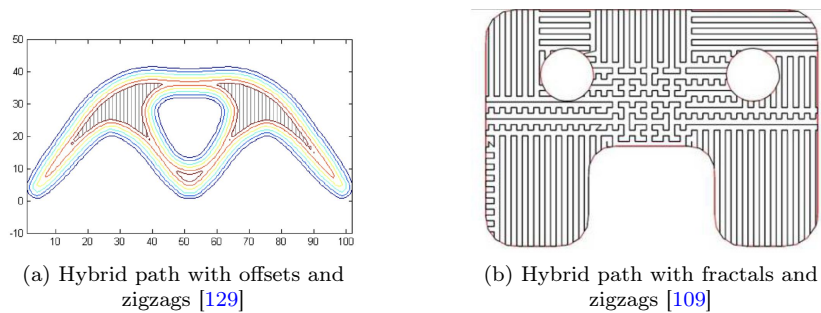
Figure 1.17: Hybrid lines
