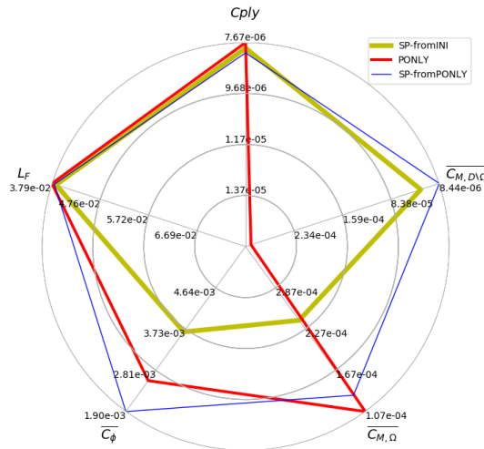
Figure 9.28: Quantitative values visualization, initialization 2, titanium, large cantilever, V_{tar} = 1.1V_0
