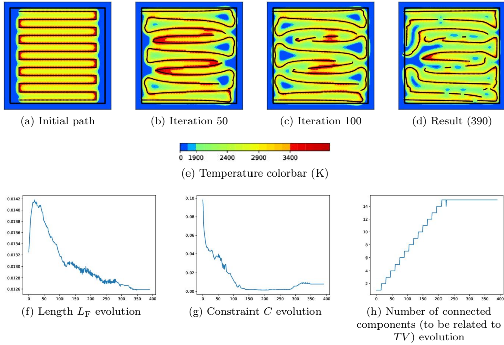
Figure 8.20: Path and temperature as well as length, constraint and number of connected components evolution with respect to iterations, starting from zigzag12-TI (titanium)
