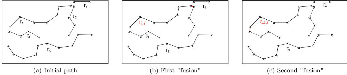
Figure 8.18: Melting algorithm
