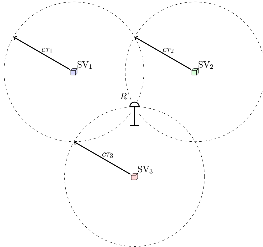
Figure 1.3: General Principle of GNSS.
