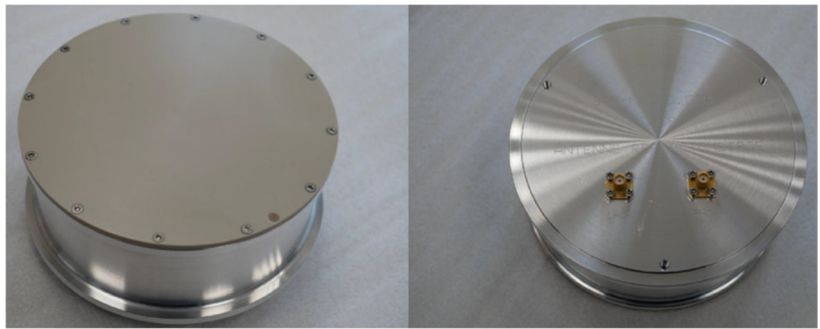
Figure 3.12: CNES dual polarization antenna (credit: CNES).
