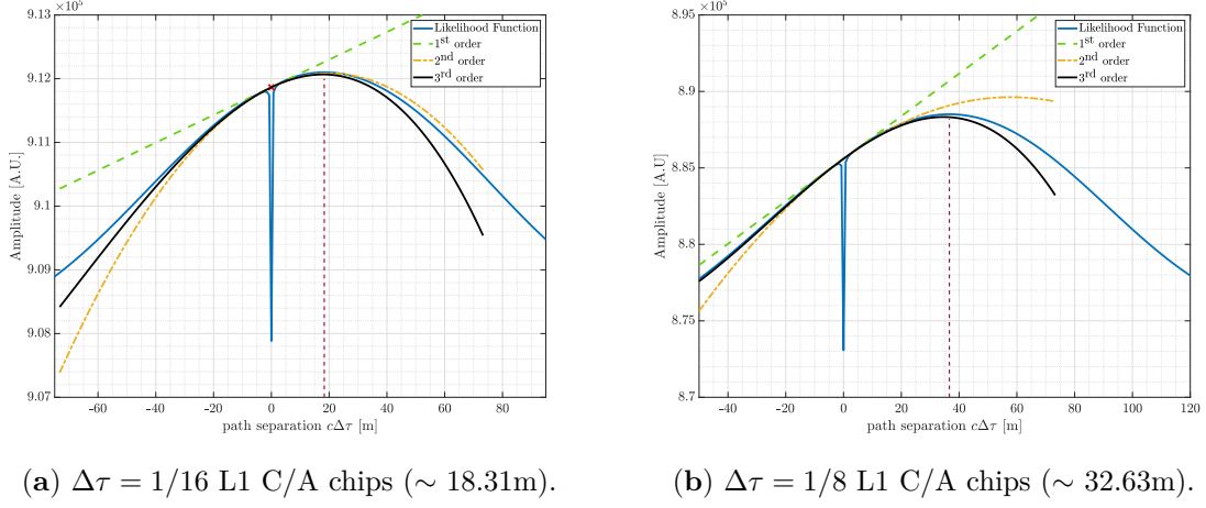
Figure 3.27: Illustration of the likelihood criterion Taylor approximations at different orders and relative delay \Delta\tau .
