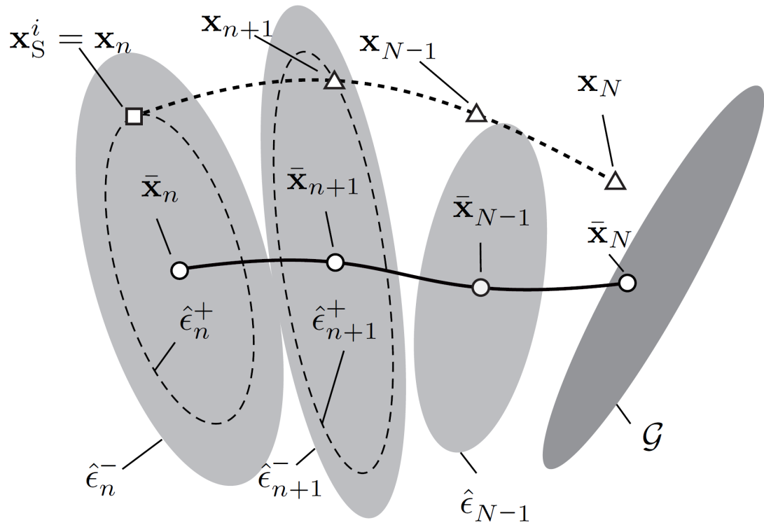
FIGURE 2.6: In this picture is shown how to adjust the funnel hypothesis through simulation as it is proposed in [6]. Each ellipsoid represents a stabilizable ball to the goal with the action defined in each ball without violating the constraints. In this picture is shown that for the state \mathbf{x}_s^i the final goal is not reached. Therefore it means that the funnel hypothesis is wrong and each ball has to be shrunk to integrate this new information from the simulation.
