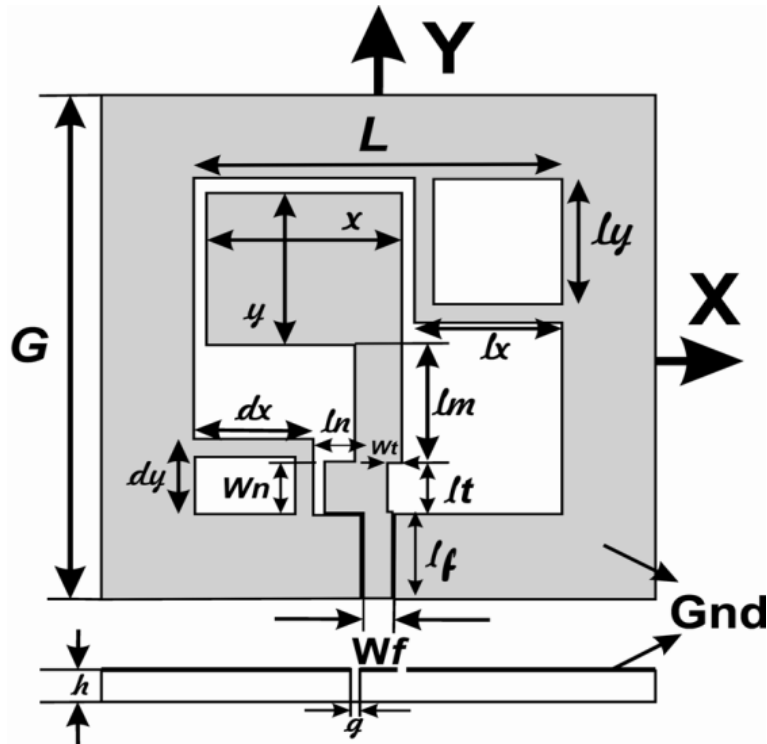
Figure 71 :Geometry of the proposed CP square slot antenna for UWB applications ( G=60 , L=40 , W_f=3 , L_f=10.3 , g=0.3 , h=0.8 , l_x=15.5 , l_y=16.5 , l_n=3.3 , W_n=6 , l_t=6 , W_t=1.5 , l_m=14 , dx=13 , dy=9 , x=21 , y=18 ) (Unit : mm).
