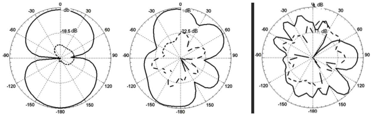
Figure 16: E plane radiation pattern diagram for an elliptical monopole antenna structure with A_2=48 mm and B=52 mm at frequencies (a) 1, (b) 6 and (c) 10GHz (From left to right, respectively.) [30-33]
