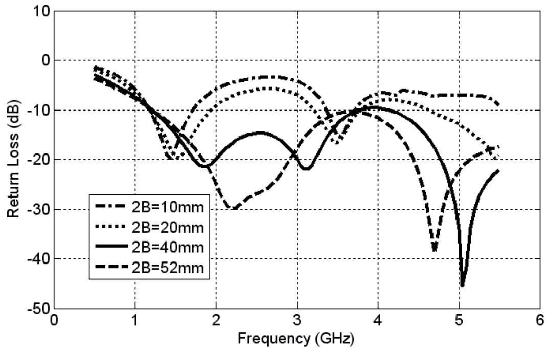
Figure 13: Return loss diagram for four elliptical monopole antennas with A_2 = 48 mm and B_2 variable [30-33].
