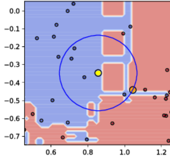
Figure 4.4: Illustrative result of the Local Risk Assessment procedure (left: S_x = 1 ) for an instance of the half-moons dataset, commented in Section 4.2.3.
