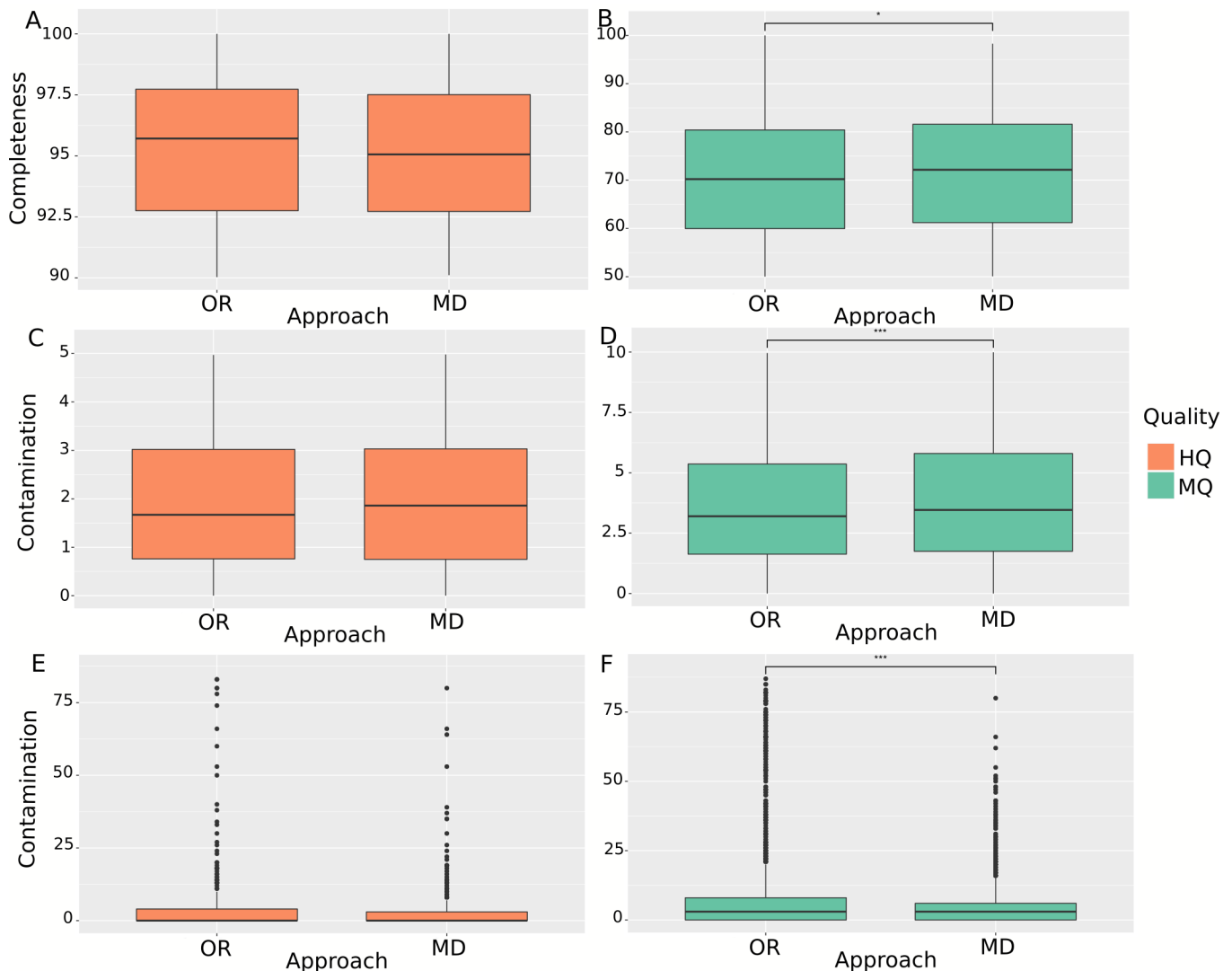
Figure 4.8 Quality of reconstructed MAGs from the Tara Ocean metagenomes. Comparison of the oceanic regions (OR) approach against the metagenomic distance approach (MD). HQ = High Quality, MQ = Medium Quality. (A) Completeness estimated for HQ MAGs; (B) Completeness estimated for MQ MAGs; (C) Contamination measured using SCGs for HQ MAGs; (D) Contamination measured using SCGs for MQ MAGs; (E) Contamination measured using all genes detected in the sequences of HQ MAGs; (F) Contamination measured using all genes detected in the sequences of MQ MAGs.
