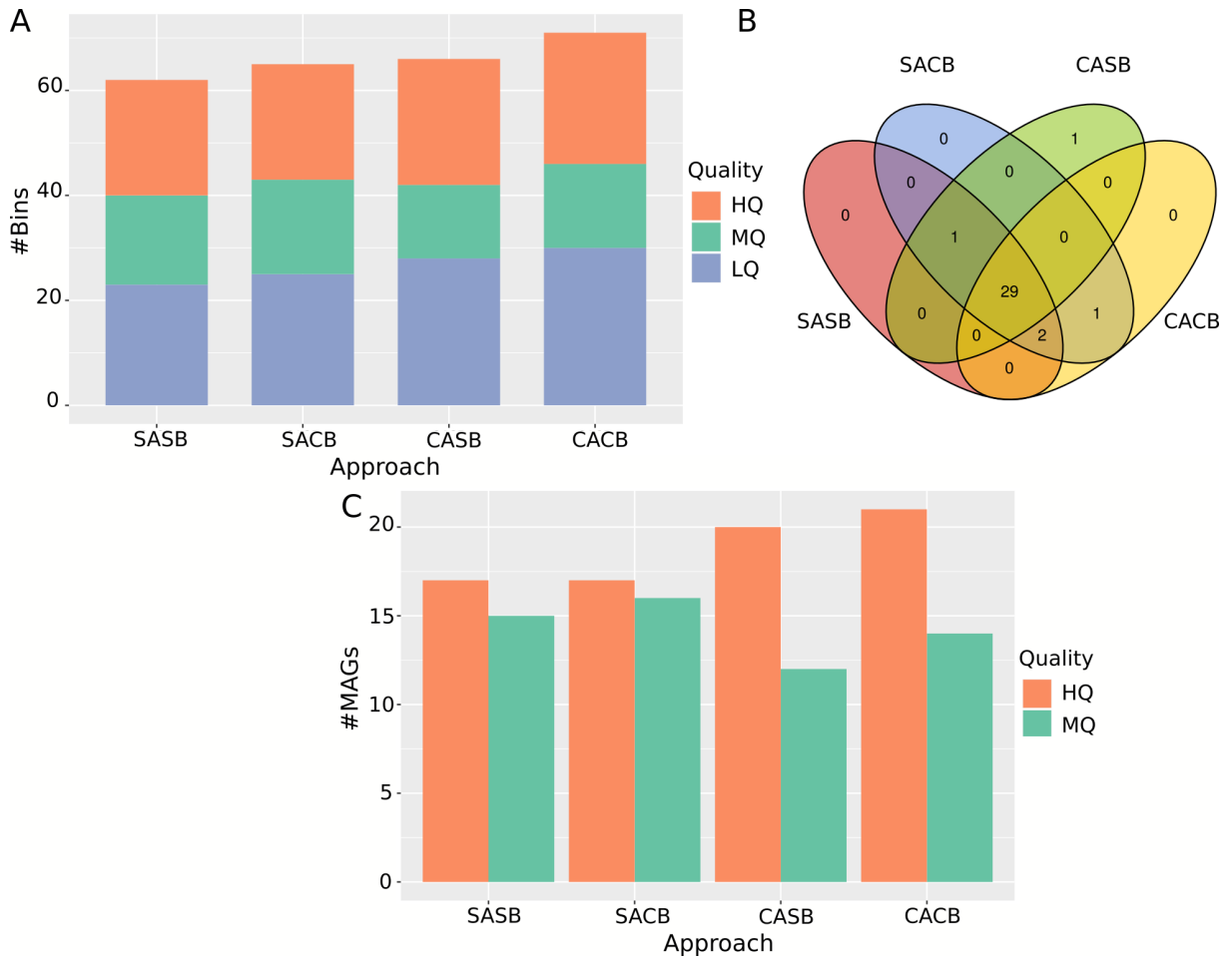
Figure 4.11 Evaluating assembly-binning strategies on simulated metagenomes. (A) Total number of bins obtained after the binning step. Colours represent quality of genome bins estimated using CheckM: High Quality (HQ), Medium Quality (MQ), and Low Quality (LQ). (B) Number of source genomes found in each strategy. Each number represents the number of times a MAG from a strategy maps against a source genome. Intersections represent common genomes between strategies. (C) Number of de-replicated MAGs obtained, after independent de-replication by dRep for each strategy. As the genomes are all represented with one single strain, de-replication at both species or strain resolution gives the same number of de-replicated genomes, so only one de-replication resolution is shown.
