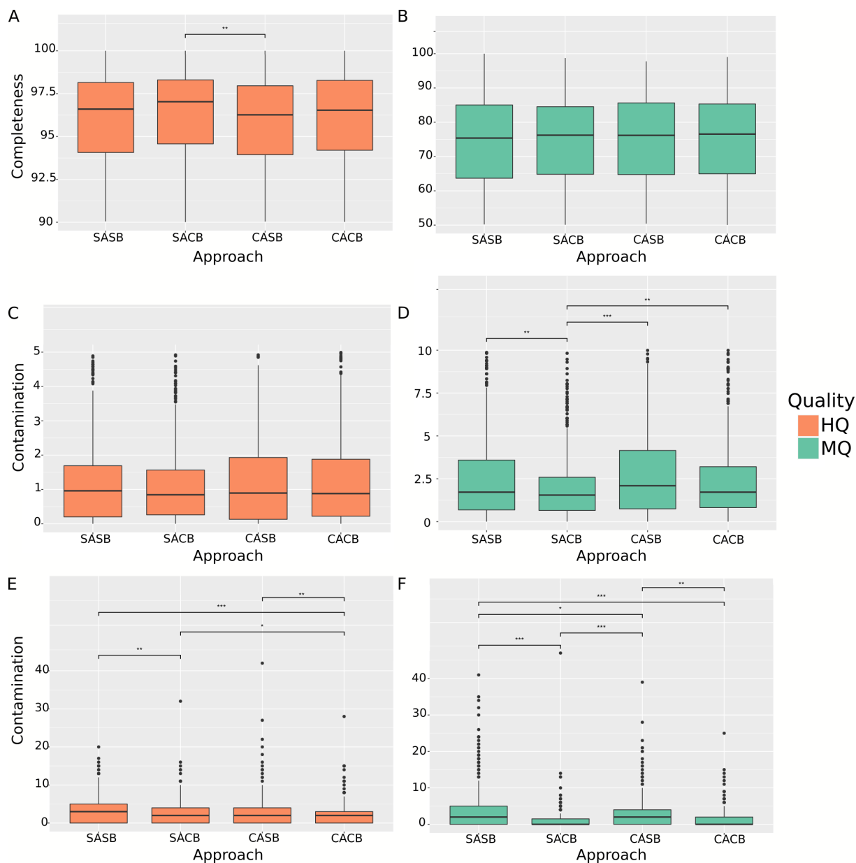
Figure 4.15 Quality of reconstructed MAGs from the HMP dataset.
