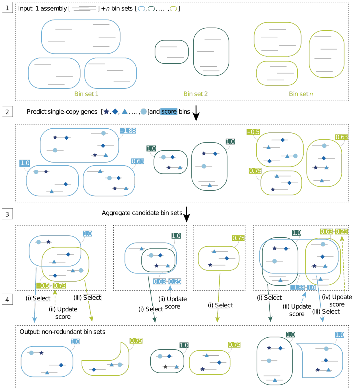
Figure 2.6 Overview of the DAS Tool algorithm.
