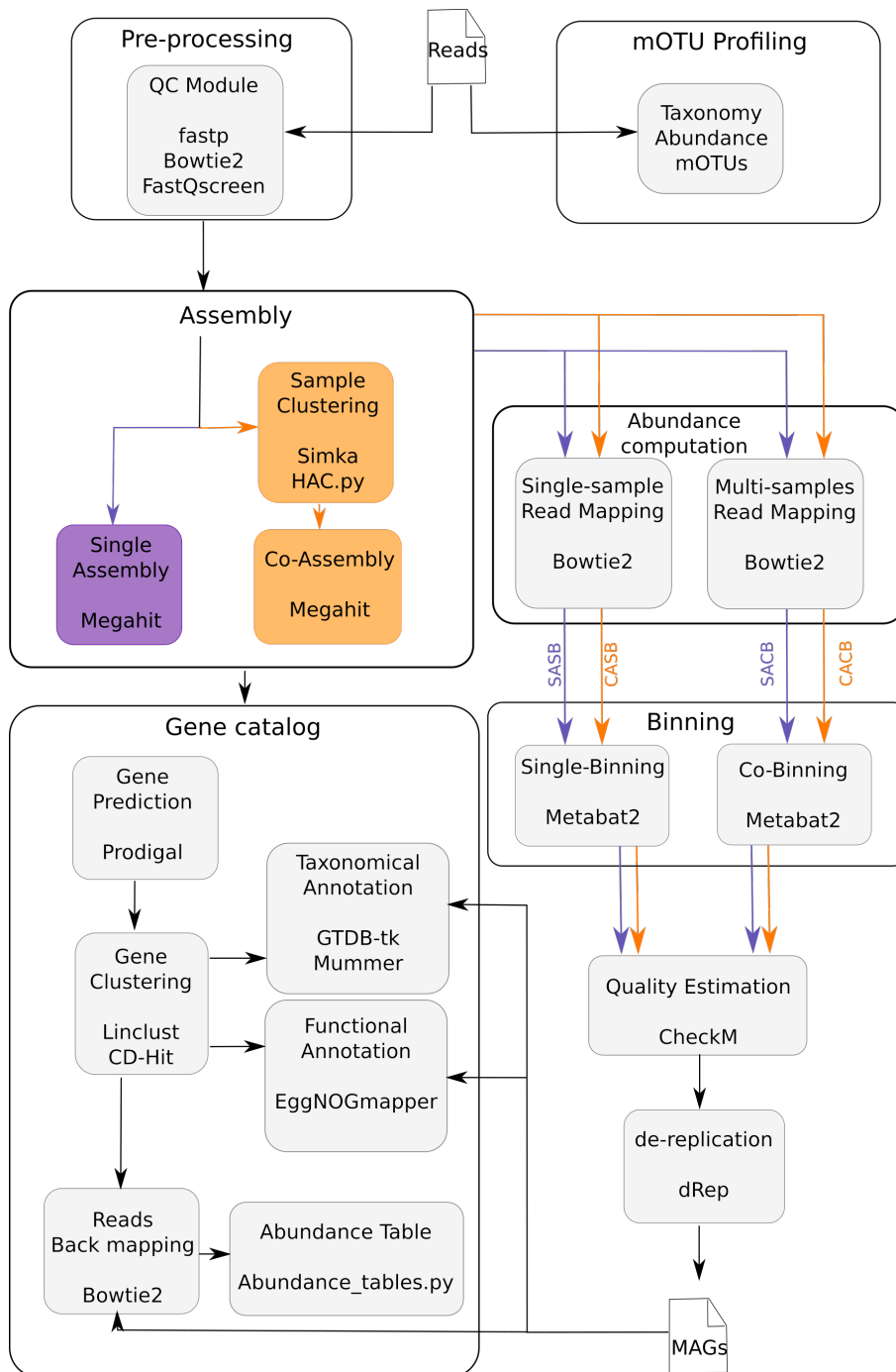
Figure 4.1 Overview of the MAGNETO workflow.
