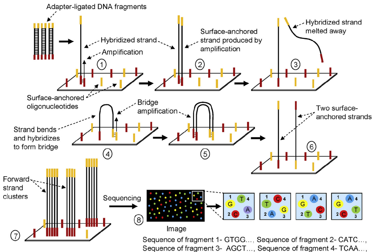
Figure 1.2 Illumina sequencing.
