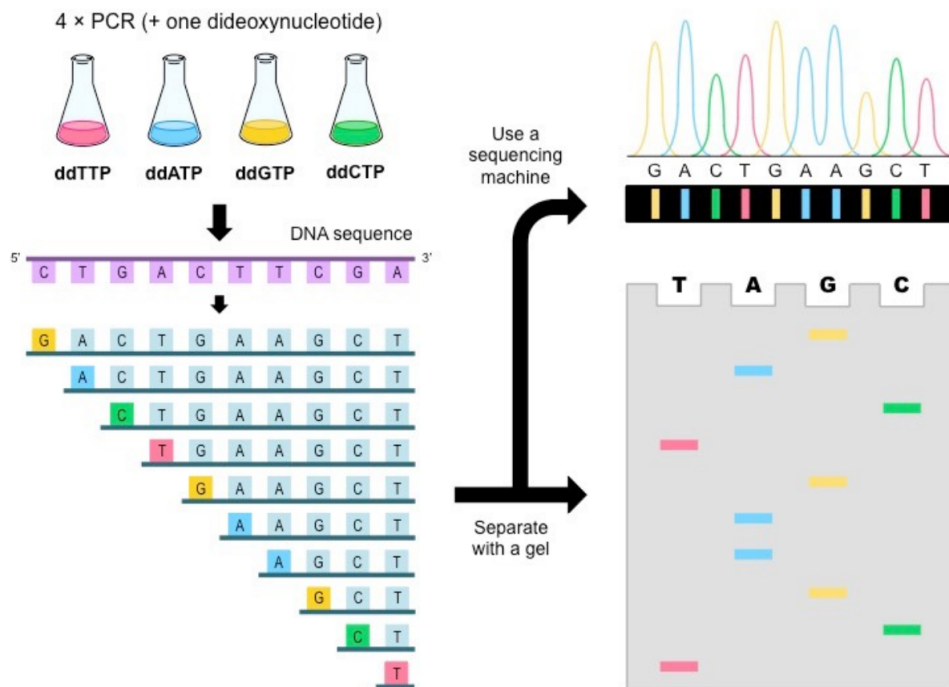
Figure 1.1 Sanger sequencing method.
