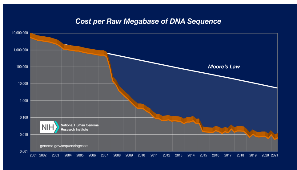
Figure 1.3 Sequencing cost per raw Mb.
