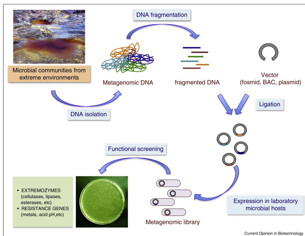
Figure 1.5 Preparation of a library for functional metagenomics.
