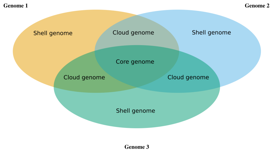
Figure 1.4 Pan-genome and its components.
