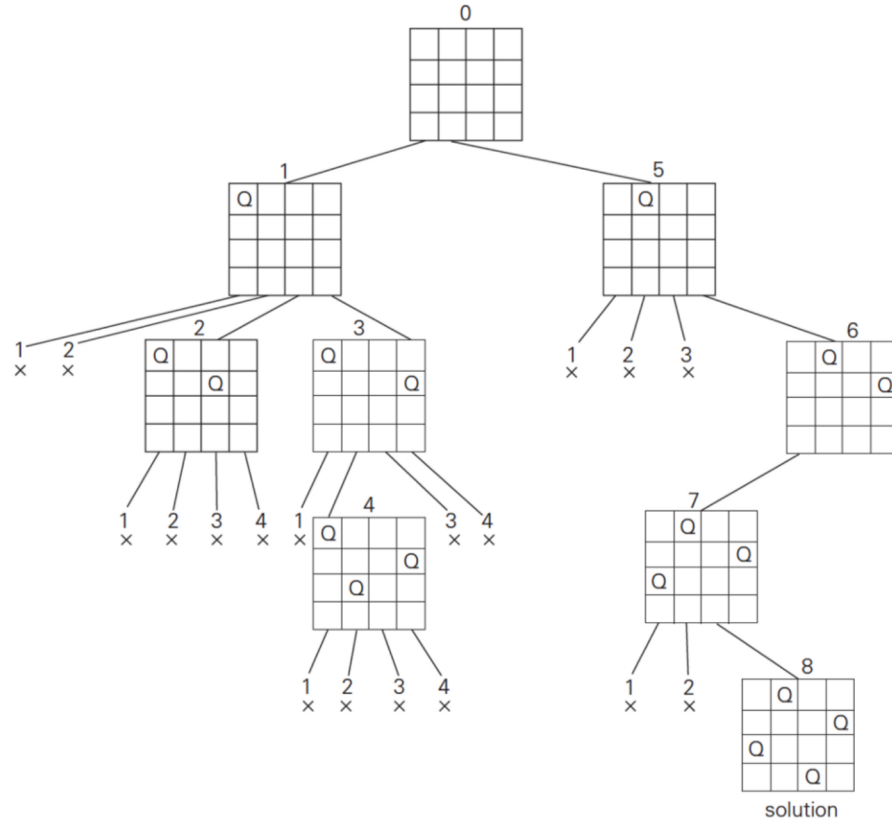
Figure 3.1 Backtracking in the 4-queens problem.
