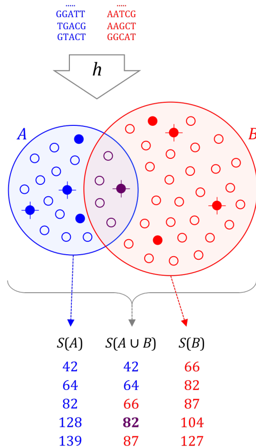
Figure 2.5 Overview of the MinHash sketch strategy for estimating contigs similarity in Mash.
