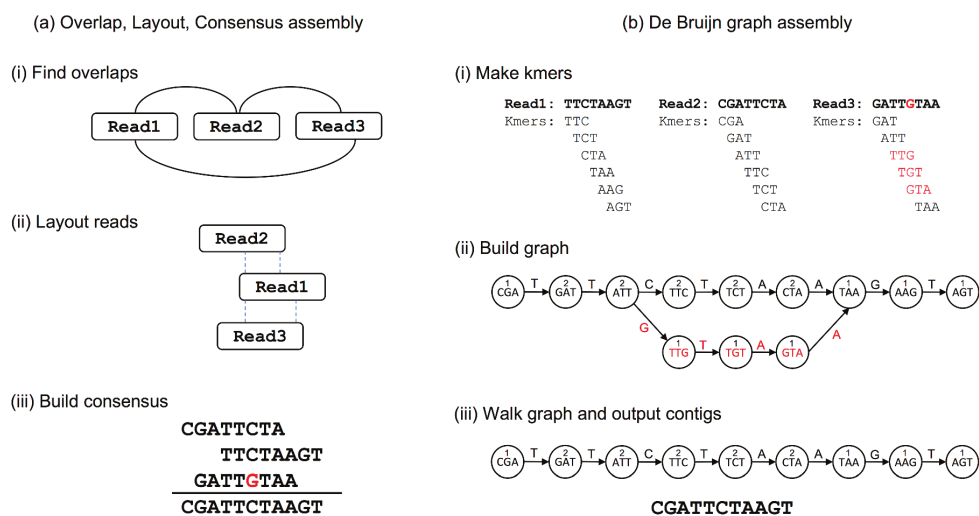
Figure 2.1 A schematic representation of an assembly graph.
