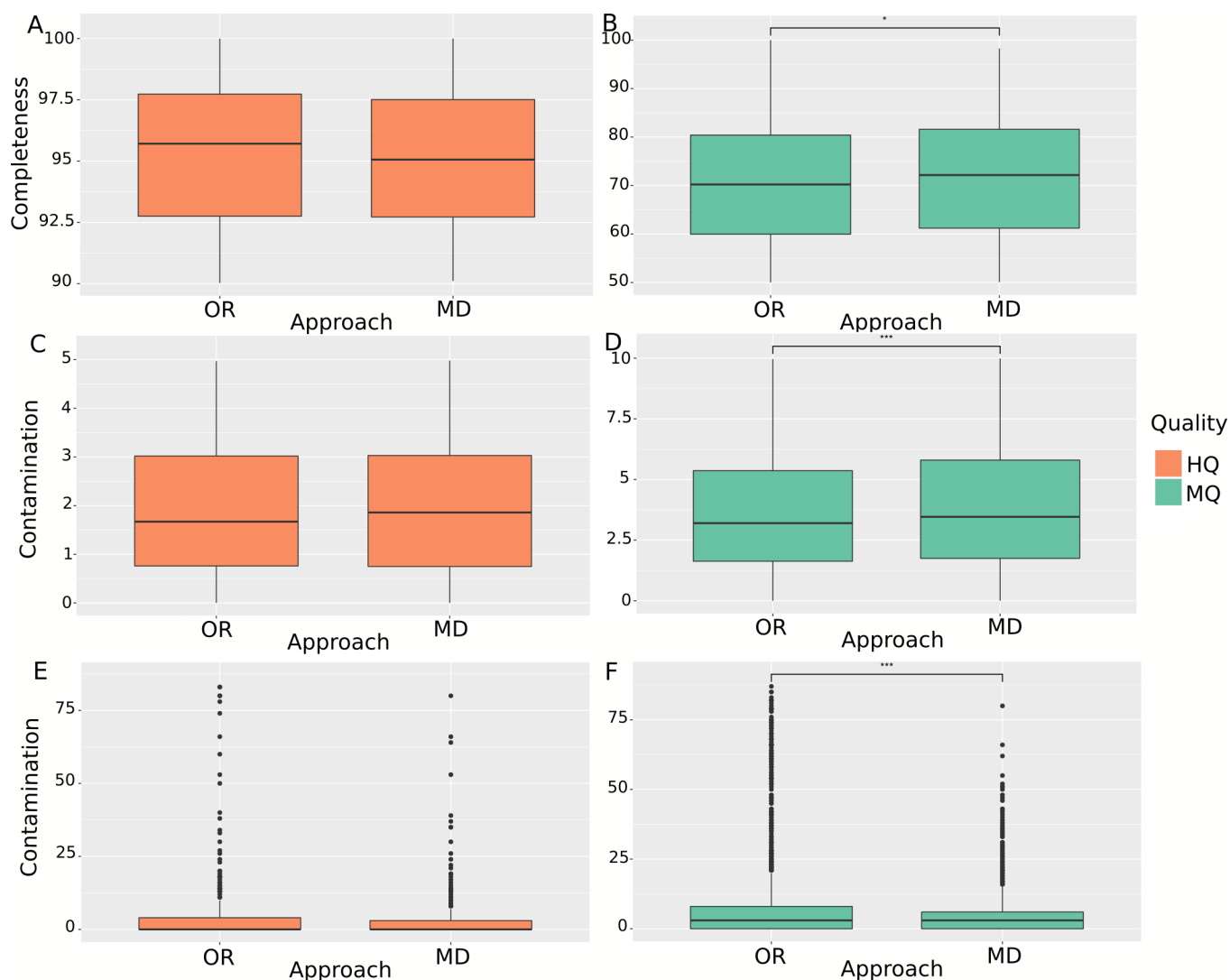
Figure 4.8 Quality of reconstructed MAGs from the Tara Ocean metagenomes.
