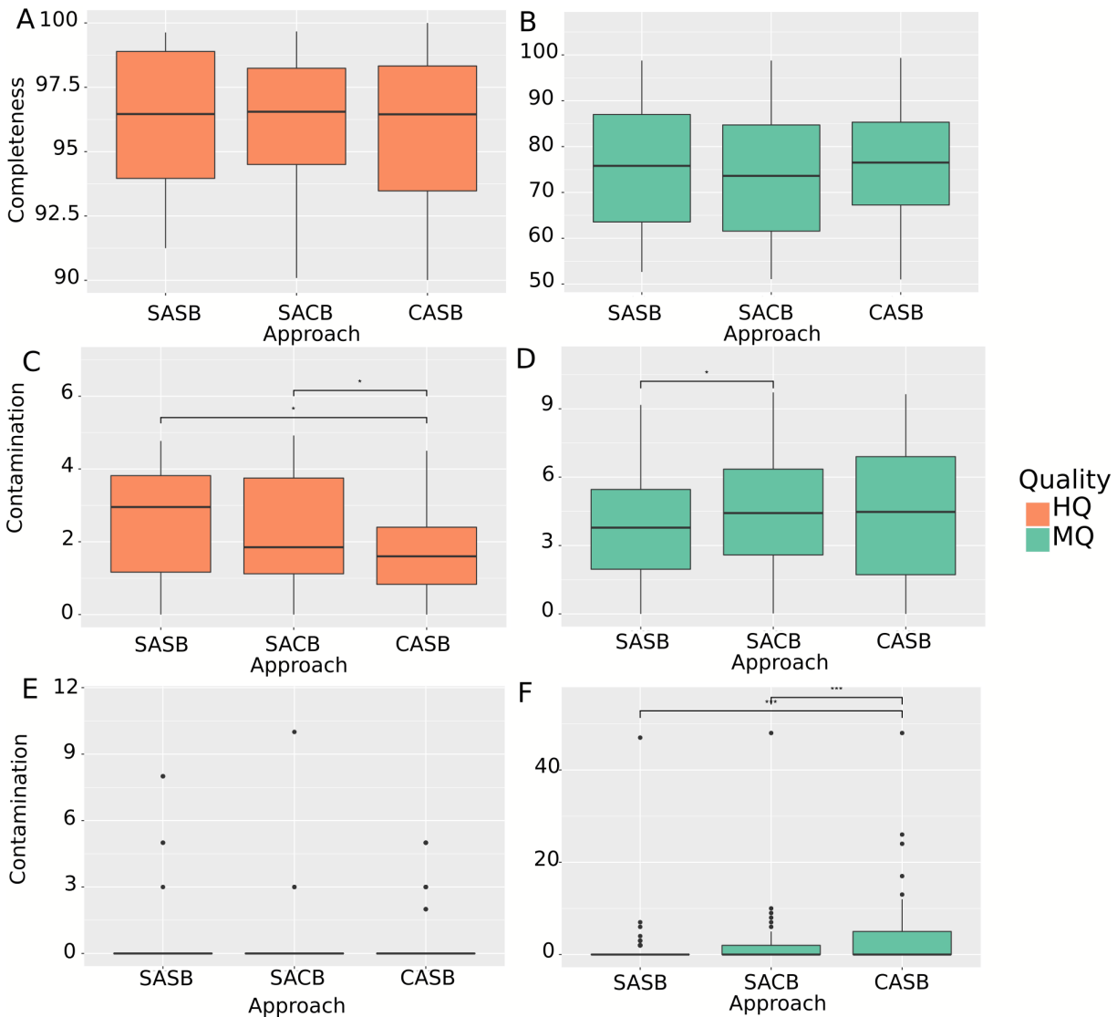
Figure 4.12 Quality of reconstructed MAGs from the CAMI dataset.
