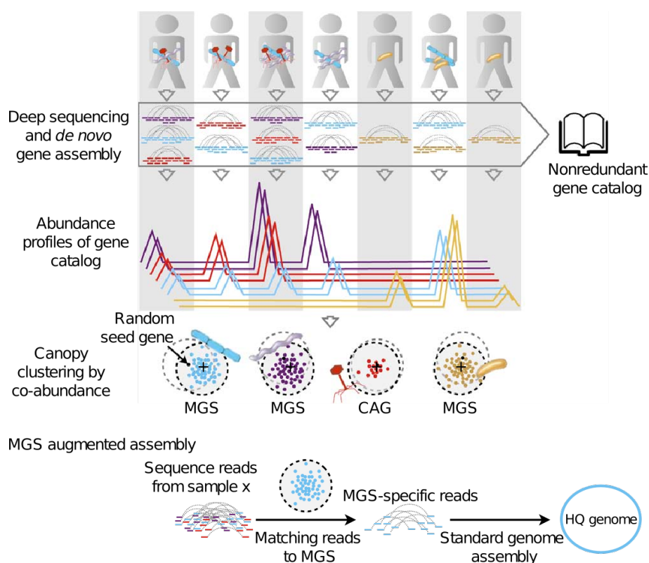
Figure 2.7 Canopy clustering algorithm.
