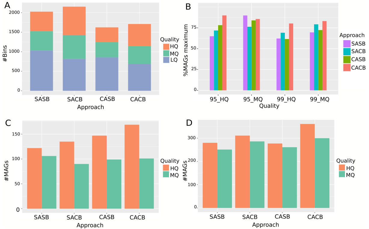
Figure 4.14 Evaluating the binning strategies on the HMP dataset.
