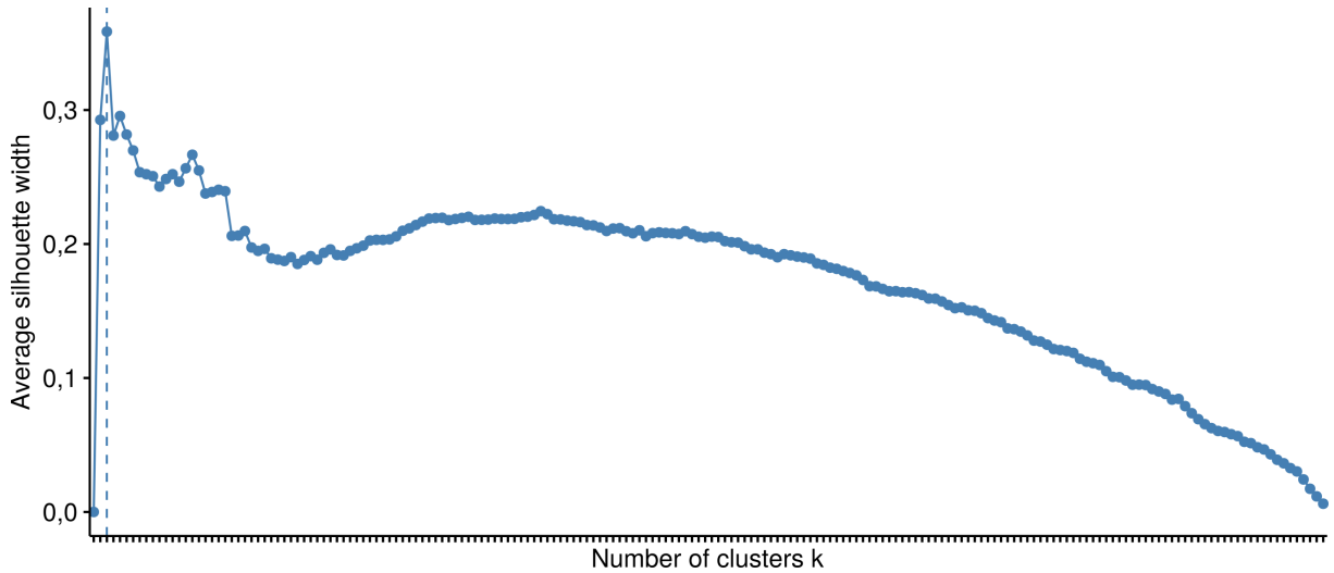
Figure 4.3 Evaluation of the partition of the whole Tara metagenomes dataset.
