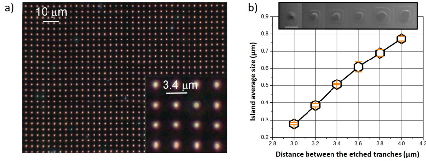
Figure 5.2: a) Optical dark-field image of a typical array of organized dewetted Si islands. The inset shows the homogeneity of the islands obtained with a periodicity of 3.4 \mu\text{m} . b) Average island size as a function between the etching pitch as obtained by scanning electron micrographs (SEM). The error bar represents the standard deviation. The line is a guide for the eyes. The top inset show a typical SEM for each etched pitch.
