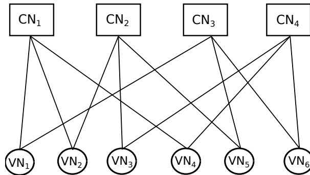
Figure 4.7: Tanner graph representation of the parity check matrix \mathbf{H} . The check-nodes CN_j are represented by squares, and The variable-nodes VN_i are represented by circles.
