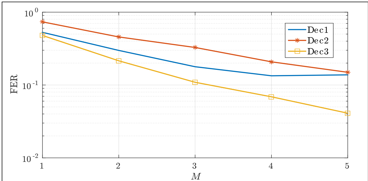
Figure 5.12: FER with respect to the number of sequences M , over the memory channel model trained onto SetE .
