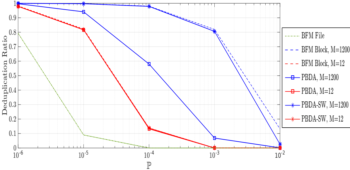
Figure 6.6: Data deduplication ratio as a function of \mathbb{P} for the four different algorithms. For the PD and SW-PD, we consider L_p = 6 , L_s = 94 (i.e., M = 1200 ), and L_p = 6 , L_s = 9994 (i.e., M = 12 ).
