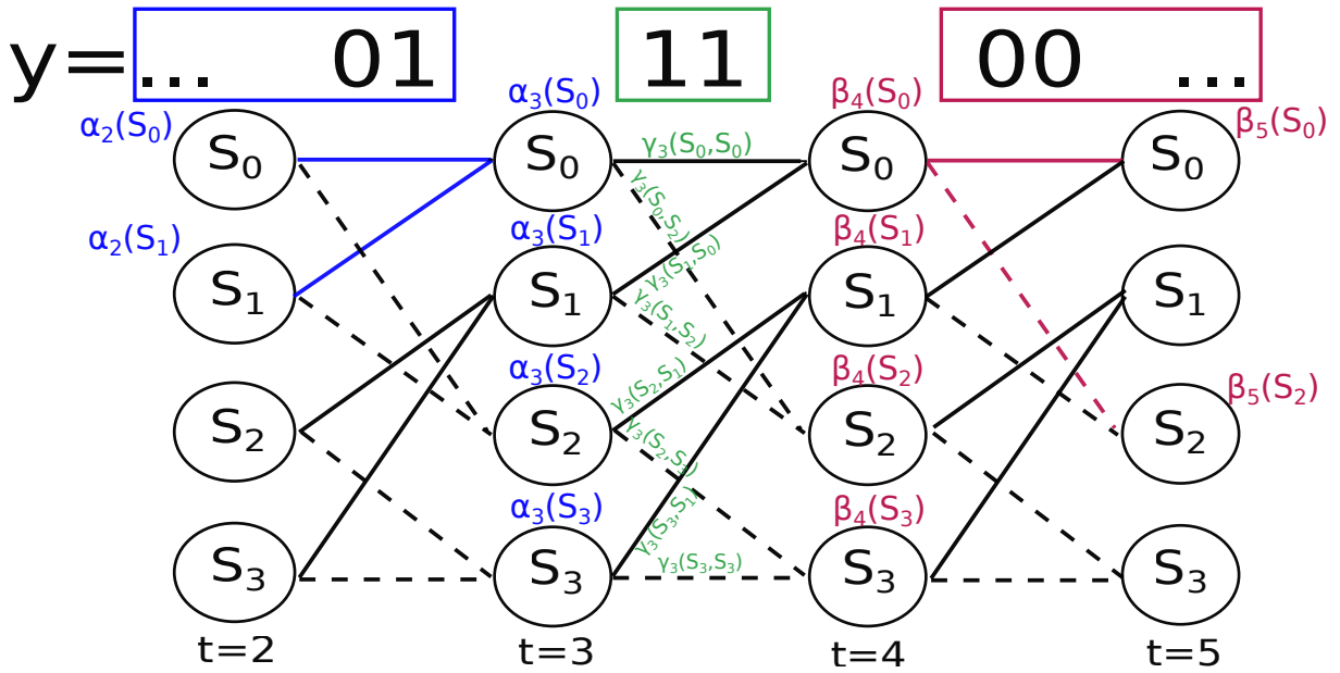
Figure 5.5: BCJR algorithm example on a partial trellis diagram, for time instants t \in [2, 5] .
