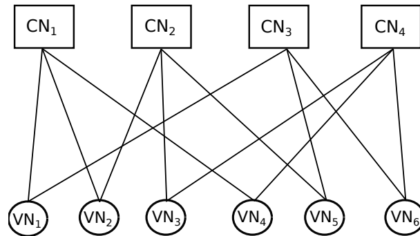
Figure 4.7: Tanner graph representation of the parity check matrix \mathbf{H} . The check-nodes CN_j are represented by squares, and The variable-nodes VN_i are represented by circles.
