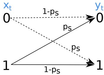
(a) Binary Symmetric Channel.
