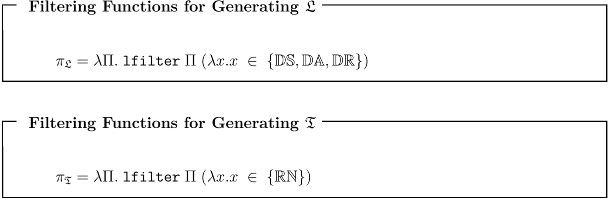
Figure 5.34: Filtering functions on \Pi , where lfilter is the classic filter function on lists in functional programming.
