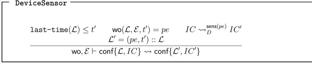
Figure 5.15: The DeviceSensor rule. A sensor, or a group of sensors detects a physical event.
