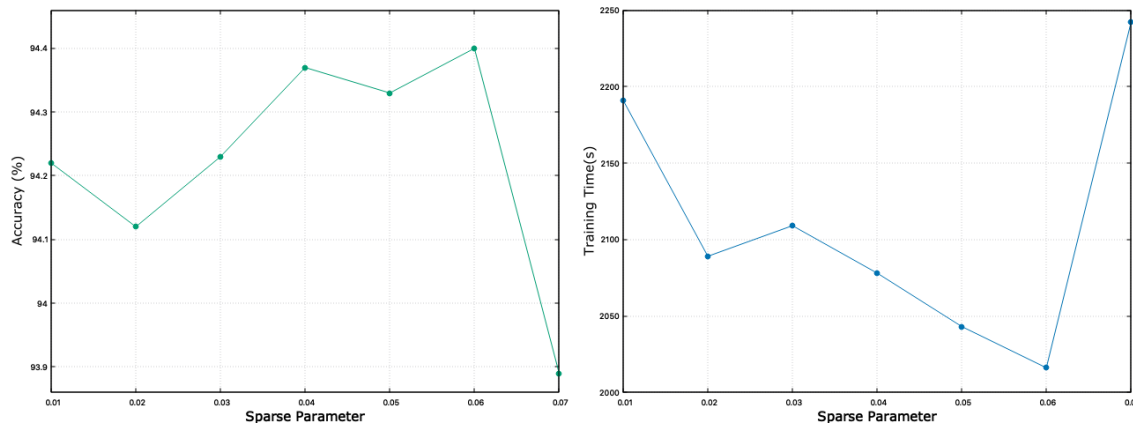
Figure 5.4: Accuracy and training time of different sparse parameter
