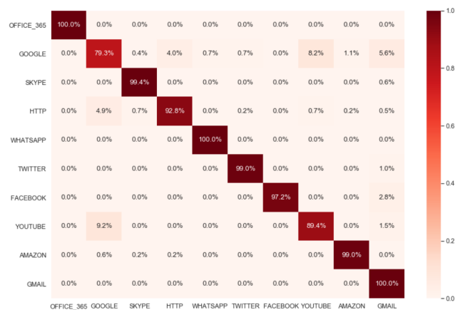
(b) Confusion matrix for Autoencoder
