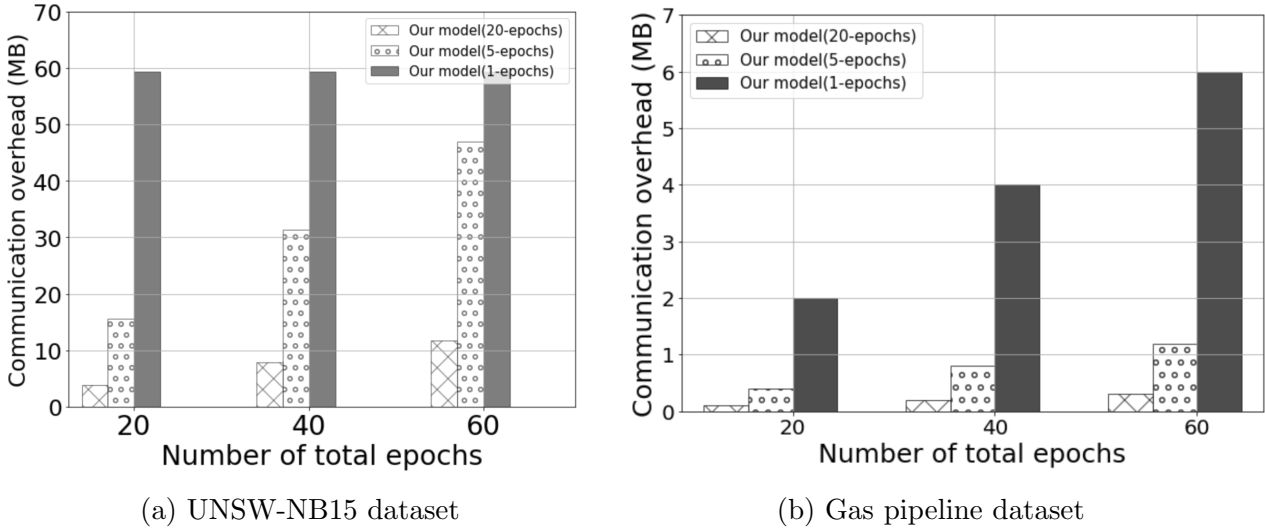
Figure 6.4: Comparison in terms of communication overhead for two datasets
