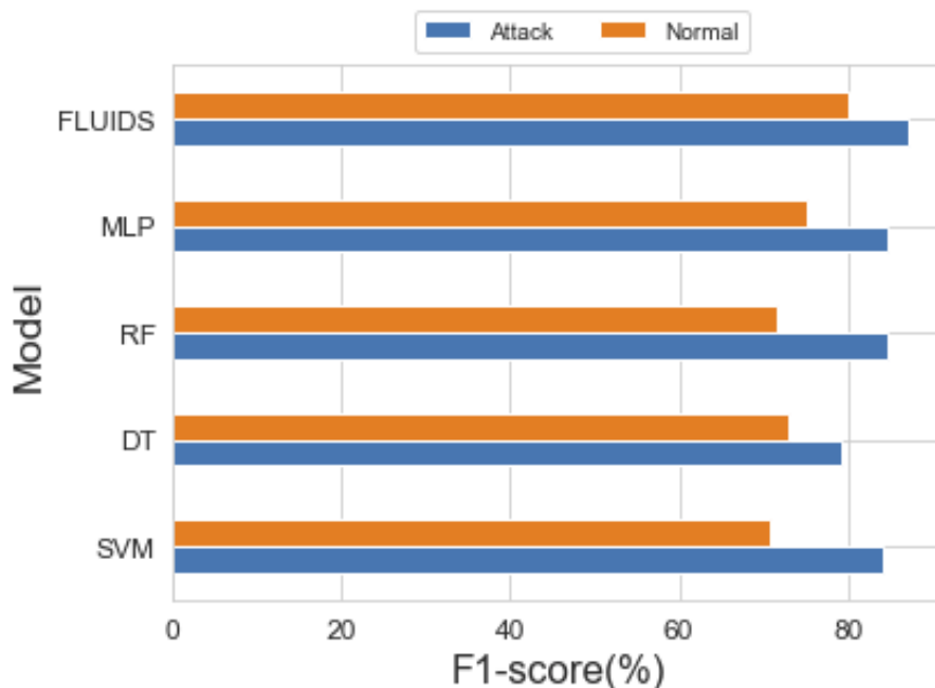
Figure 6.5: The performance of identifying normal and attack flows of FLUIDS against supervised models using the UNSW-NB15 dataset.
