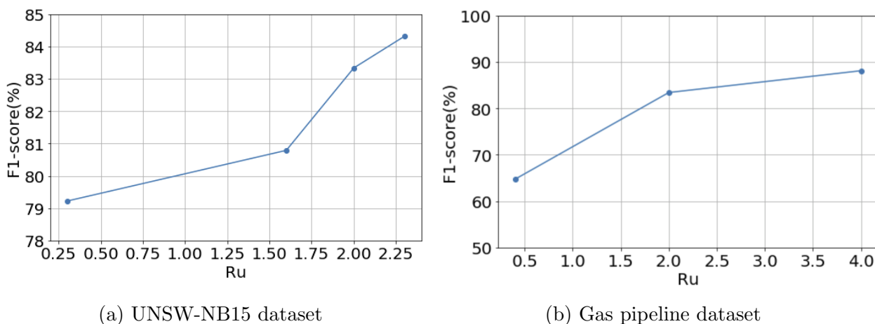
Figure 6.3: F1-score with various unlabeled ratio ( R_u ).
