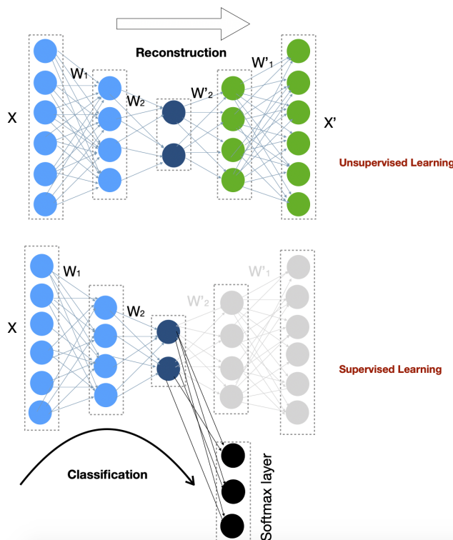
Figure 5.8: Classification process with AE model
