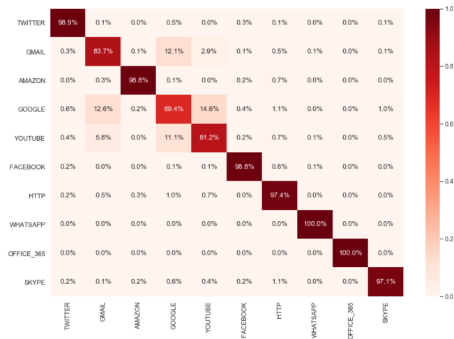
(c) Confusion matrix for XGBoost
