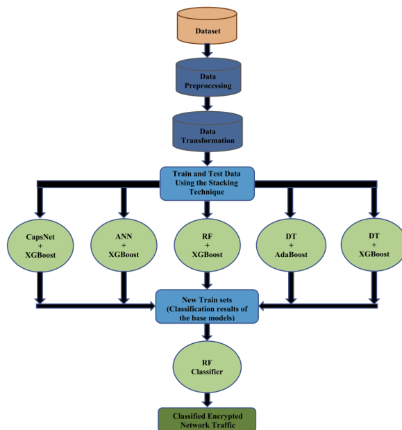
Figure 3.2: Training process of CARD-B [104]
