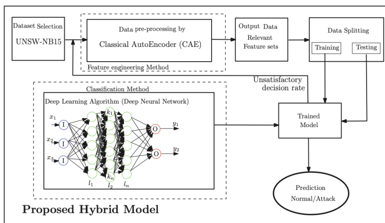
Figure 3.5: Training process of the hybrid anomaly detection method [126]
