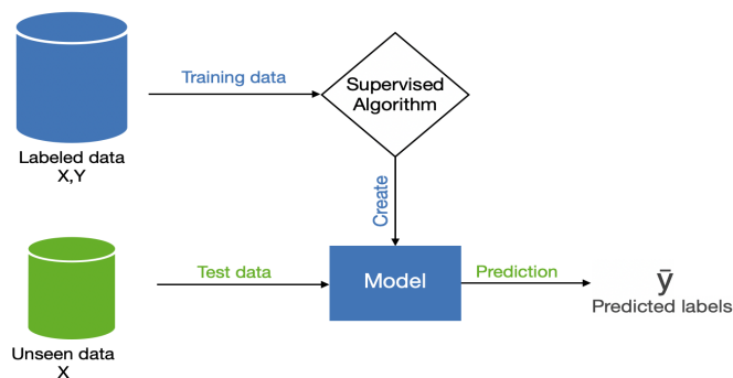
Figure 2.2: Training process of supervised learning algorithm
