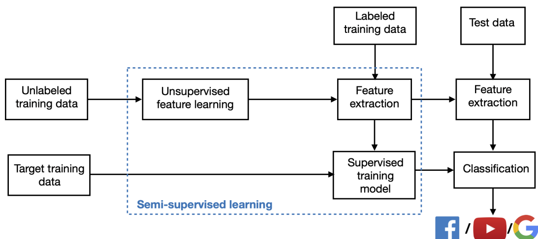
Figure 5.1: Structure of the semi-supervised network traffic classification model
