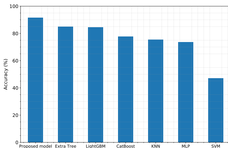
Figure 4.4: Comprehensive comparison of well-known classifiers against the proposed blending model.
