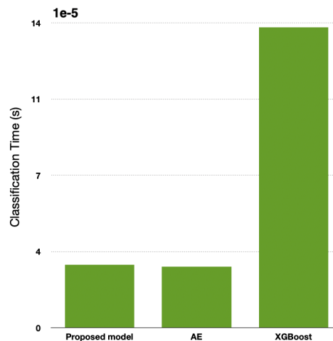
Figure 5.11: Classification time comparison per sample
