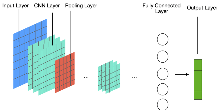
Figure 2.12: CNN (Convolution Neural Networks)
