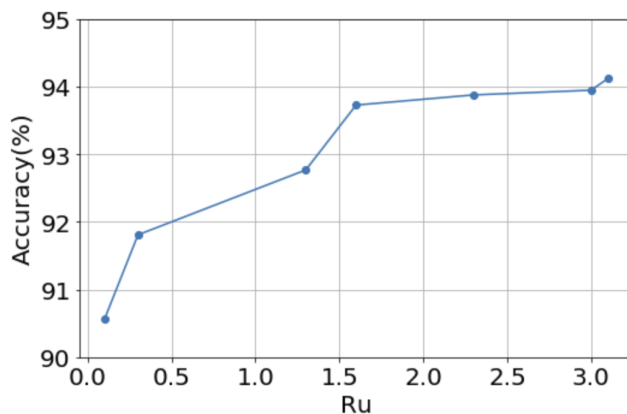
Figure 5.3: Performance of model with different unlabeled ratios.
