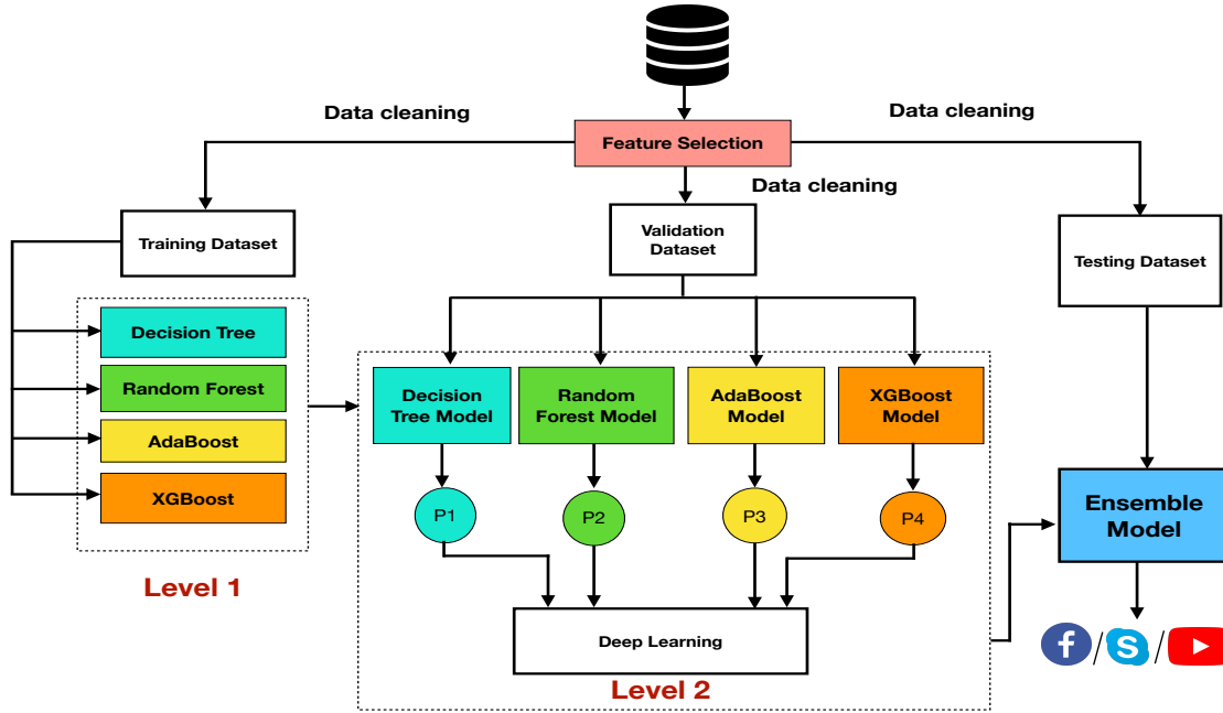
Figure 4.1: Flowchart for the proposed blending ensemble model
