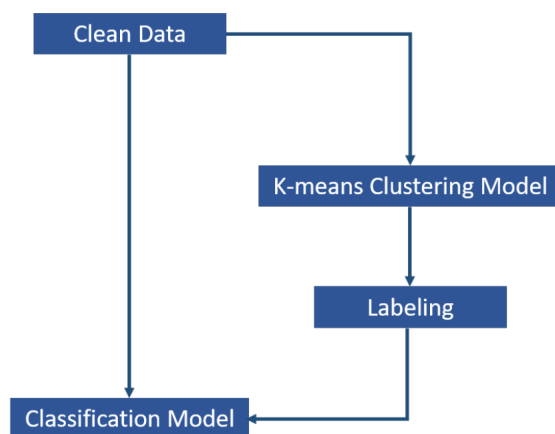
Figure 3.3: Training process of the semi-supervised model [29]
