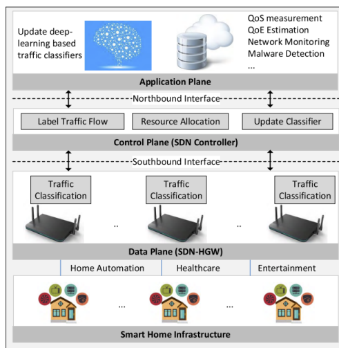
Figure 3.4: Overview of the SDN-HGW framework [113].
