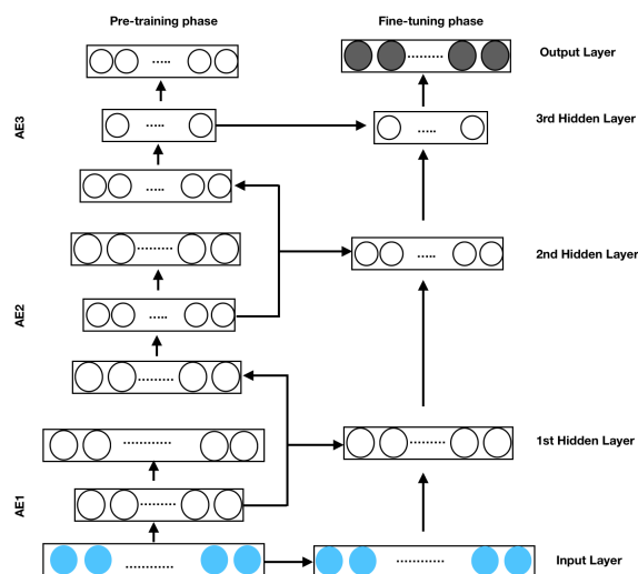
Figure 5.2: General Stacked Autoencoder process
