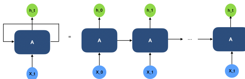
Figure 2.13: RNN (Recurrent Neural Networks)
