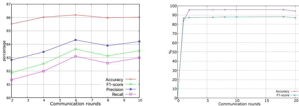
(a) UNSW-NB15 dataset
