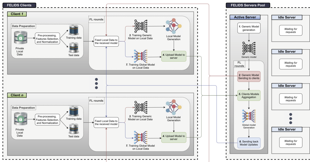
Figure 3.6: FLIDS architecture [139]
