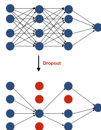
Figure 2.18: Dropout technique
