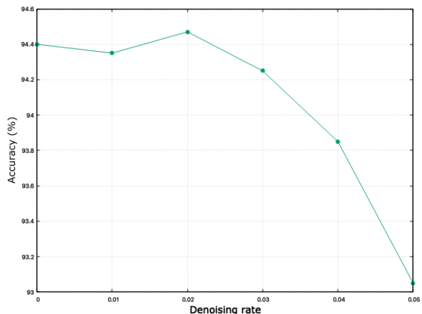
Figure 5.6: Effect of denoising coding
