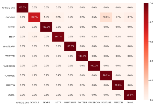
(a) Confusion matrix for the proposed model
