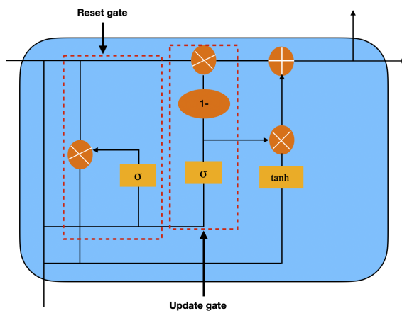
Figure 2.15: GRU (Gated Recurrent Unit)
