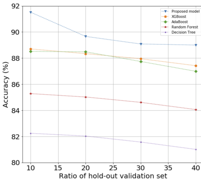
Figure 4.2: Effect of hold-out validation set ratio on the proposed blending model.
