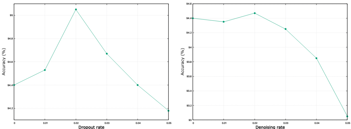
Figure 5.5: Effect of dropout
