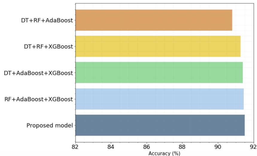
Figure 4.3: Results of the different combinations of the base classifier experiments and their impact on the proposed blending model.
