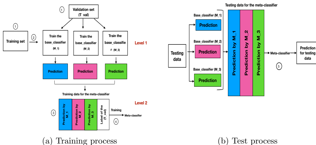
Figure 2.6: Blending ensemble process
