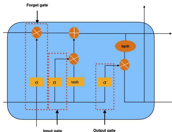
Figure 2.14: LSTM (Long Short-Term Memory)
