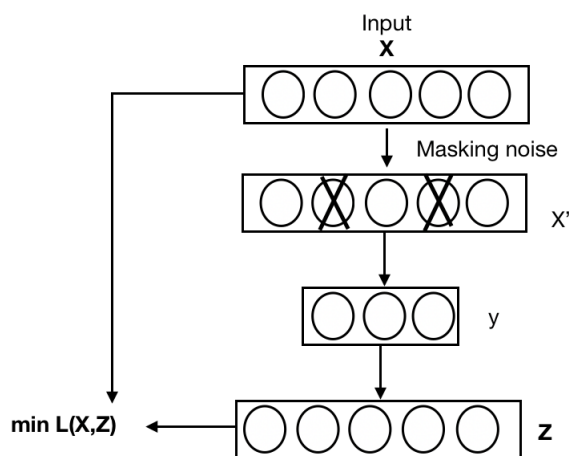
Figure 2.17: Training process of individual denoising autoencoders
