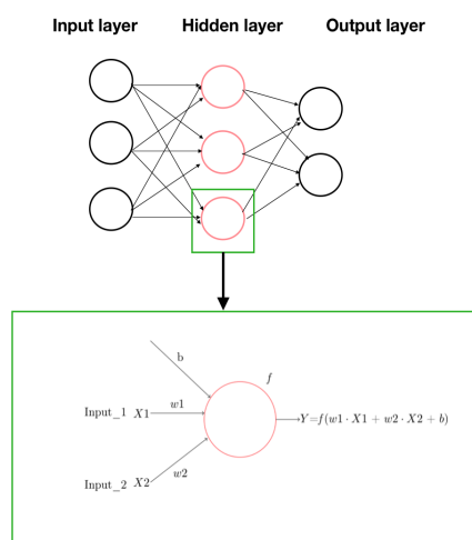
Figure 2.9: Structure of shallow Neural Network and its neuron
