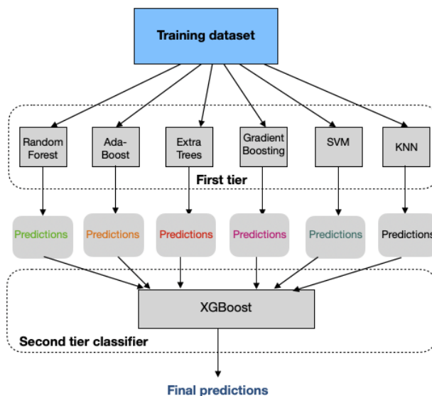
Figure 3.1: Flowchart for the proposed ensemble classifier in a two-tier architecture [99].
