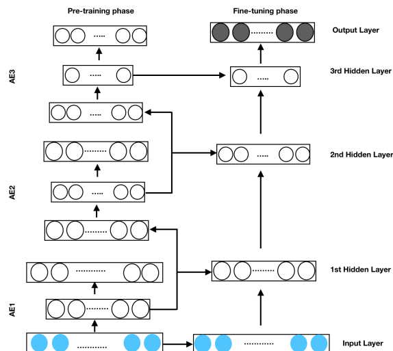
Figure 2.16: General Stacked AE process
