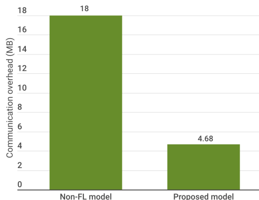
Figure 6.6: Comparison in terms of communication overhead.
