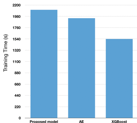
Figure 5.10: Training time comparison
