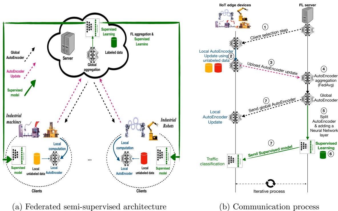
Figure 6.1: The network architecture and communication process of FLUIDS.
