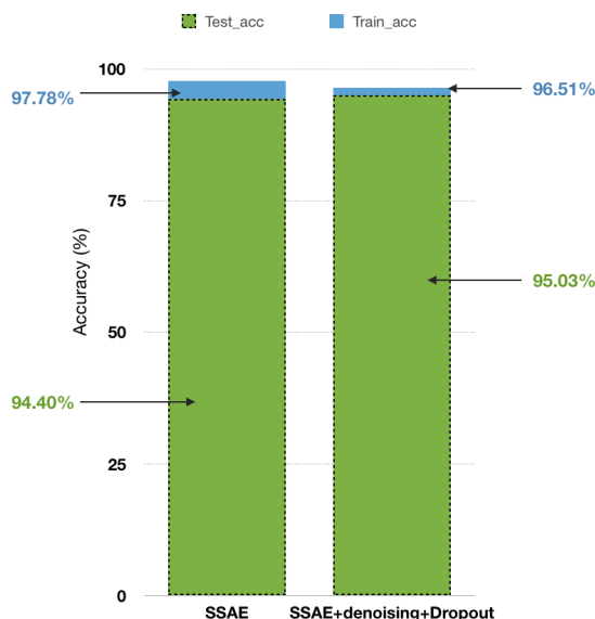
Figure 5.7: Accuracy of our model without and with enforcement (dropout and denoising)
