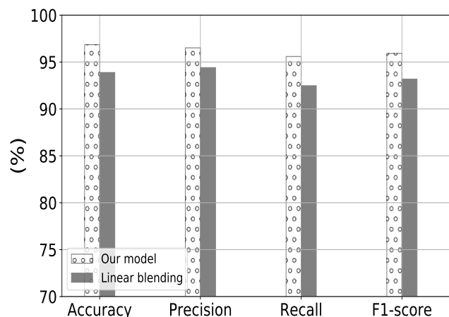
Figure 4.6: Our model vs. linear blending
