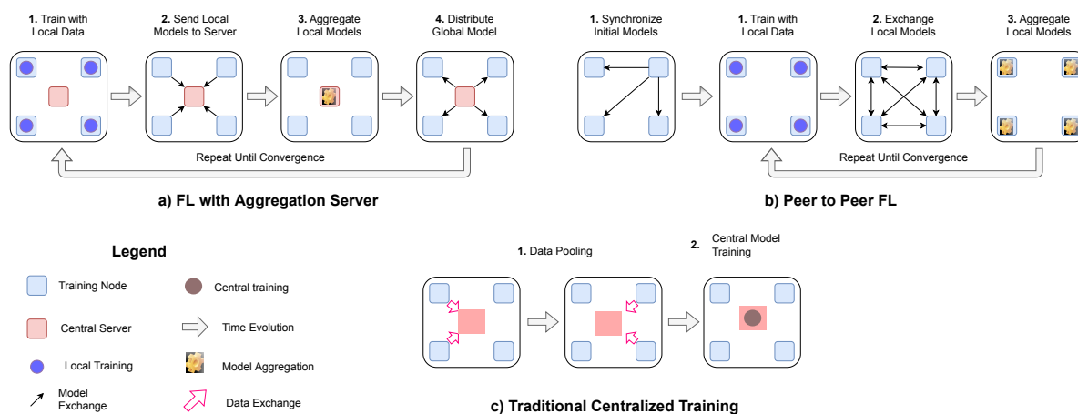
Figure 2.19: Typical FL workflows in comparison to traditional learning based on a centralized data manager. (a) Centralized FL and (b) Peer to Peer FL formulations allow private data to remain local to clients. (c) A general non-FL training workflow where the clients send their data to a central entity for model training.
