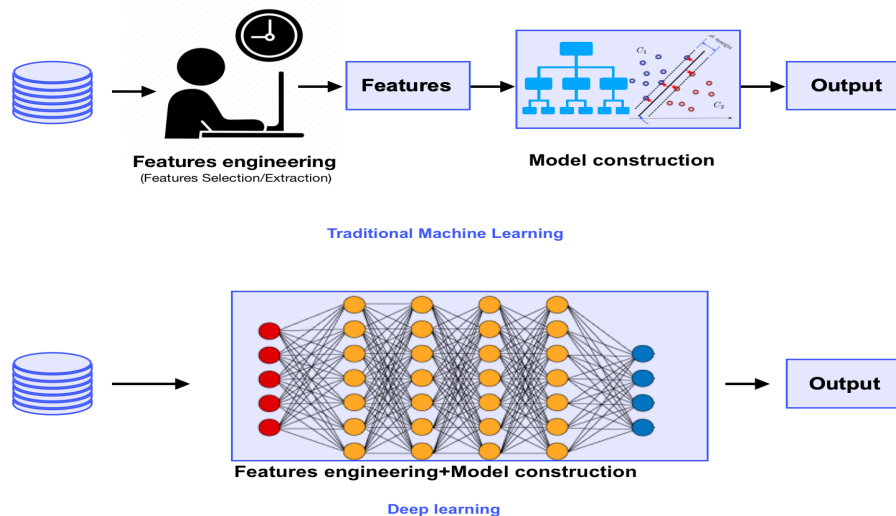
Figure 2.7: Difference between traditional Machine Learning and Deep Learning
