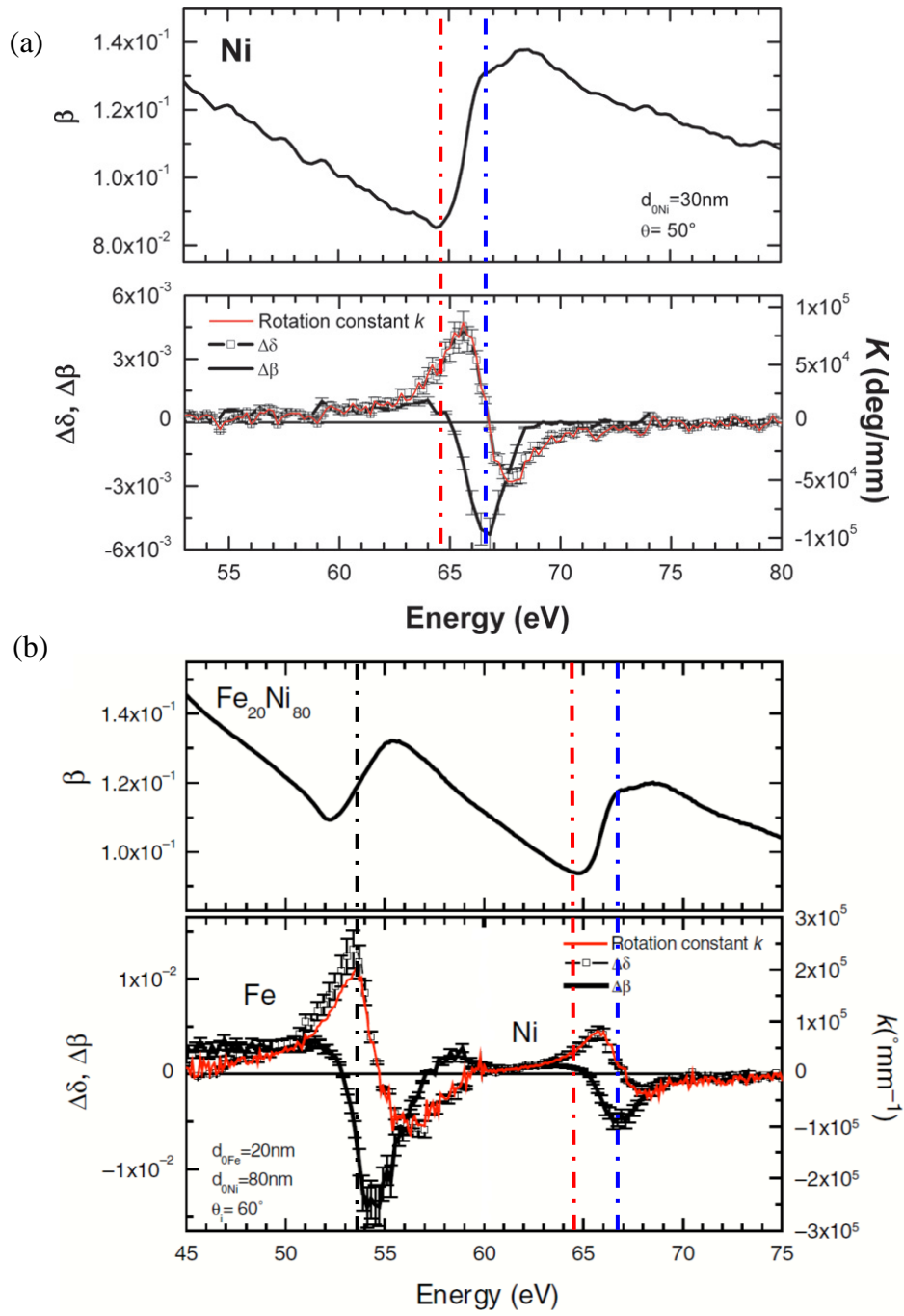
Figure 4.11: Magneto optical constant as function of photon energy for (a) Ni and (b) Py measured around the Ni and Fe M edges [93]. The red dash line is 64.7 eV and the blue dash line is 66.9 eV and the black dash is 53.7 eV. Pure Ni (a) and Py (b).
